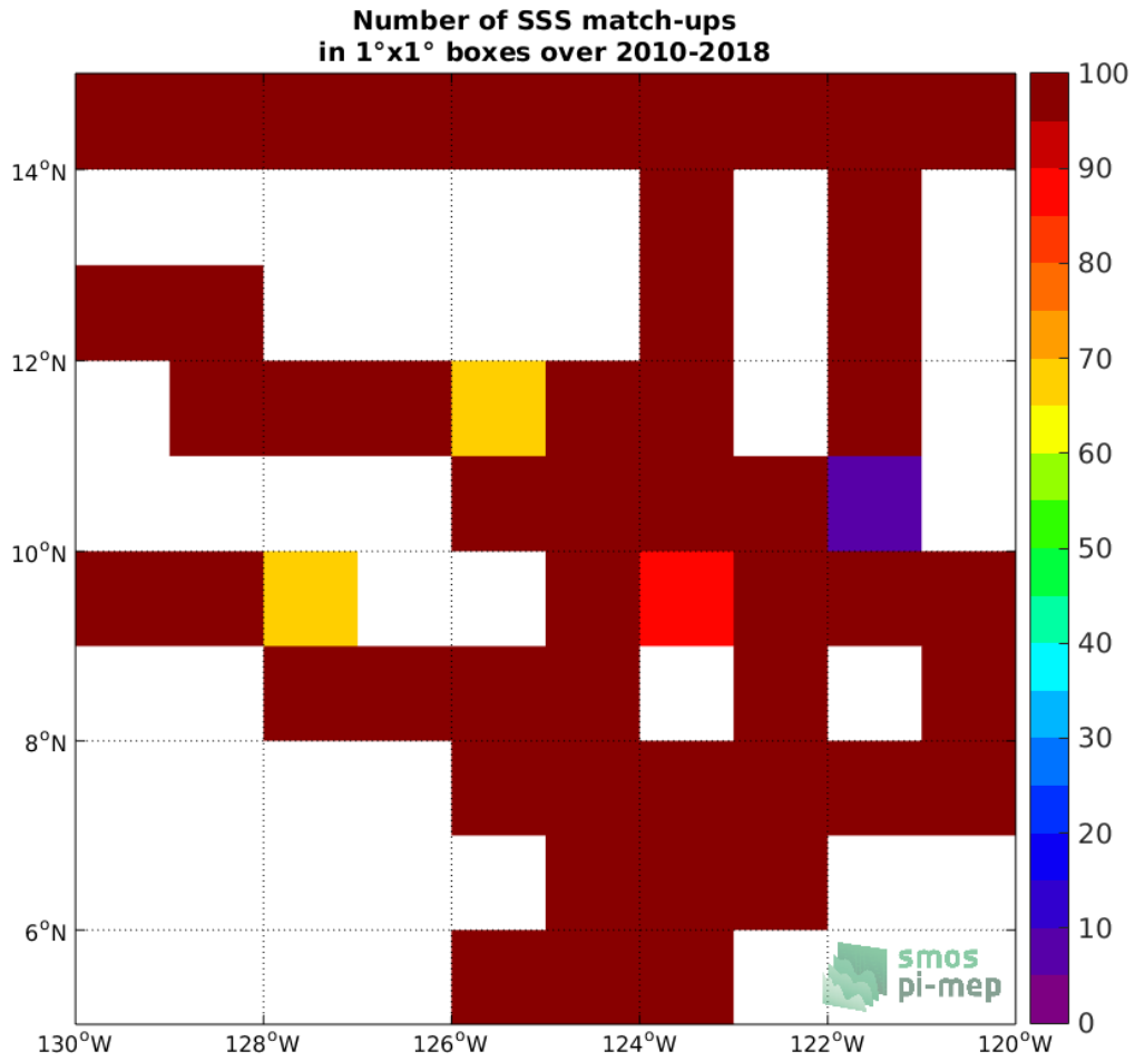
Figure 4: Number of SSS match-ups between TSG-SAMOS SSS and the SMOS-L3-CATDS-CPDC-V317-10DAYS-25KM SSS product for the SPURS 2 Pi-MEP region over 1°x1° boxes and for the full satellite product period.
