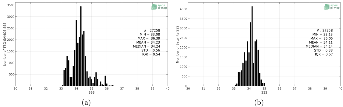
Figure 2: Histograms of SSS from TSG-SAMOS (a) and SMOS-L3-CATDS-CPDC-V317-10DAYS-25KM (b) considering all match-up pairs per bins of 0.1 over the SPURS 2 Pi-MEP region and for the full satellite product period.
