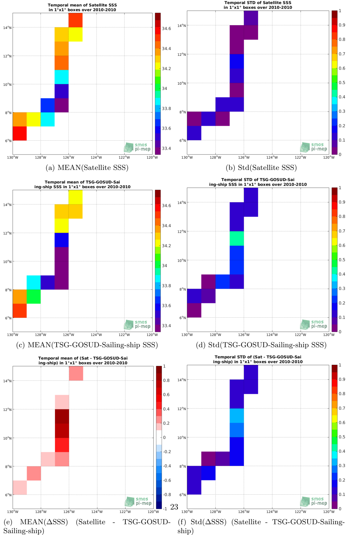
Figure 6: Temporal mean (left) and Std (right) of SSS from SMOS L3 v317 - 10 Days - 25 km (CATDS-CPDC) (top), TSG-GOSUD-Sailing-ship (middle), and of \Delta SSS (Satellite - TSG-GOSUD-Sailing-ship). Only match-up pairs are used to generate these maps.
