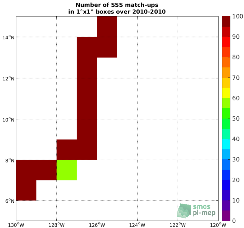
Figure 4: Number of SSS match-ups between TSG-GOSUD-Sailing-ship SSS and the SMOS L3 v317 - 10 Days - 25 km (CATDS-CPDC) SSS product for the SPURS 2 Pi-MEP region over 1°x1° boxes and for the full satellite product period.
