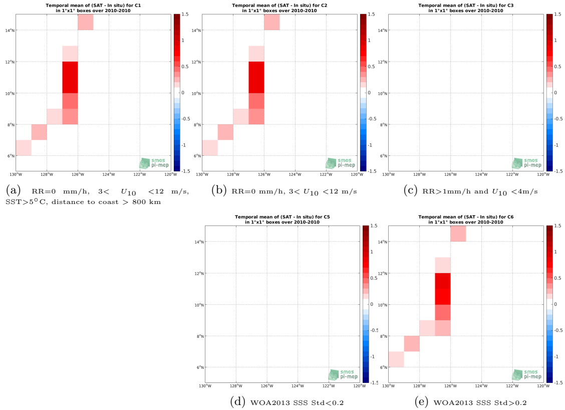
Figure 12: Temporal mean gridded over spatial boxes of size 1°x1° of \Delta SSS (SMOS L3 v317 - 10 Days - 25 km (CATDS-CPDC) - TSG-GOSUD-Sailing-ship) for 5 different subdatasets corresponding to: RR=0 mm/h, 3 < U_{10} < 12 m/s, SST > 5°C, distance to coast > 800 km (a), RR=0 mm/h, 3 < U_{10} < 12 m/s (b), RR > 1mm/h and U_{10} < 4 m/s (c), WOA2013 SSS Std < 0.2 (d), WOA2013 SSS Std > 0.2 (e).
