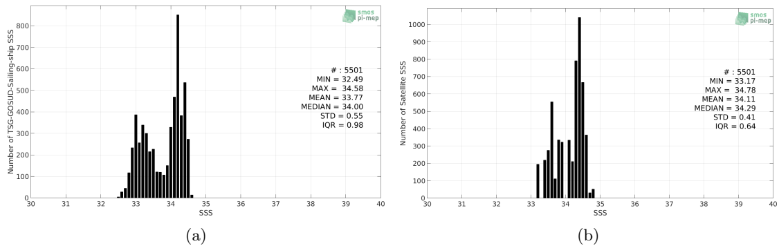
Figure 2: Histograms of SSS from TSG-GOSUD-Sailing-ship (a) and SMOS L3 v317 - 10 Days - 25 km (CATDS-CPDC) (b) considering all match-up pairs per bins of 0.1 over the SPURS 2 Pi-MEP region and for the full satellite product period.
