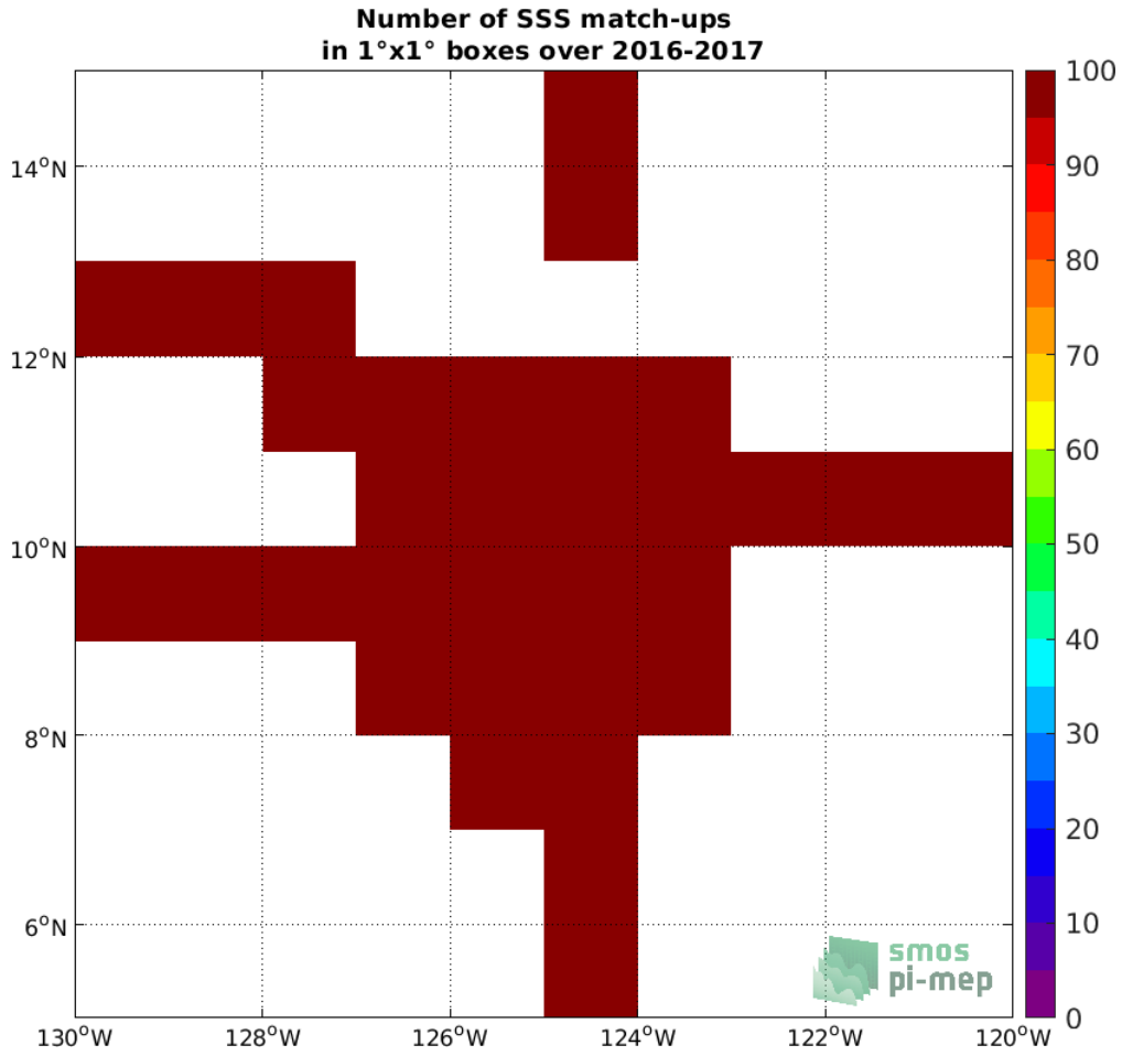
Figure 3: Number of SSS match-ups between Salinity Snake SSS and the SMOS SSS L3 v317 - 10 Days - 25 km (CATDS-CPDC) SSS product for the SPURS 2 Pi-MEP region over 1°x1° boxes and for the full satellite product period.
