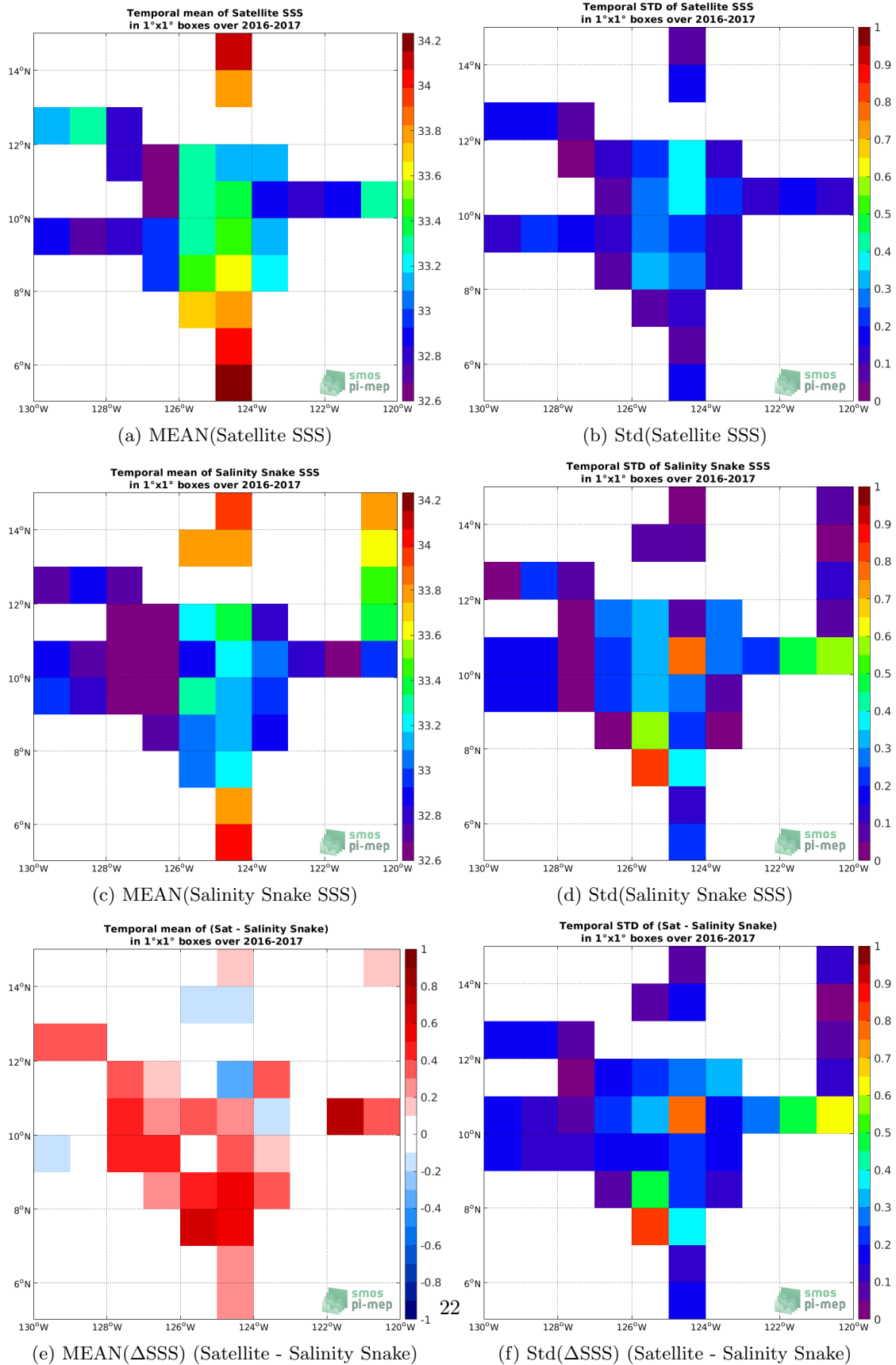
Figure 5: Temporal mean (left) and Std (right) of SSS from SMOS SSS L3 v317 - 10 Days - 25 km (CATDS-CPDC) (top), Salinity Snake (middle), and of \Delta SSS (Satellite - Salinity Snake). Only match-up pairs are used to generate these maps.
