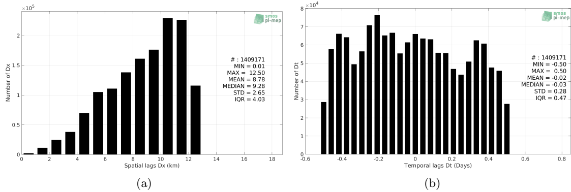
Figure 4: Histograms of the spatial (a) and temporal (b) lags between the location/time of the Salinity Snake measurement and the date of the corresponding SMOS SSS L3 v317 - 10 Days - 25 km (CATDS-CPDC) SSS pixel.
