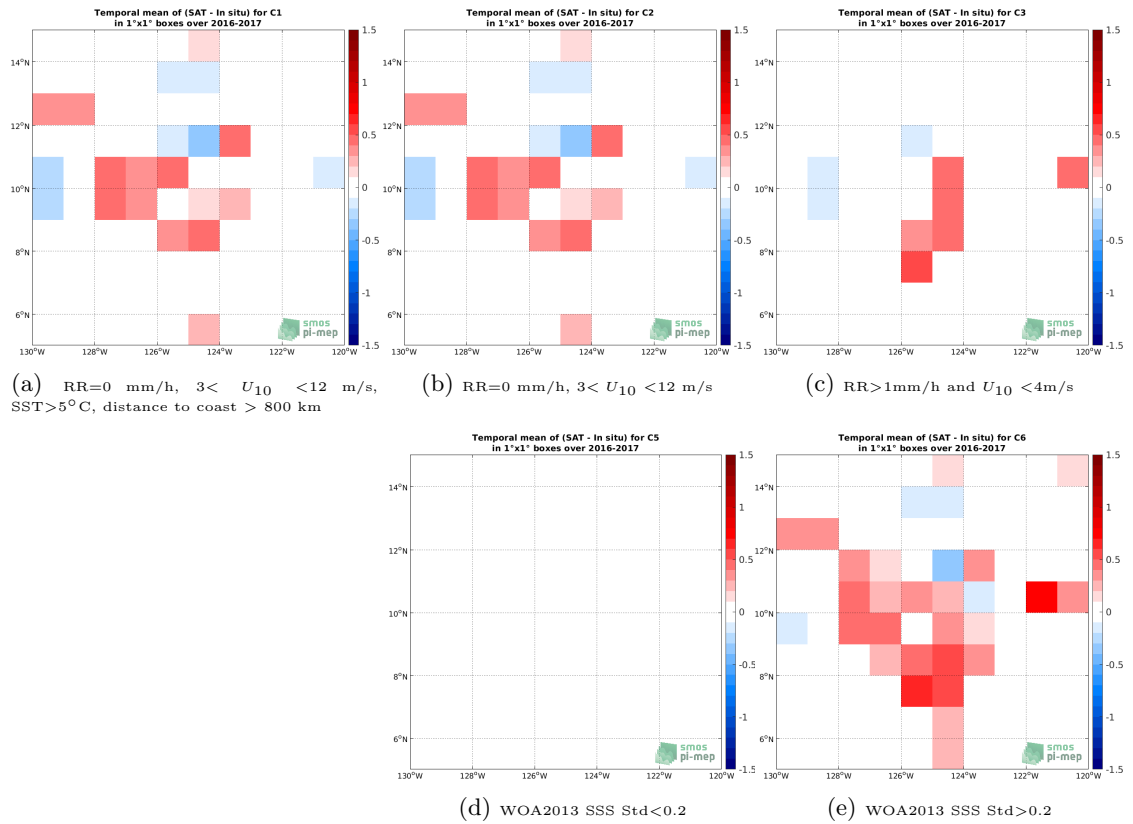
Figure 11: Temporal mean gridded over spatial boxes of size 1^\circ \times 1^\circ of \Delta SSS (SMOS SSS L3 v317 - 10 Days - 25 km (CATDS-CPDC) - Salinity Snake) for 5 different subdatasets corresponding to:RR=0 mm/h, 3 < U_{10} < 12 m/s, SST >5^\circ C, distance to coast > 800 km (a), RR=0 mm/h, 3 < U_{10} < 12 m/s (b), RR >1 mm/h and U_{10} < 4 m/s (c), WOA2013 SSS Std <0.2 (d), WOA2013 SSS Std >0.2 (e).
