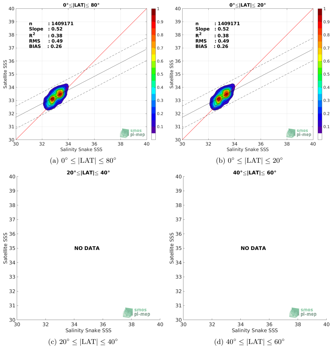
Figure 8: Contour maps of the concentration of SMOS SSS L3 v317 - 10 Days - 25 km (CATDS-CPDC) SSS (y-axis) versus Salinity Snake SSS (x-axis) at match-up pairs for different latitude bands. For each plot, the red line shows x=y . The black thin and dashed lines indicate a linear fit through the data cloud and the \pm 95\% confidence levels, respectively. The number match-up pairs n , the slope and R^2 coefficient of the linear fit, the root mean square (RMS) and the mean bias between satellite and in situ data are indicated for each latitude band in each plots.
