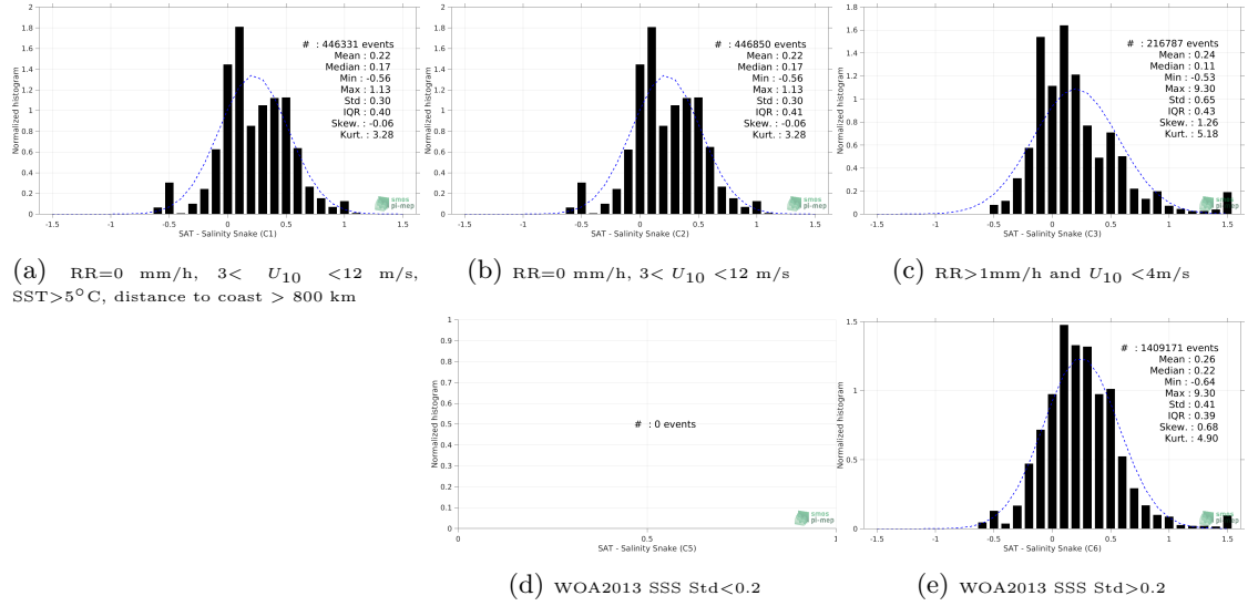
Figure 12: Normalized histogram of \Delta SSS (SMOS SSS L3 v317 - 10 Days - 25 km (CATDS-CPDC) - Salinity Snake) for 5 different subdatasets corresponding to: RR=0 mm/h, 3 < U_{10} < 12 m/s, SST > 5°C, distance to coast > 800 km (a), RR=0 mm/h, 3 < U_{10} < 12 m/s (b), RR > 1mm/h and U_{10} < 4 m/s (c), WOA2013 SSS Std < 0.2 (d), WOA2013 SSS Std > 0.2 (e).
