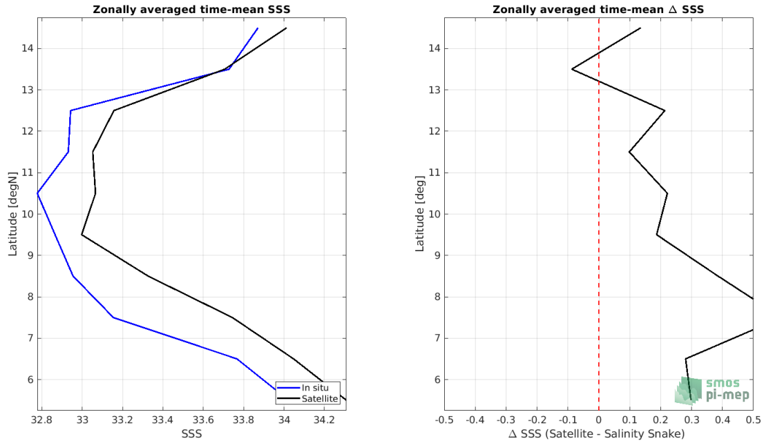
Figure 7: Left panel: Zonal mean SSS from SMOS SSS L3 v317 - 10 Days - 25 km (CATDS-CPDC) satellite product (black) and from Salinity Snake (blue). Right panel: Zonal mean of \Delta SSS (Satellite - Salinity Snake) for all the collected Pi-MEP match-up pairs estimated over the full satellite product period.
