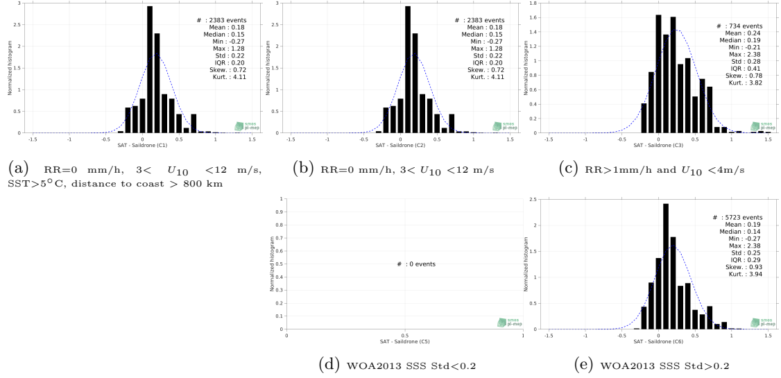
Figure 12: Normalized histogram of \Delta SSS (SMOS SSS L3 v317 - 10 Days - 25 km (CATDS-CPDC) - Sairdrone) for 5 different subdatasets corresponding to: RR=0 mm/h, 3 < U_{10} < 12 m/s, SST > 5°C, distance to coast > 800 km (a), RR=0 mm/h, 3 < U_{10} < 12 m/s (b), RR > 1mm/h and U_{10} < 4 m/s (c), WOA2013 SSS Std < 0.2 (d), WOA2013 SSS Std > 0.2 (e).
