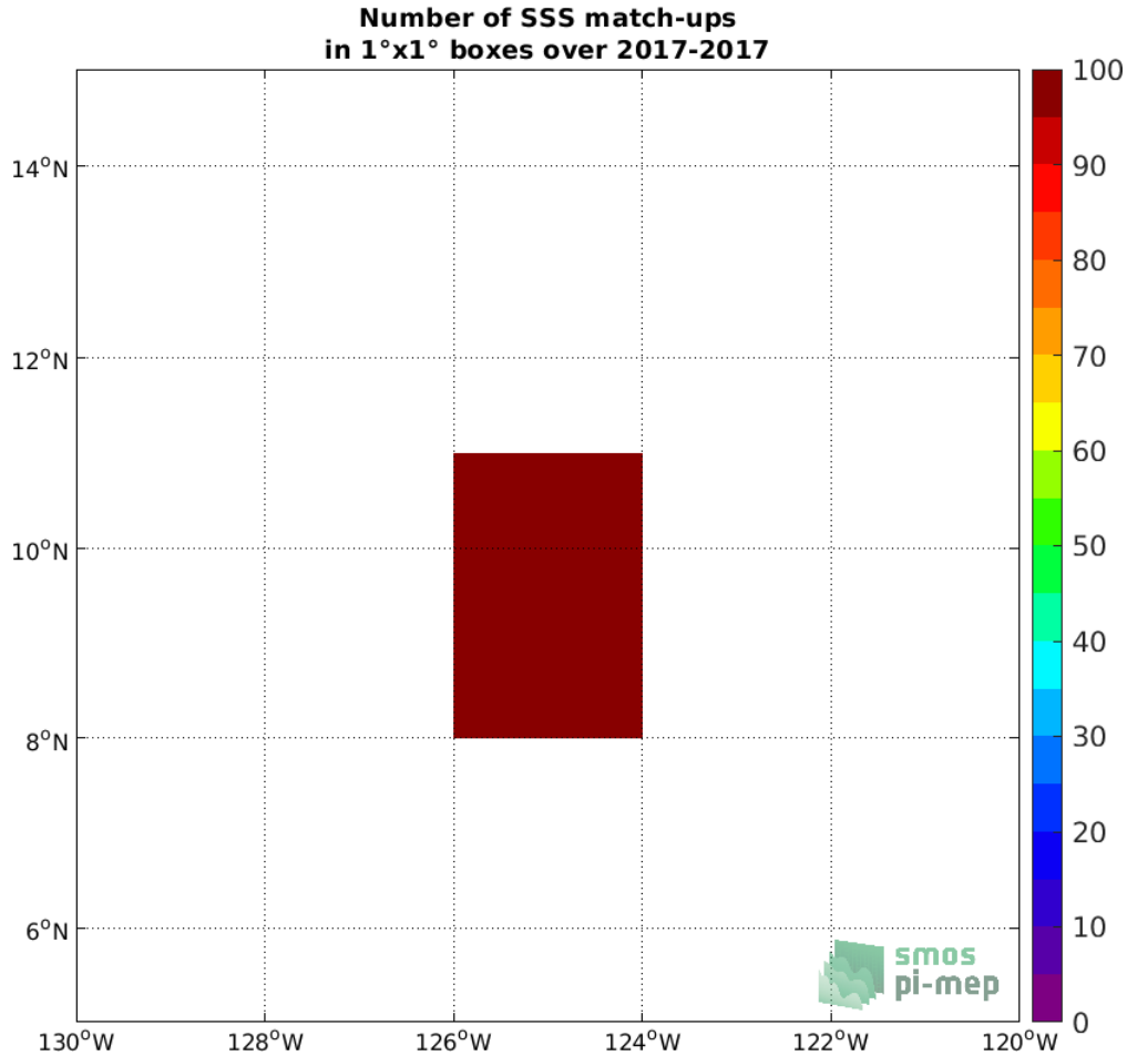
Figure 3: Number of SSS match-ups between Saildrone SSS and the SMOS SSS L3 v317 - 10 Days - 25 km (CATDS-CPDC) SSS product for the SPURS 2 Pi-MEP region over 1^\circ \times 1^\circ boxes and for the full satellite product period.
