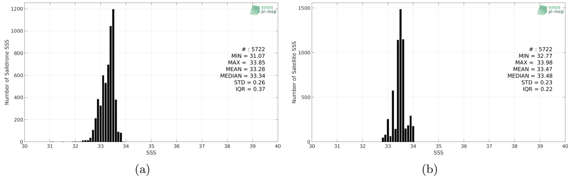
Figure 2: Histograms of SSS from Saildrone (a) and SMOS SSS L3 v317 - 10 Days - 25 km (CATDS-CPDC) (b) considering all match-up pairs per bins of 0.1 over the SPURS 2 Pi-MEP region and for the full satellite product period.
