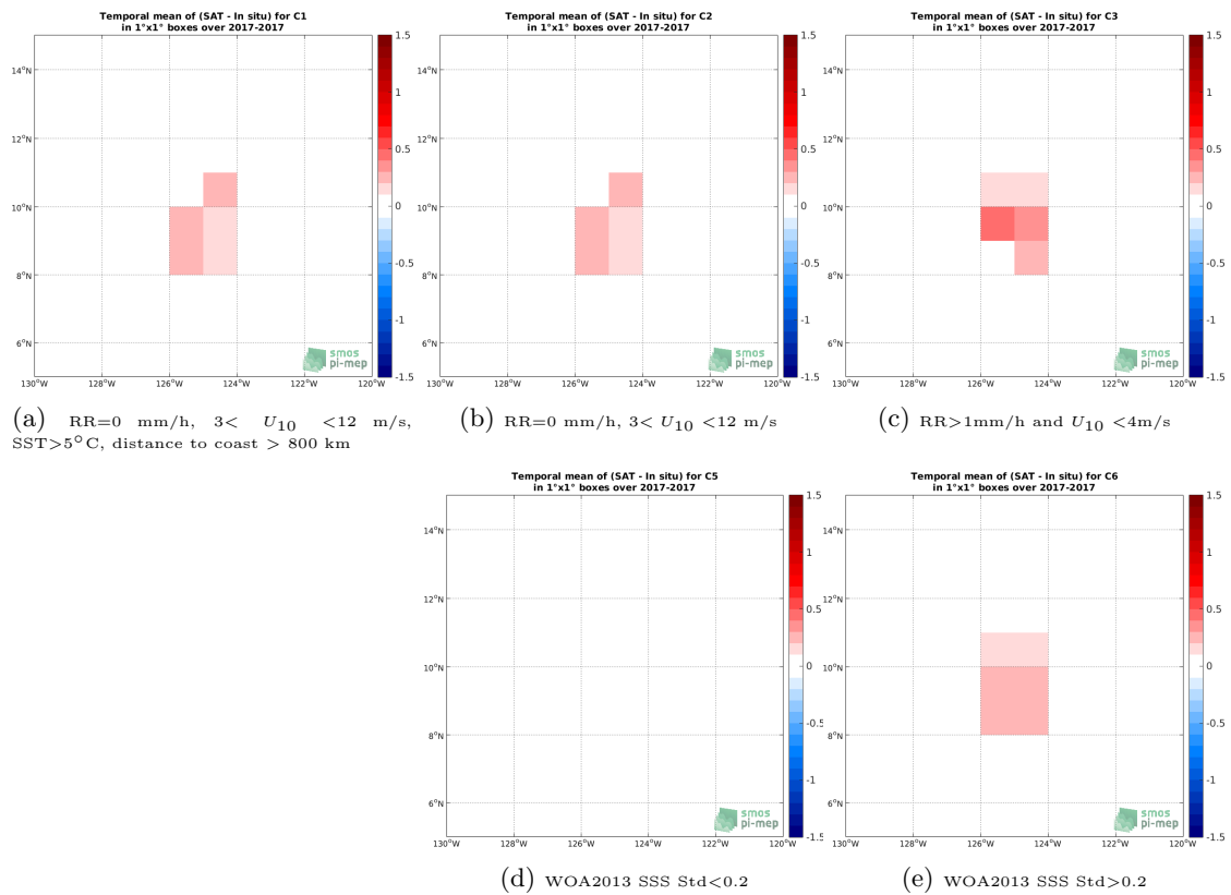
Figure 12: Temporal mean gridded over spatial boxes of size 1^\circ \times 1^\circ of \Delta SSS (SMOS SSS L3 v317 - 10 Days - 25 km (CATDS-CPDC) - Saifdrone) for 5 different subdatasets corresponding to:RR=0 mm/h, 3 < U_{10} < 12 m/s, SST >5^\circ\text{C} , distance to coast > 800 km (a), RR=0 mm/h, 3 < U_{10} < 12 m/s (b), RR >1 mm/h and U_{10} < 4 m/s (c), WOA2013 SSS Std <0.2 (d), WOA2013 SSS Std >0.2 (e).
