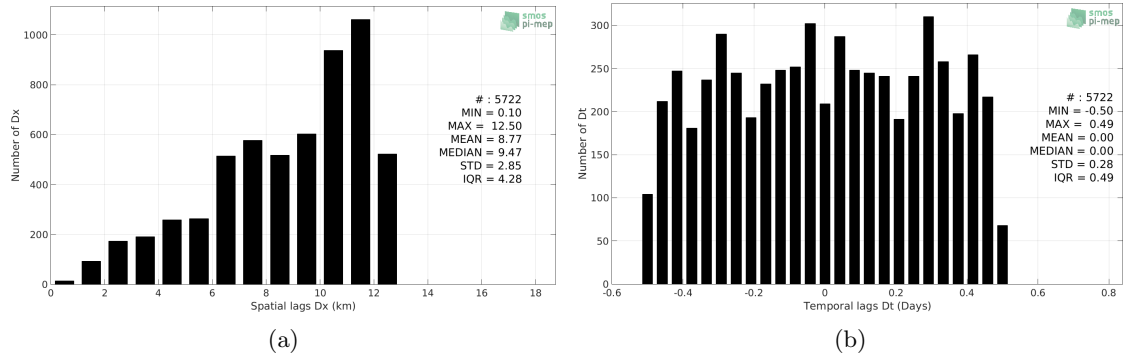
Figure 5: Histograms of the spatial (a) and temporal (b) lags between the time of the Saildrone measurements and the date of the corresponding SMOS SSS L3 v317 - 10 Days - 25 km (CATDS-CPDC) SSS product.
