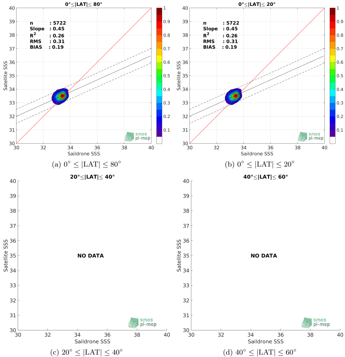
Figure 9: Contour maps of the concentration of SMOS SSS L3 v317 - 10 Days - 25 km (CATDS-CPDC) SSS (y-axis) versus SAILDRONE SSS (x-axis) at match-up pairs for different latitude bands. For each plot, the red line shows x=y . The black thin and dashed lines indicate a linear fit through the data cloud and the \pm 95\% confidence levels, respectively. The number match-up pairs n , the slope and R^2 coefficient of the linear fit, the root mean square (RMS) and the mean bias between satellite and in situ data are indicated for each latitude band in each plots.
