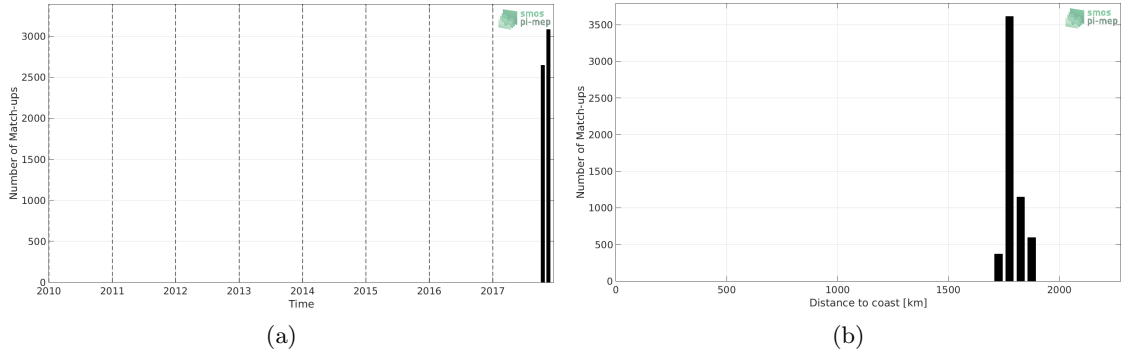
Figure 1: Number of match-ups between Saildrone and SMOS SSS L3 v317 - 10 Days - 25 km (CATDS-CPDC) SSS as a function of time (a) and as function of the distance to coast (b) over the SPURS 2 Pi-MEP region and for the full satellite product period.
