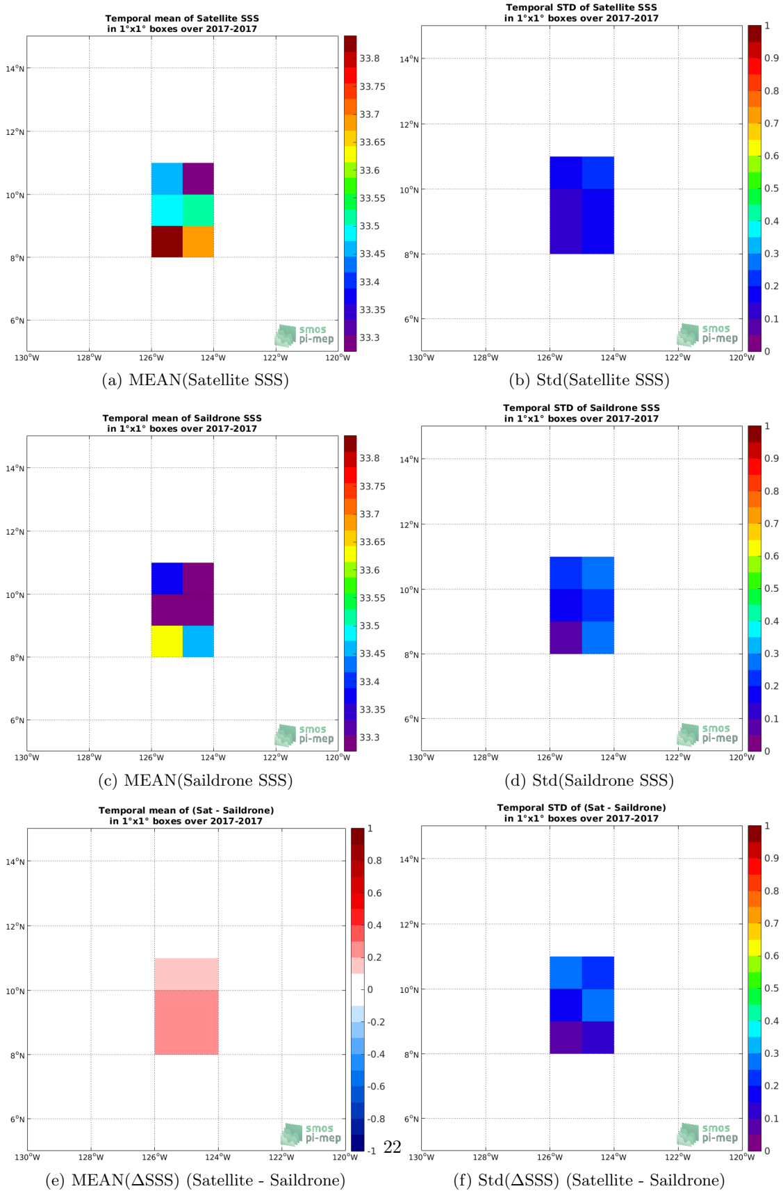
Figure 6: Temporal mean (left) and Std (right) of SSS from SMOS SSS L3 v317 - 10 Days - 25 km (CATDS-CPDC) (top), Saildrone (middle), and of \Delta SSS (Satellite - Saildrone). Only match-up pairs are used to generate these maps.
