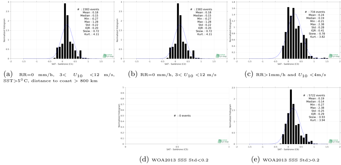
Figure 13: Normalized histogram of \Delta SSS (SMOS SSS L3 v317 - 10 Days - 25 km (CATDS-CPDC) - Saildrone) for 5 different subdatasets corresponding to: RR=0 mm/h, 3 < U_{10} < 12 m/s, SST > 5°C, distance to coast > 800 km (a), RR=0 mm/h, 3 < U_{10} < 12 m/s (b), RR > 1mm/h and U_{10} < 4 m/s (c), WOA2013 SSS Std < 0.2 (d), WOA2013 SSS Std > 0.2 (e).
