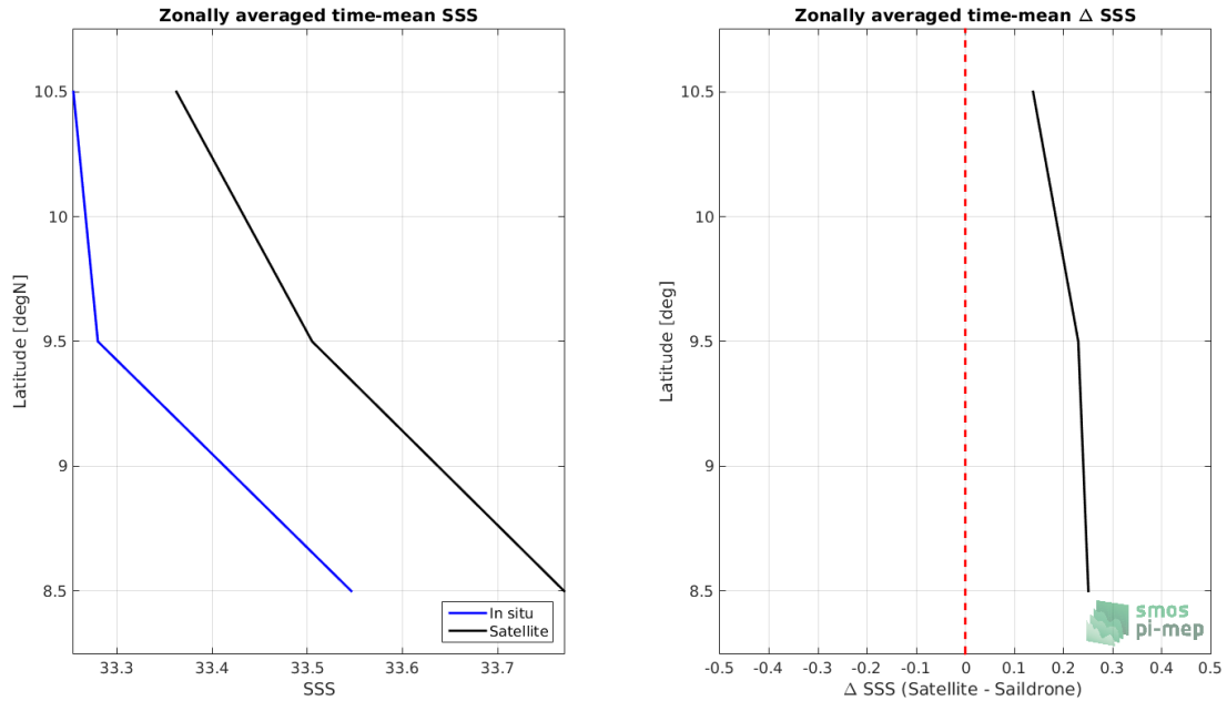
Figure 8: Left panel: Zonal mean SSS from SMOS SSS L3 v317 - 10 Days - 25 km (CATDS-CPDC) satellite product (black) and from Sairdrone (blue). Right panel: Zonal mean of \Delta SSS (Satellite - Sairdrone) for all the collected Pi-MEP match-up pairs estimated over the full satellite product period.
