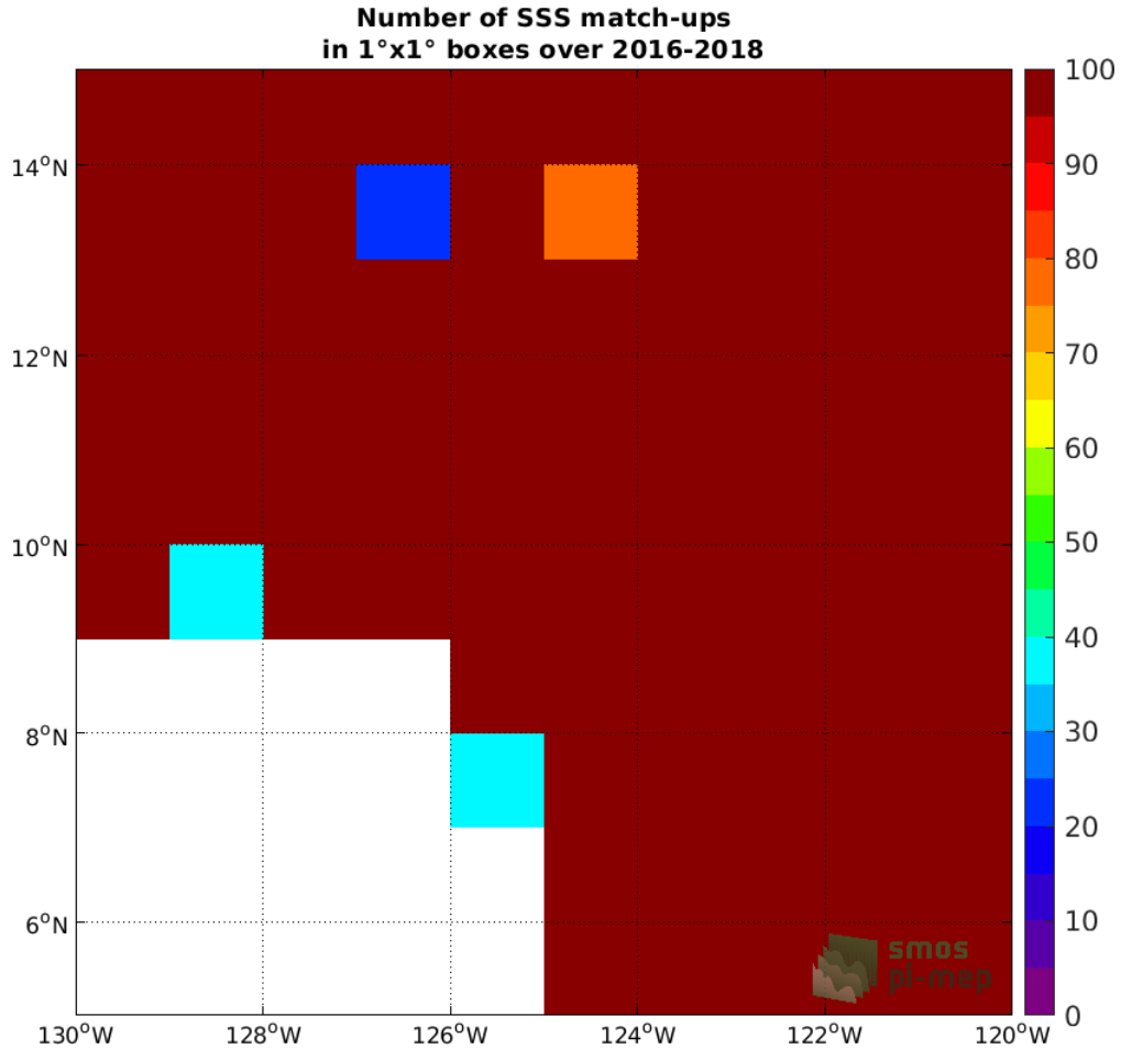
Figure 3: Number of SSS match-ups between Surface drifters SSS and the SMOS SSS L3 v317 - 10 Days - 25 km (CATDS-CPDC) SSS product for the SPURS 2 Pi-MEP region over 1^\circ \times 1^\circ boxes and for the full satellite product period.
