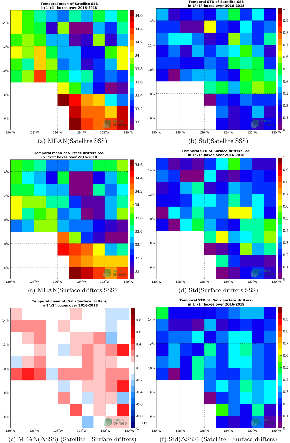
Figure 5: Temporal mean (left) and Std (right) of SSS from SMOS SSS L3 v317 - 10 Days - 25 km (CATDS-CPDC) (top), Surface drifters (middle), and of \Delta SSS (Satellite - Surface drifters). Only match-up pairs are used to generate these maps.
