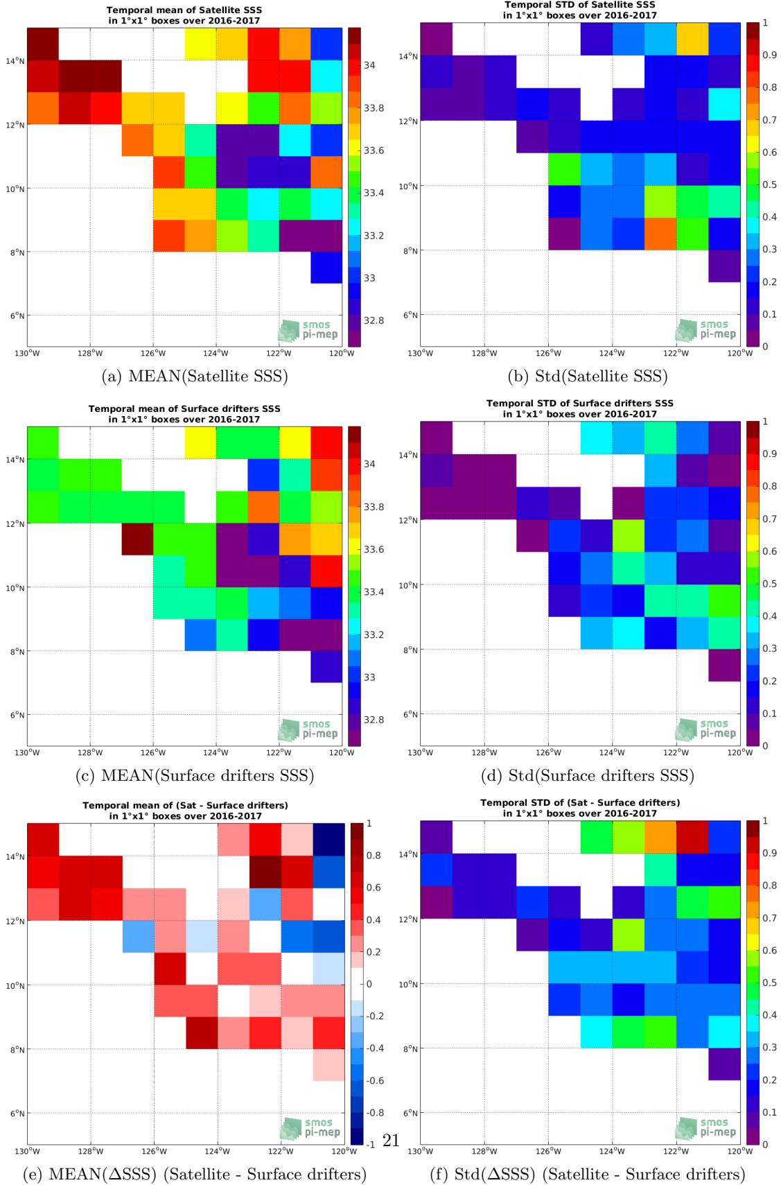
Figure 5: Temporal mean (left) and Std (right) of SSS from SMOS-L3-CATDS-CPDC-V317-10DAYS-25KM (top), Surface drifters (middle), and of \Delta SSS (Satellite - Surface drifters). Only match-up pairs are used to generate these maps.
