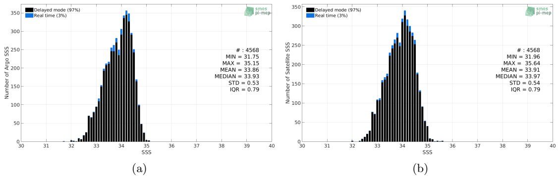
Figure 2: Histograms of SSS from Argo (a) and SMOS SSS L3 v317 - 10 Days - 25 km (CATDS-CPDC) (b) considering all match-up pairs per bins of 0.1 over the SPURS 2 Pi-MEP region and for the full satellite product period.
