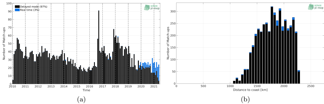
Figure 1: Number of match-ups between Argo and SMOS SSS L3 v317 - 10 Days - 25 km (CATDS-CPDC) SSS as a function of time (a) and as function of the distance to coast (b) over the SPURS 2 Pi-MEP region and for the full satellite product period.
