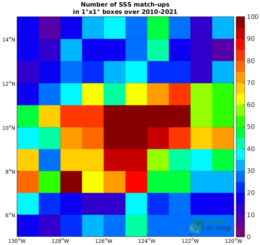
Figure 4: Number of SSS match-ups between Argo SSS and the SMOS SSS L3 v317 - 10 Days - 25 km (CATDS-CPDC) SSS product for the SPURS 2 Pi-MEP region over 1°×1° boxes and for the full satellite product period.
