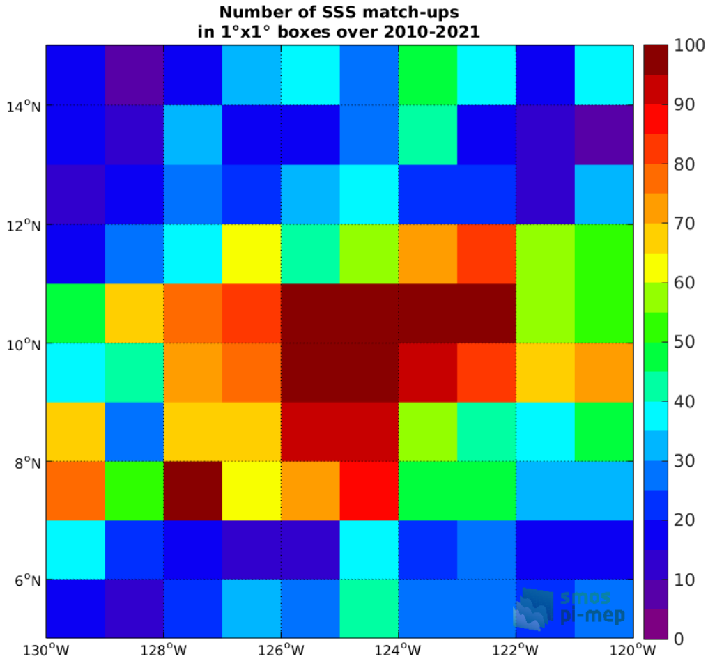
Figure 4: Number of SSS match-ups between Argo SSS and the SMOS SSS L3 v317 - 10 Days - 25 km (CATDS-CPDC) SSS product for the SPURS 2 Pi-MEP region over 1°x1° boxes and for the full satellite product period.
