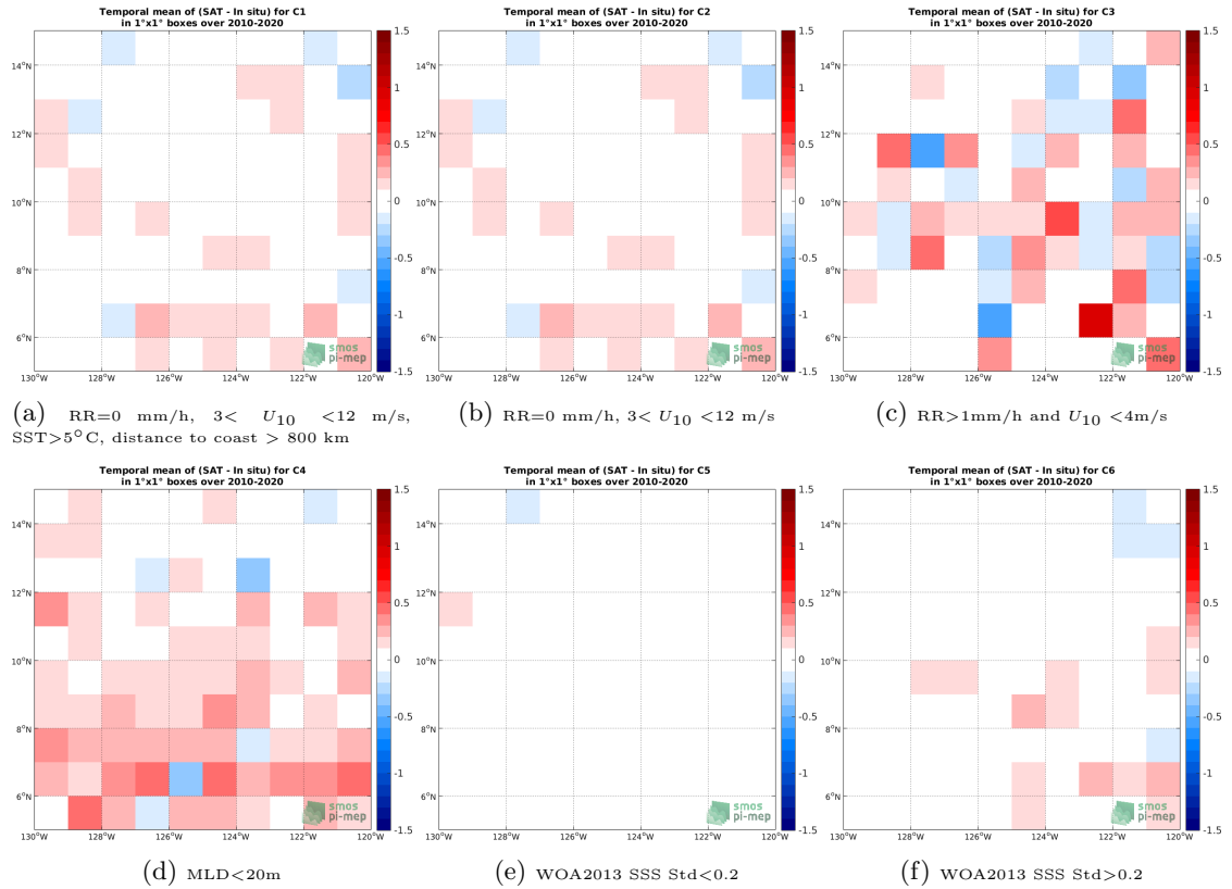
Figure 12: Temporal mean gridded over spatial boxes of size 1^\circ \times 1^\circ of \Delta SSS (SMOS SSS L3 v317 - 10 Days - 25 km (CATDS-CPDC) - Argo) for 6 different subdatasets corresponding to:RR=0 mm/h, 3 < U_{10} < 12 m/s, SST >5^\circ C, distance to coast > 800 km (a), RR=0 mm/h, 3 < U_{10} < 12 m/s (b), RR >1 mm/h and U_{10} < 4 m/s (c),MLD <20 m (d),WOA2013 SSS Std <0.2 (e),WOA2013 SSS Std >0.2 (f).
