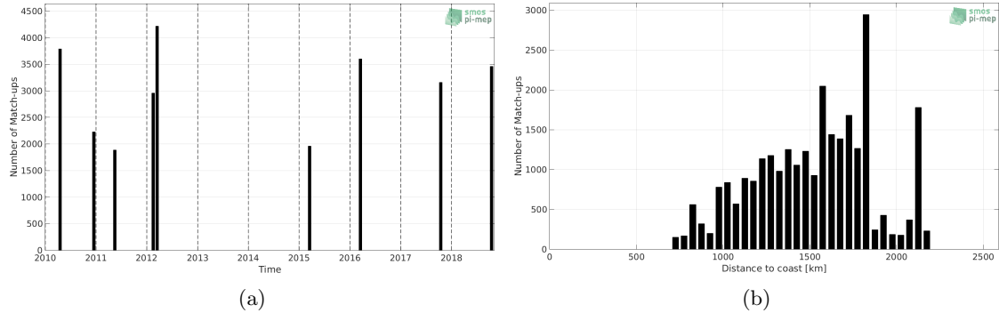
Figure 1: Number of match-ups between TSG-SAMOS and SMOS-L3-CATDS-CPDC-V3-MONTHLY-25KM SSS as a function of time (a) and as function of the distance to coast (b) over the SPURS 2 Pi-MEP region and for the full satellite product period.
