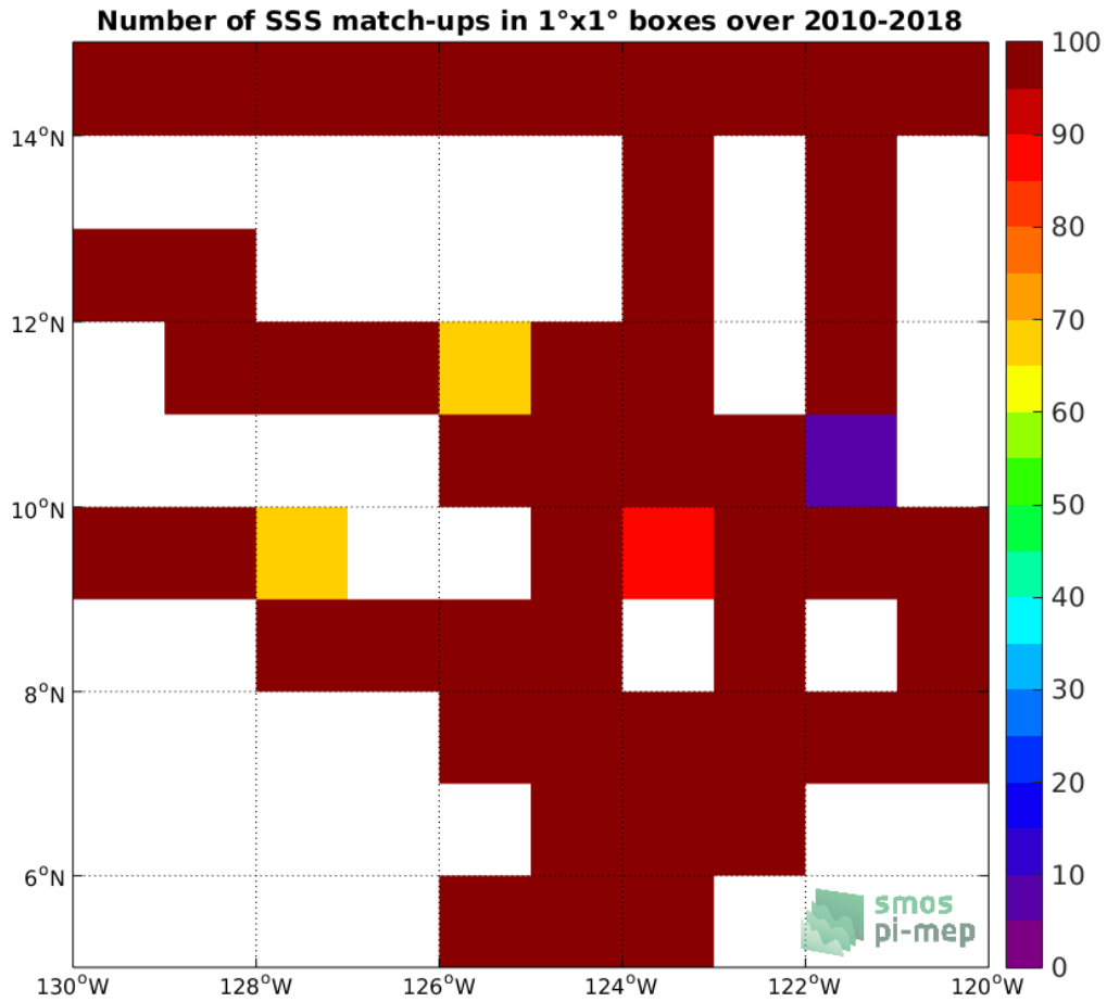
Figure 4: Number of SSS match-ups between TSG-SAMOS SSS and the SMOS-L3-CATDS-CPDC-V3-MONTHLY-25KM SSS product for the SPURS 2 Pi-MEP region over 1°x1° boxes and for the full satellite product period.
