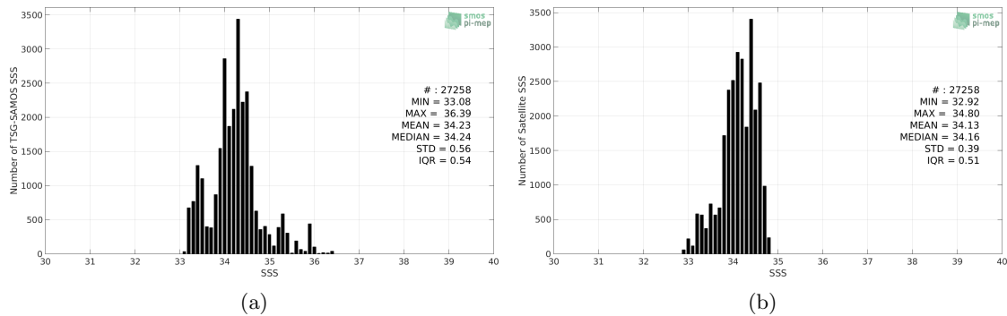
Figure 2: Histograms of SSS from TSG-SAMOS (a) and SMOS-L3-CATDS-CPDC-V3-MONTHLY-25KM (b) considering all match-up pairs per bins of 0.1 over the SPURS 2 Pi-MEP region and for the full satellite product period.
