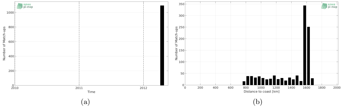
Figure 1: Number of match-ups between TSG-GOSUD-Research-vessel and SMOS-L3-CATDS-CPDC-V3-MONTHLY-25KM SSS as a function of time (a) and as function of the distance to coast (b) over the SPURS 2 Pi-MEP region and for the full satellite product period.
