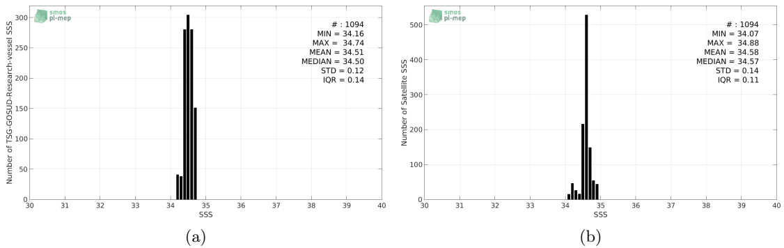
Figure 2: Histograms of SSS from TSG-GOSUD-Research-vessel (a) and SMOS-L3-CATDS-CPDC-V3-MONTHLY-25KM (b) considering all match-up pairs per bins of 0.1 over the SPURS 2 Pi-MEP region and for the full satellite product period.
