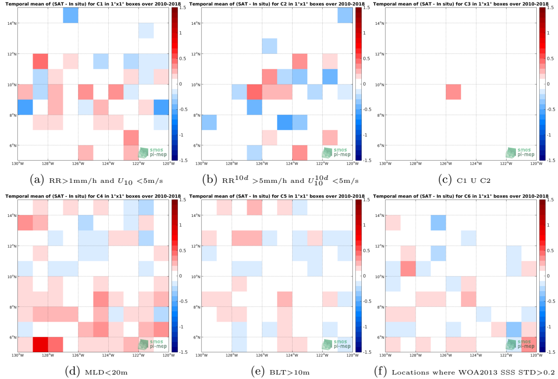
Figure 12: Temporal mean gridded over spatial boxes of size 1^\circ \times 1^\circ of \Delta\text{SSS} (SMOS-L3-CATDS-CPDC-V3-MONTHLY-25KM - Argo) for 6 different subdatasets corresponding to: \text{RR} > 1\text{mm/h} and U_{10} < 5\text{m/s} (a), \text{RR}^{10d} > 5\text{mm/h} and U_{10}^{10d} < 5\text{m/s} (b), C1 U C2 (c), \text{MLD} < 20\text{m} (d), \text{BLT} > 10\text{m} (e), Locations where WOA2013 SSS STD > 0.2 (f).
