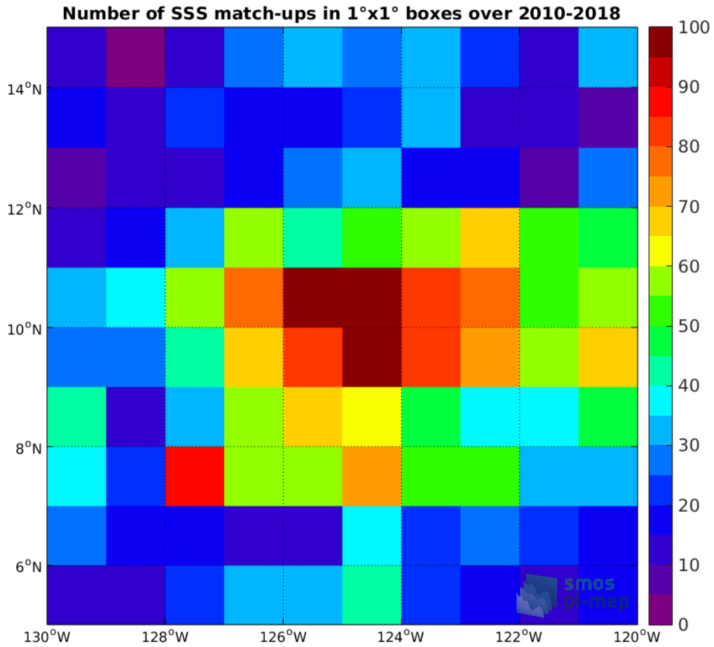
Figure 4: Number of SSS match-ups between Argo SSS and the SMOS-L3-CATDS-CPDC-V3-MONTHLY-25KM SSS product for the SPURS 2 Pi-MEP region over 1°x1° boxes and for the full satellite product period.
