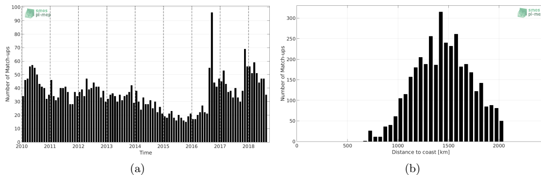
Figure 1: Number of match-ups between Argo and SMOS-L3-CATDS-CPDC-V3-MONTHLY-25KM SSS as a function of time (a) and as function of the distance to coast (b) over the SPURS 2 Pi-MEP region and for the full satellite product period.
