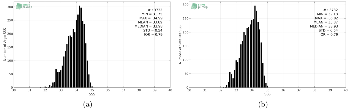
Figure 2: Histograms of SSS from Argo (a) and SMOS-L3-CATDS-CPDC-V3-MONTHLY-25KM (b) considering all match-up pairs per bins of 0.1 over the SPURS 2 Pi-MEP region and for the full satellite product period.
