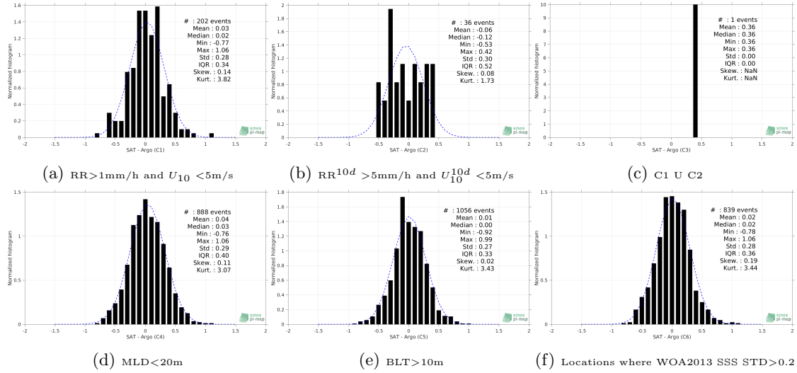
Figure 13: Normalized histogram of \Delta SSS (SMOS-L3-CATDS-CPDC-V3-MONTHLY-25KM - Argo) for 6 different subdatasets corresponding to: RR>1mm/h and U_{10} < 5\text{m/s} (a), RR^{10d} > 5\text{mm/h} and U_{10}^{10d} < 5\text{m/s} (b), C1 U C2 (c),MLD<20m (d),BLT>10m (e),Locations where WOA2013 SSS STD>0.2 (f).
