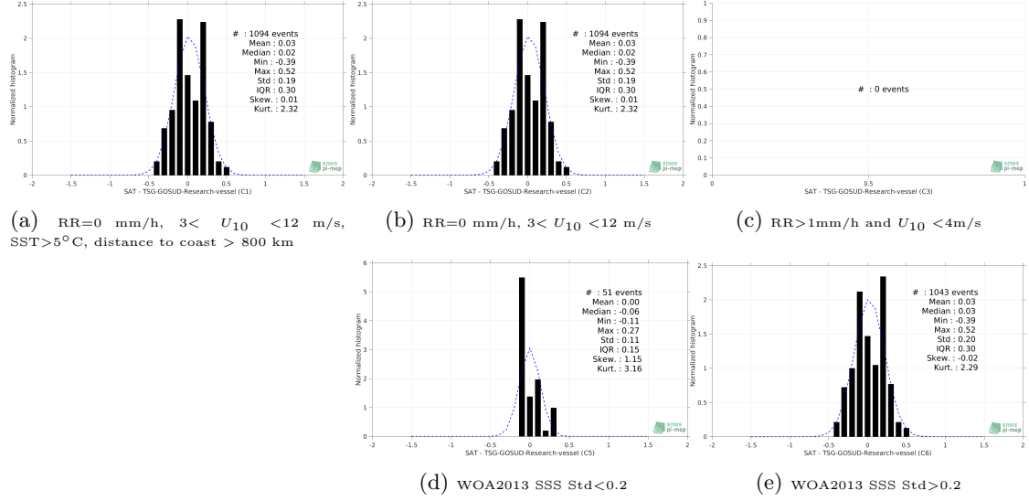
Figure 13: Normalized histogram of \Delta SSS (SMOS-L3-CATDS-CPDC-V3-10DAYS-25KM - TSG-GOSUD-Research-vessel) for 5 different subdatasets corresponding to: RR=0 mm/h, 3 < U_{10} < 12 m/s, SST>5°C, distance to coast > 800 km (a), RR=0 mm/h, 3 < U_{10} < 12 m/s (b), RR>1mm/h and U_{10} < 4 m/s (c), WOA2013 SSS Std<0.2 (d), WOA2013 SSS Std>0.2 (e).
