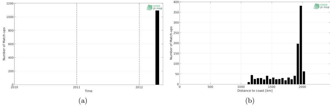
Figure 1: Number of match-ups between TSG-GOSUD-Research-vessel and SMOS-L3-CATDS-CPDC-V3-10DAYS-25KM SSS as a function of time (a) and as function of the distance to coast (b) over the SPURS 2 Pi-MEP region and for the full satellite product period.
