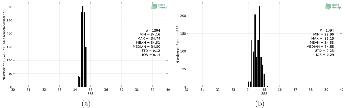
Figure 2: Histograms of SSS from TSG-GOSUD-Research-vessel (a) and SMOS-L3-CATDS-CPDC-V3-10DAYS-25KM (b) considering all match-up pairs per bins of 0.1 over the SPURS 2 Pi-MEP region and for the full satellite product period.
