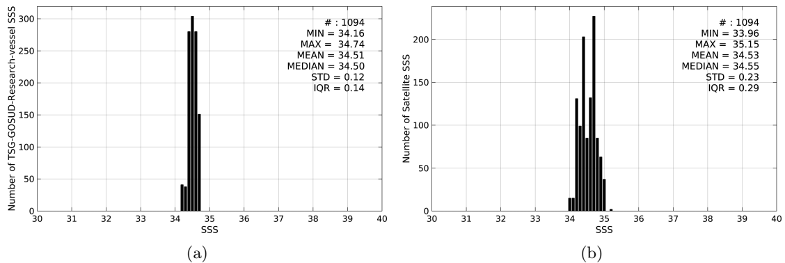
Figure 2: Histograms of SSS from TSG-GOSUD-Research-vessel (a) and SMOS-L3-CATDS-CPDC-V3-10DAYS-25KM (b) considering all match-up pairs per bins of 0.1 over the SPURS 2 Pi-MEP region and for the full satellite product period.
