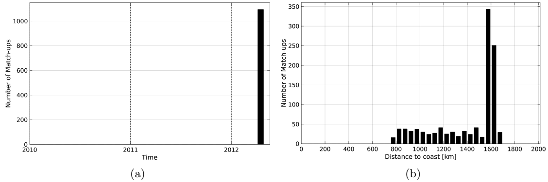
Figure 1: Number of match-ups between TSG-GOSUD-Research-vessel and SMOS-L3-CATDS-CPDC-V3-10DAYS-25KM SSS as a function of time (a) and as function of the distance to coast (b) over the SPURS 2 Pi-MEP region and for the full satellite product period.
