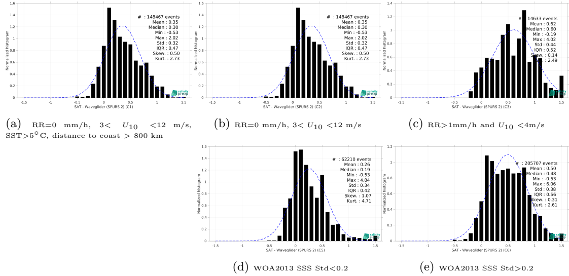
Figure 13: Normalized histogram of \Delta SSS (SMOS SSS L3 v2 - 9-Days (BEC) - Waveglider (SPURS 2)) for 5 different subdatasets corresponding to: RR=0 mm/h, 3 < U_{10} < 12 m/s, SST > 5°C, distance to coast > 800 km (a), RR=0 mm/h, 3 < U_{10} < 12 m/s (b), RR > 1mm/h and U_{10} < 4 m/s (c), WOA2013 SSS Std < 0.2 (d), WOA2013 SSS Std > 0.2 (e).
