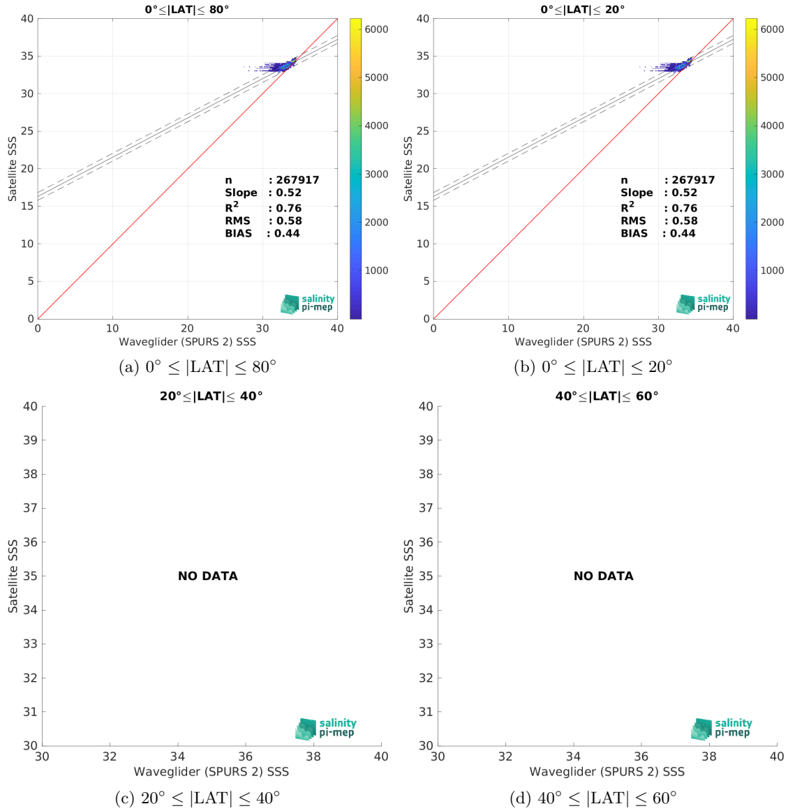
Figure 9: Contour maps of the concentration of SMOS SSS L3 v2 - 9-Days (BEC) SSS (y-axis) versus Waveglider (SPURS 2) SSS (x-axis) at match-up pairs for different latitude bands. For each plot, the red line shows x=y . The black thin and dashed lines indicate a linear fit through the data cloud and the \pm 95\% confidence levels, respectively. The number match-up pairs n , the slope and R^2 coefficient of the linear fit, the root mean square (RMS) and the mean bias between satellite and in situ data are indicated for each latitude band in each plots.
