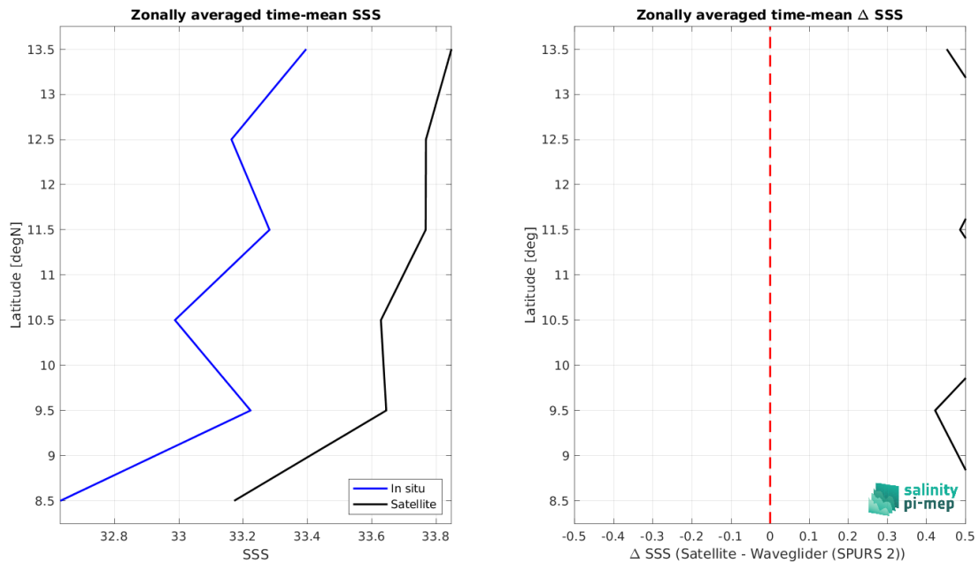
Figure 8: Left panel: Zonal mean SSS from SMOS SSS L3 v2 - 9-Days (BEC) satellite product (black) and from Waveglider (SPURS 2) (blue). Right panel: Zonal mean of \Delta SSS (Satellite - Waveglider (SPURS 2)) for all the collected Pi-MEP match-up pairs estimated over the full satellite product period.
