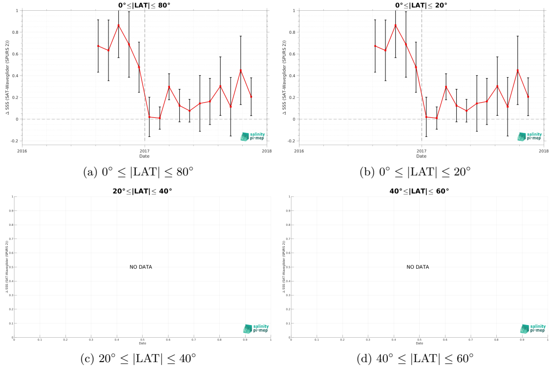
Figure 10: Monthly median (red curves) of \Delta\text{SSS} (Satellite - Waveglider (SPURS 2)) and \pm 1 Std (black vertical thick bars) as function of time for all the collected Pi-MEP match-up pairs estimated over the SPURS 2 Pi-MEP region and for the full satellite product period are shown for different latitude bands: (a) 80°S-80°N, (b) 20°S-20°N, (c) 40°S-20°S and 20°N-40°N and (d) 60°S-40°S and 40°N-60°N.
