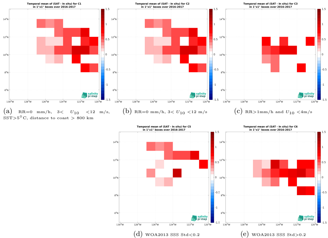
Figure 12: Temporal mean gridded over spatial boxes of size 1^\circ \times 1^\circ of \Delta SSS (SMOS SSS L3 v2 - 9-Days (BEC) - Waveglider (SPURS 2)) for 5 different subdatasets corresponding to:RR=0 mm/h, 3 < U_{10} < 12 m/s, SST >5^\circ C, distance to coast > 800 km (a), RR=0 mm/h, 3 < U_{10} < 12 m/s (b), RR >1 mm/h and U_{10} < 4 m/s (c), WOA2013 SSS Std <0.2 (d), WOA2013 SSS Std >0.2 (e).
