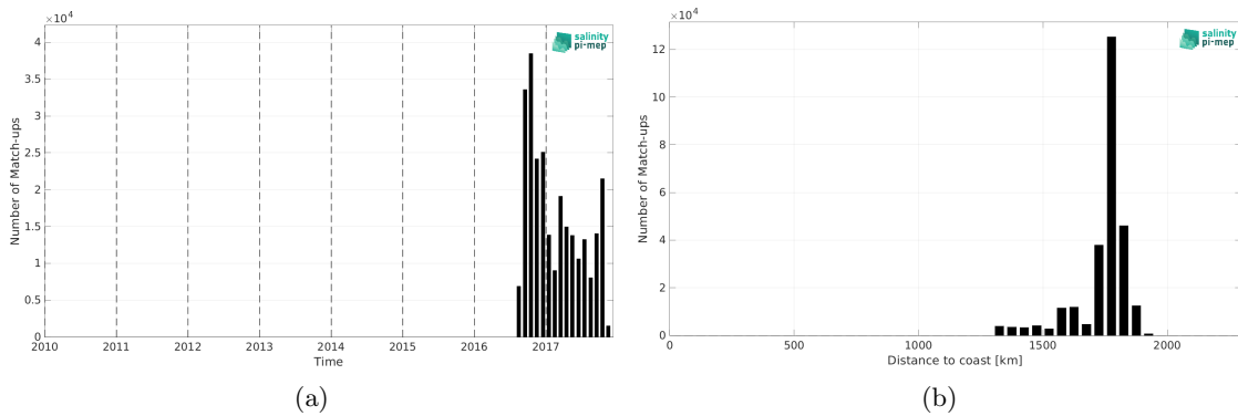
Figure 1: Number of match-ups between Waveglider (SPURS 2) and SMOS SSS L3 v2 - 9-Days (BEC) SSS as a function of time (a) and as function of the distance to coast (b) over the SPURS 2 Pi-MEP region and for the full satellite product period.
