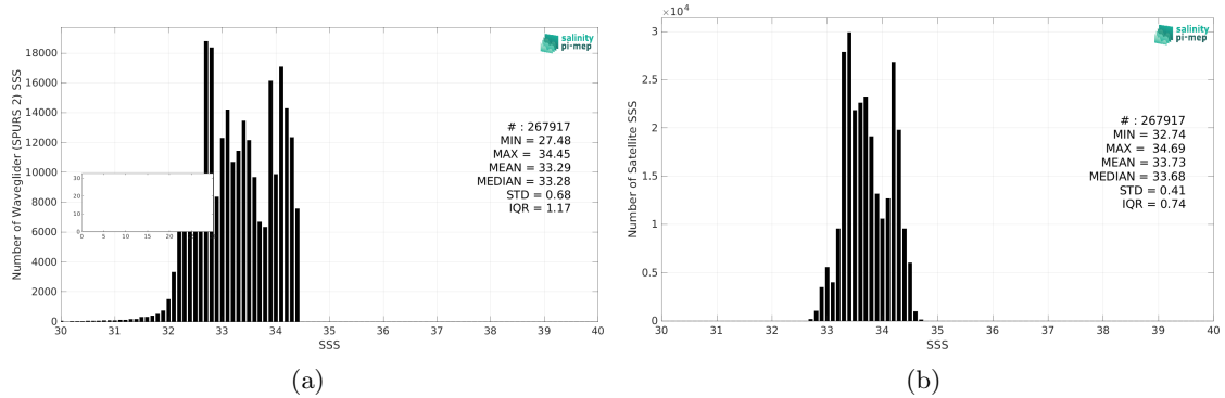
Figure 2: Histograms of SSS from Waveglider (SPURS 2) (a) and SMOS SSS L3 v2 - 9-Days (BEC) (b) considering all match-up pairs per bins of 0.1 over the SPURS 2 Pi-MEP region and for the full satellite product period.
