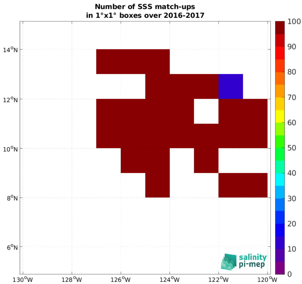
Figure 4: Number of SSS match-ups between Waveglider (SPURS 2) SSS and the SMOS SSS L3 v2 - 9-Days (BEC) SSS product for the SPURS 2 Pi-MEP region over 1^\circ \times 1^\circ boxes and for the full satellite product period.
