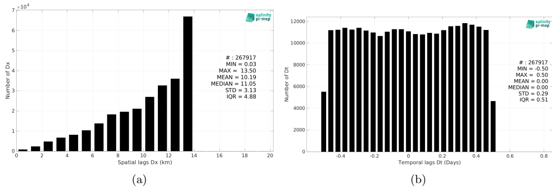
Figure 5: Histograms of the spatial (a) and temporal (b) lags between the location/time of the Waveglider (SPURS 2) measurement and the date of the corresponding SMOS SSS L3 v2 - 9-Days (BEC) SSS pixel.
