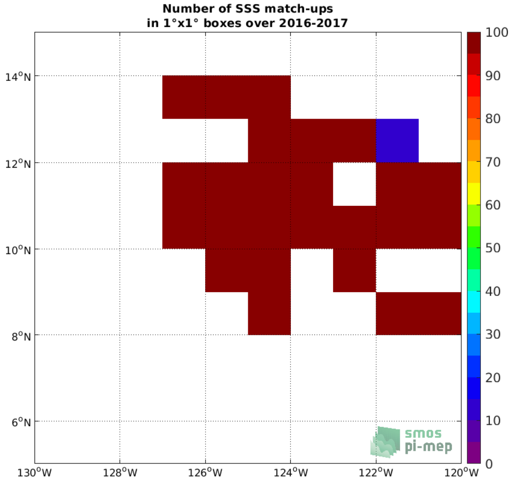
Figure 3: Number of SSS match-ups between Waveglider SSS and the SMOS SSS L3 v2 - 9-Days (BEC) SSS product for the SPURS 2 Pi-MEP region over 1^\circ \times 1^\circ boxes and for the full satellite product period.
