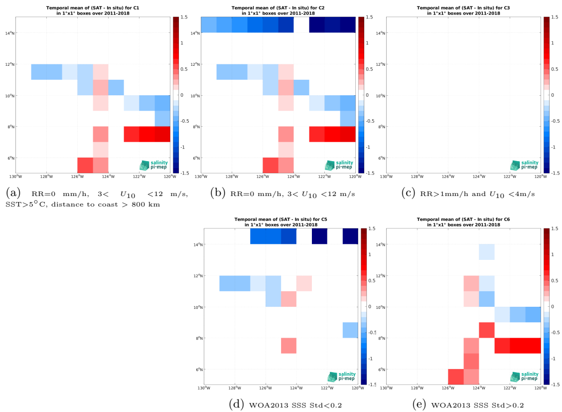
Figure 14: Temporal mean gridded over spatial boxes of size 1^\circ \times 1^\circ of \Delta\text{SSS} (SMOS SSS L3 v2 - 9-Days (BEC) - TSG (SAMOS)) for 5 different subdatasets corresponding to: RR=0 mm/h, 3 < U_{10} < 12 m/s, SST > 5°C, distance to coast > 800 km (a), RR=0 mm/h, 3 < U_{10} < 12 m/s (b), RR > 1mm/h and U_{10} < 4 m/s (c), WOA2013 SSS Std < 0.2 (d), WOA2013 SSS Std > 0.2 (e).
