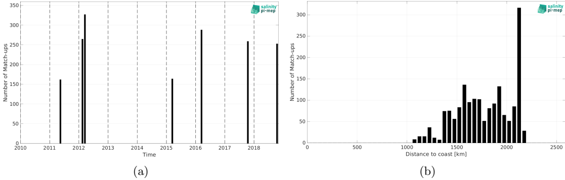
Figure 2: Number of match-ups between TSG (SAMOS) and SMOS SSS L3 v2 - 9-Days (BEC) SSS as a function of time (a) and as function of the distance to coast (b) over the SPURS 2 Pi-MEP region and for the full satellite product period.
