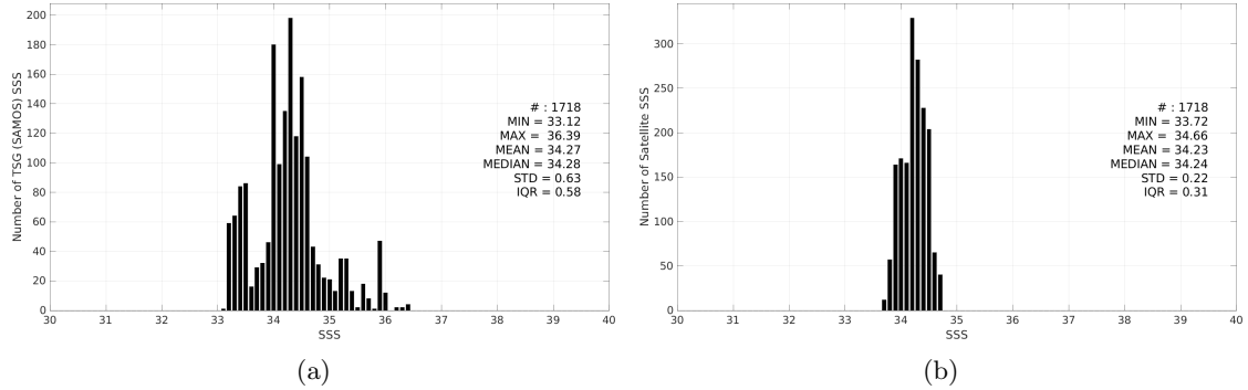
Figure 3: Histograms of SSS from TSG (SAMOS) (a) and SMOS SSS L3 v2 - 9-Days (BEC) (b) considering all match-up pairs per bins of 0.1 over the SPURS 2 Pi-MEP region and for the full satellite product period.
