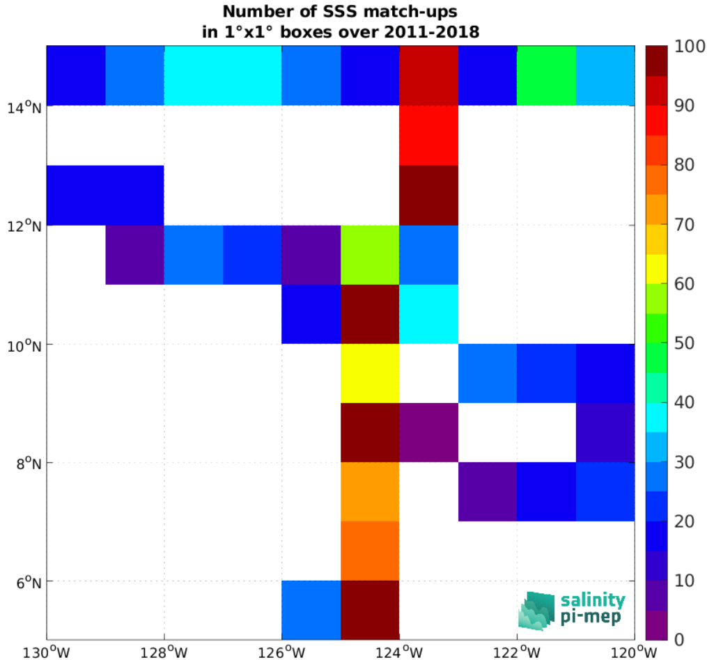
Figure 5: Number of SSS match-ups between TSG (SAMOS) SSS and the SMOS SSS L3 v2 - 9-Days (BEC) SSS product for the SPURS 2 Pi-MEP region over 1^\circ \times 1^\circ boxes and for the full satellite product period.
