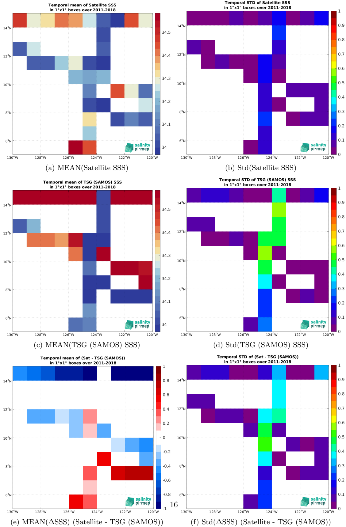
Figure 7: Temporal mean (left) and Std (right) of SSS from SMOS SSS L3 v2 - 9-Days (BEC) (top), TSG (SAMOS) (middle), and of \Delta SSS (Satellite - TSG (SAMOS)). Only match-up pairs are used to generate these maps.
