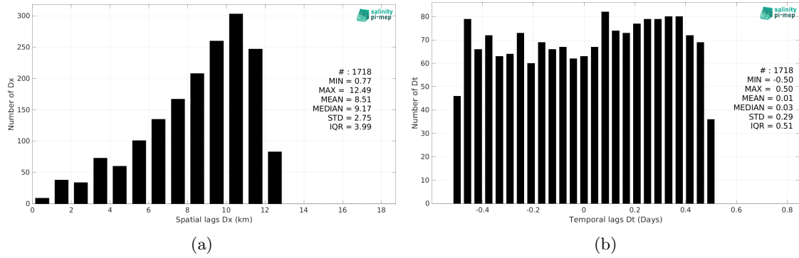
Figure 6: Histograms of the spatial (a) and temporal (b) lags between the location/time of the TSG (SAMOS) measurement and the date of the corresponding SMOS SSS L3 v2 - 9-Days (BEC) SSS pixel.
