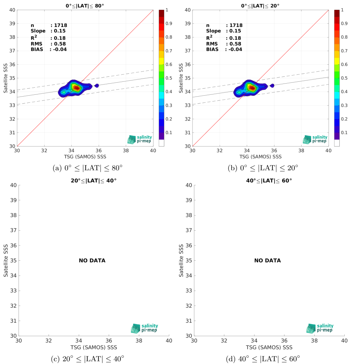
Figure 10: Contour maps of the concentration of SMOS SSS L3 v2 - 9-Days (BEC) SSS (y-axis) versus TSG (SAMOS) SSS (x-axis) at match-up pairs for different latitude bands. For each plot, the red line shows x=y . The black thin and dashed lines indicate a linear fit through the data cloud and the \pm 95\% confidence levels, respectively. The number match-up pairs n , the slope and R^2 coefficient of the linear fit, the root mean square (RMS) and the mean bias between satellite and in situ data are indicated for each latitude band in each plots.
