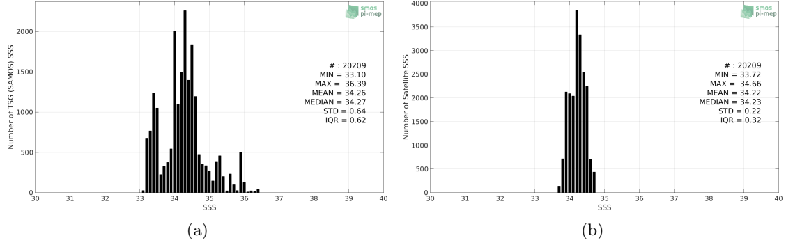
Figure 2: Histograms of SSS from TSG (SAMOS) (a) and SMOS SSS L3 v2 - 9-Days (BEC) (b) considering all match-up pairs per bins of 0.1 over the SPURS 2 Pi-MEP region and for the full satellite product period.
