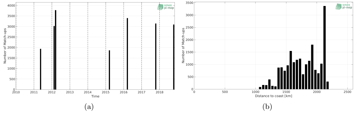
Figure 1: Number of match-ups between TSG (SAMOS) and SMOS SSS L3 v2 - 9-Days (BEC) SSS as a function of time (a) and as function of the distance to coast (b) over the SPURS 2 Pi-MEP region and for the full satellite product period.
