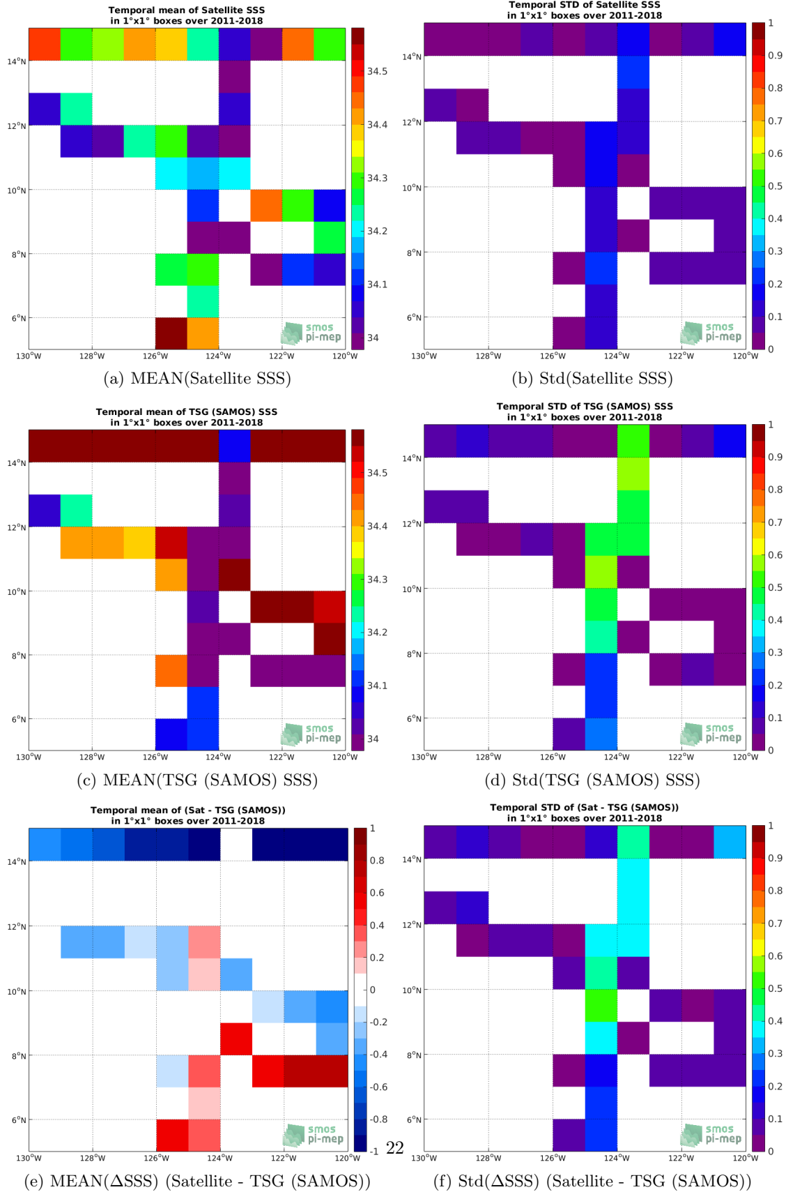
Figure 6: Temporal mean (left) and Std (right) of SSS from SMOS SSS L3 v2 - 9-Days (BEC) (top), TSG (SAMOS) (middle), and of \Delta SSS (Satellite - TSG (SAMOS)). Only match-up pairs are used to generate these maps.
