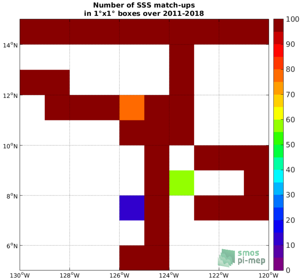
Figure 4: Number of SSS match-ups between TSG (SAMOS) SSS and the SMOS SSS L3 v2 - 9-Days (BEC) SSS product for the SPURS 2 Pi-MEP region over 1°×1° boxes and for the full satellite product period.
