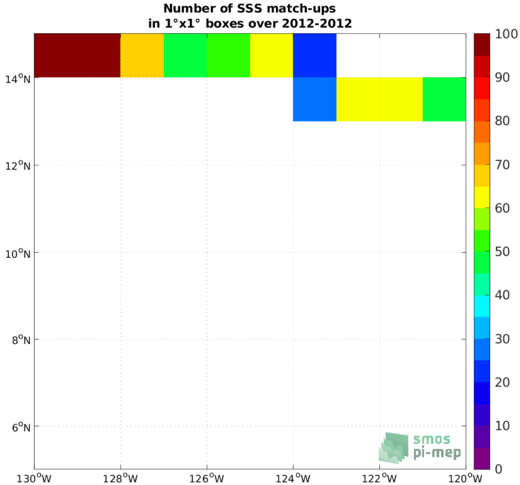
Figure 4: Number of SSS match-ups between TSG (GOSUD-Research-vessel) SSS and the SMOS SSS L3 v2 - 9-Days (BEC) SSS product for the SPURS 2 Pi-MEP region over 1^\circ \times 1^\circ boxes and for the full satellite product period.
