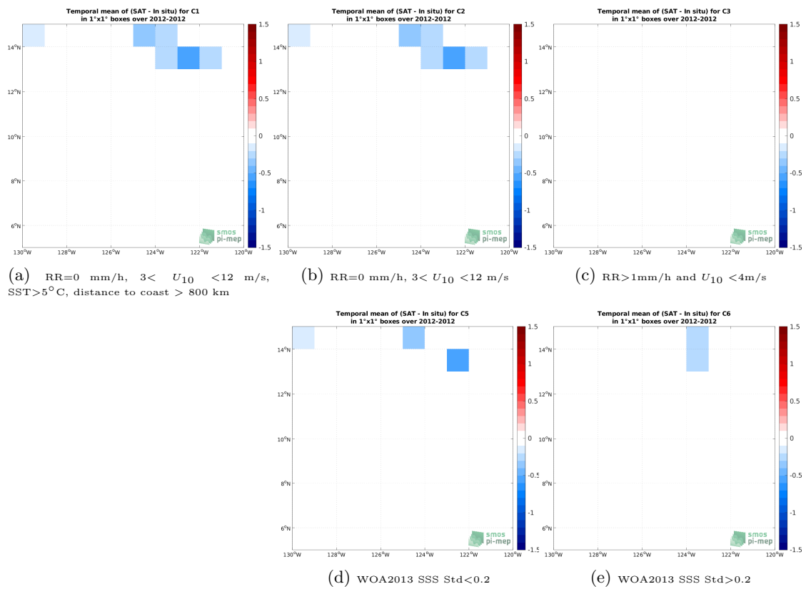
Figure 12: Temporal mean gridded over spatial boxes of size 1^\circ \times 1^\circ of \Delta\text{SSS} (SMOS SSS L3 v2 - 9-Days (BEC) - TSG (GOSUD-Research-vessel)) for 5 different subdatasets corresponding to:RR=0 mm/h, 3 < U_{10} < 12 m/s, SST>5°C, distance to coast > 800 km (a), RR=0 mm/h, 3 < U_{10} < 12 m/s (b), RR>1mm/h and U_{10} < 4 m/s (c), WOA2013 SSS Std<0.2 (d), WOA2013 SSS Std>0.2 (e).
