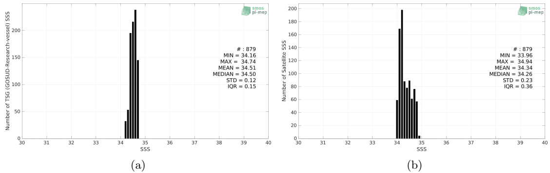
Figure 2: Histograms of SSS from TSG (GOSUD-Research-vessel) (a) and SMOS SSS L3 v2 - 9-Days (BEC) (b) considering all match-up pairs per bins of 0.1 over the SPURS 2 Pi-MEP region and for the full satellite product period.
