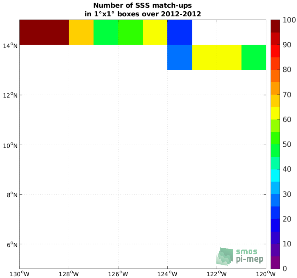
Figure 4: Number of SSS match-ups between TSG (GOSUD-Research-vessel) SSS and the SMOS SSS L3 v2 - 9-Days (BEC) SSS product for the SPURS 2 Pi-MEP region over 1°x1° boxes and for the full satellite product period.
