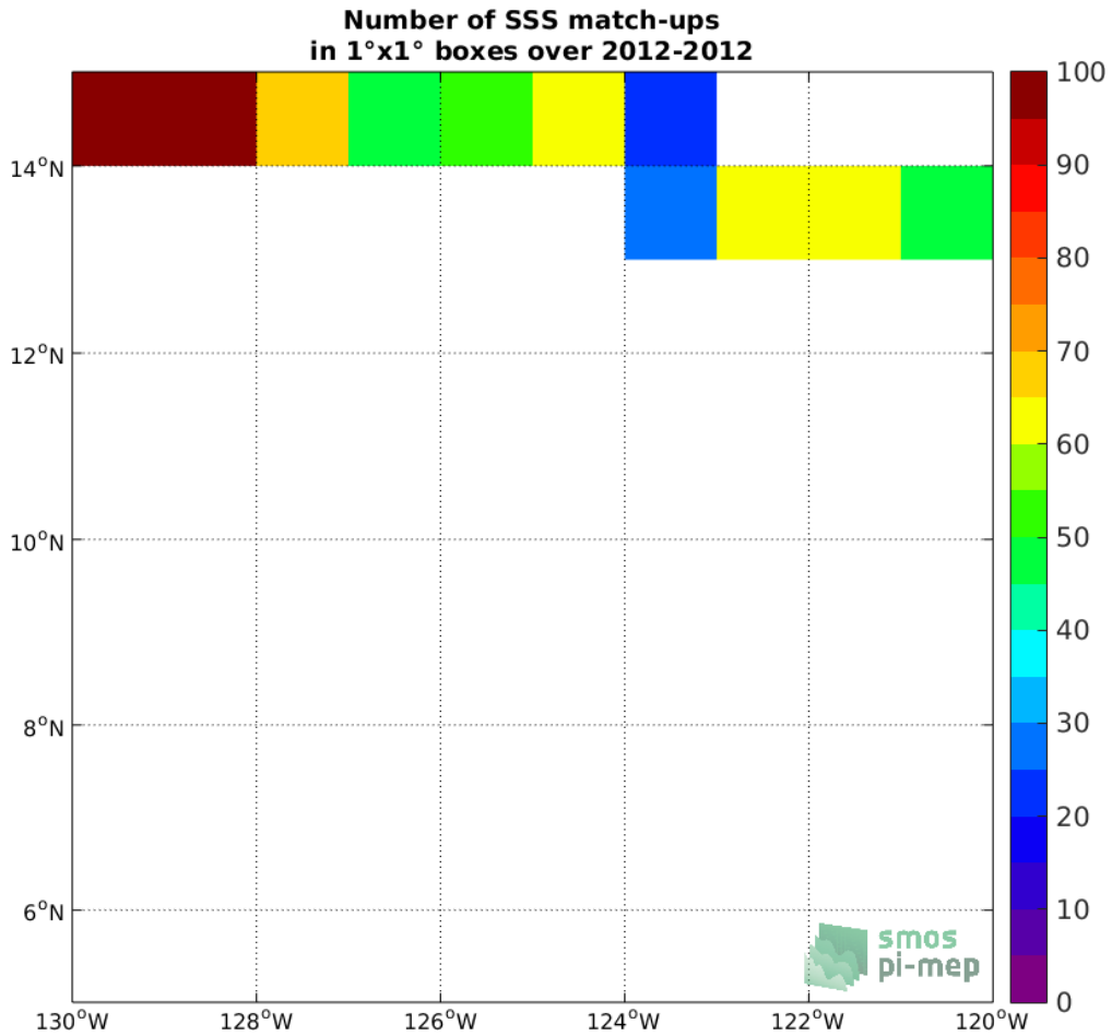
Figure 4: Number of SSS match-ups between TSG (GOSUD-Research-vessel) SSS and the SMOS SSS L3 v2 - 9-Days (BEC) SSS product for the SPURS 2 Pi-MEP region over 1°×1° boxes and for the full satellite product period.
