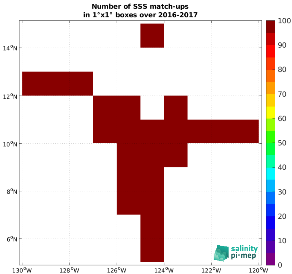
Figure 4: Number of SSS match-ups between Salinity Snake (SPURS 2) SSS and the SMOS SSS L3 v2 - 9-Days (BEC) SSS product for the SPURS 2 Pi-MEP region over 1^{\circ} \times 1^{\circ} boxes and for the full satellite product period.
