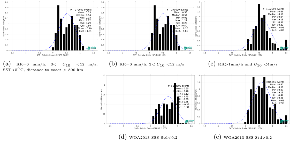
Figure 13: Normalized histogram of \Delta SSS (SMOS SSS L3 v2 - 9-Days (BEC) - Salinity Snake (SPURS 2)) for 5 different subdatasets corresponding to: RR=0 mm/h, 3 < U_{10} < 12 m/s, SST>5°C, distance to coast > 800 km (a), RR=0 mm/h, 3 < U_{10} < 12 m/s (b), RR>1mm/h and U_{10} < 4 m/s (c), WOA2013 SSS Std<0.2 (d), WOA2013 SSS Std>0.2 (e).
