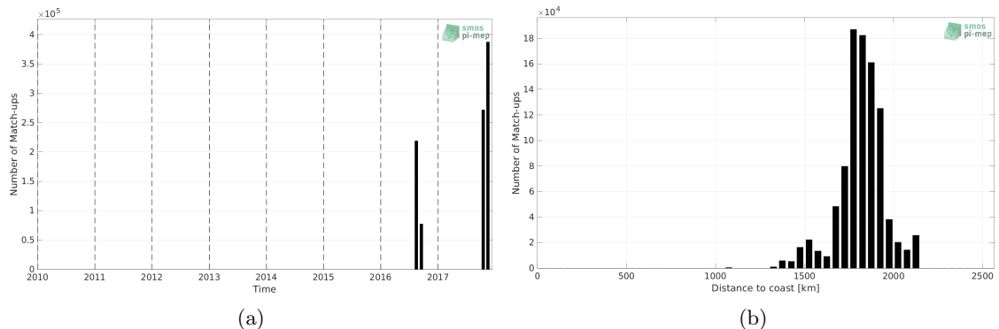
Figure 1: Number of match-ups between Salinity Snake and SMOS SSS L3 v2 - 9-Days (BEC) SSS as a function of time (a) and as function of the distance to coast (b) over the SPURS 2 Pi-MEP region and for the full satellite product period.
