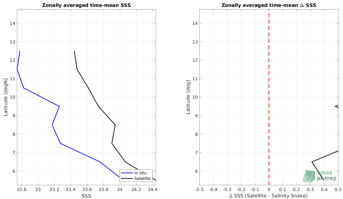
Figure 8: Left panel: Zonal mean SSS from SMOS SSS L3 v2 - 9-Days (BEC) satellite product (black) and from Salinity Snake (blue). Right panel: Zonal mean of \Delta SSS (Satellite - Salinity Snake) for all the collected Pi-MEP match-up pairs estimated over the full satellite product period.
