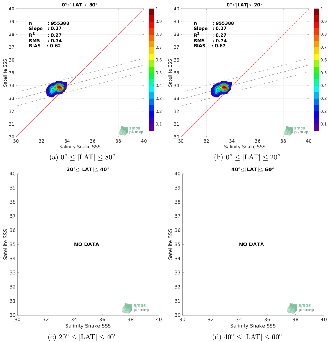
Figure 9: Contour maps of the concentration of SMOS SSS L3 v2 - 9-Days (BEC) SSS (y-axis) versus Salinity Snake SSS (x-axis) at match-up pairs for different latitude bands. For each plot, the red line shows x=y . The black thin and dashed lines indicate a linear fit through the data cloud and the \pm 95\% confidence levels, respectively. The number match-up pairs n , the slope and R^2 coefficient of the linear fit, the root mean square (RMS) and the mean bias between satellite and in situ data are indicated for each latitude band in each plots.
