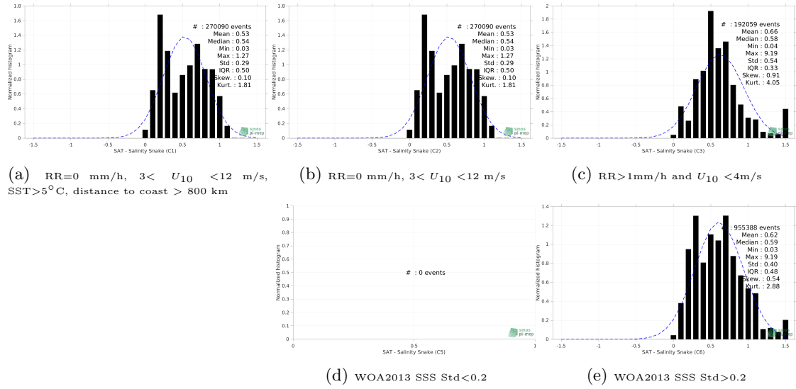
Figure 13: Normalized histogram of \Delta SSS (SMOS SSS L3 v2 - 9-Days (BEC) - Salinity Snake) for 5 different subdatasets corresponding to: RR=0 mm/h, 3 < U_{10} < 12 m/s, SST > 5°C, distance to coast > 800 km (a), RR=0 mm/h, 3 < U_{10} < 12 m/s (b), RR > 1mm/h and U_{10} < 4 m/s (c), WOA2013 SSS Std < 0.2 (d), WOA2013 SSS Std > 0.2 (e).
