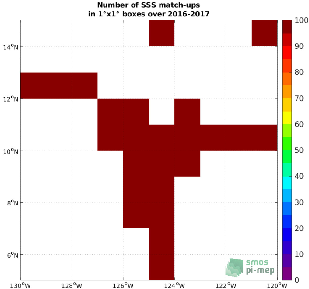
Figure 4: Number of SSS match-ups between Salinity Snake SSS and the SMOS SSS L3 v2 - 9-Days (BEC) SSS product for the SPURS 2 Pi-MEP region over 1^\circ \times 1^\circ boxes and for the full satellite product period.
