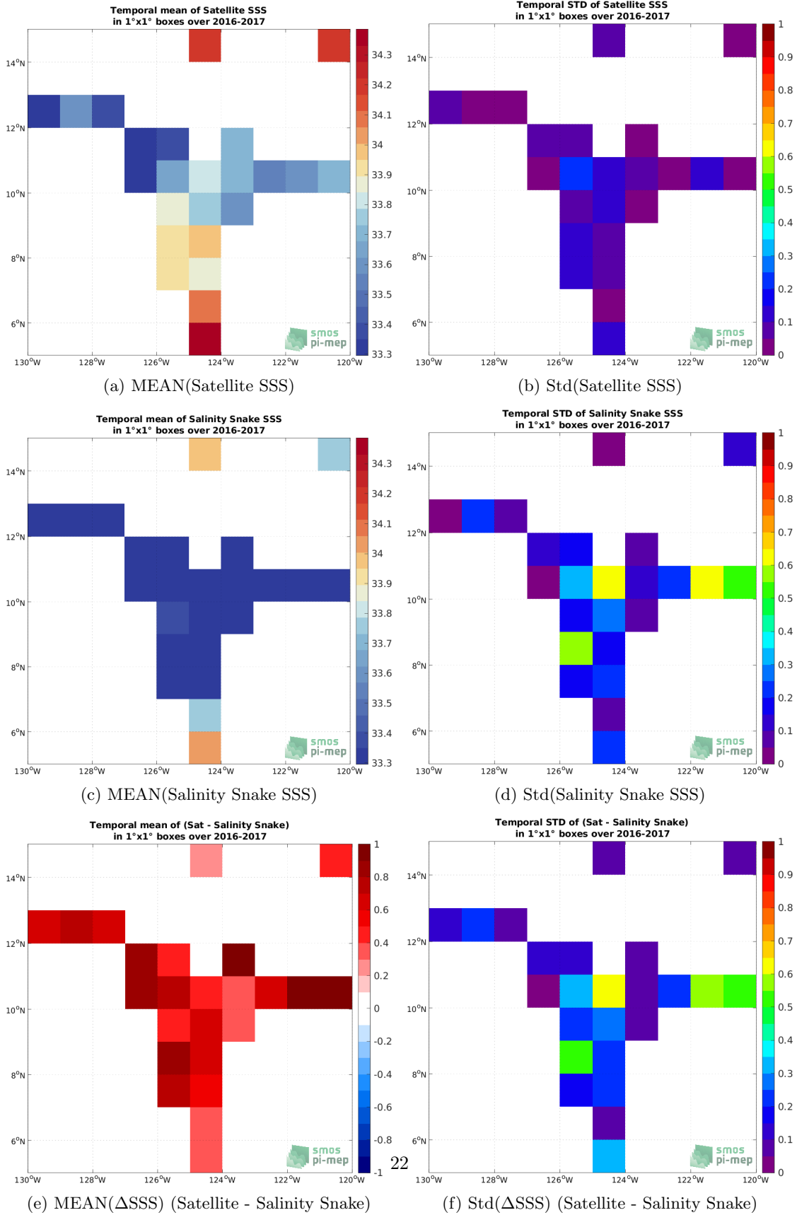
Figure 6: Temporal mean (left) and Std (right) of SSS from SMOS SSS L3 v2 - 9-Days (BEC) (top), Salinity Snake (middle), and of \Delta SSS (Satellite - Salinity Snake). Only match-up pairs are used to generate these maps.
