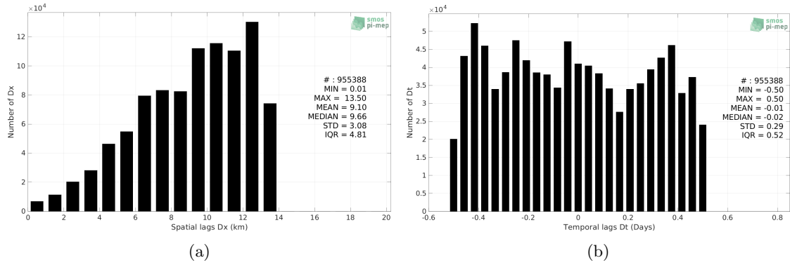
Figure 5: Histograms of the spatial (a) and temporal (b) lags between the location/time of the Salinity Snake measurement and the date of the corresponding SMOS SSS L3 v2 - 9-Days (BEC) SSS pixel.
