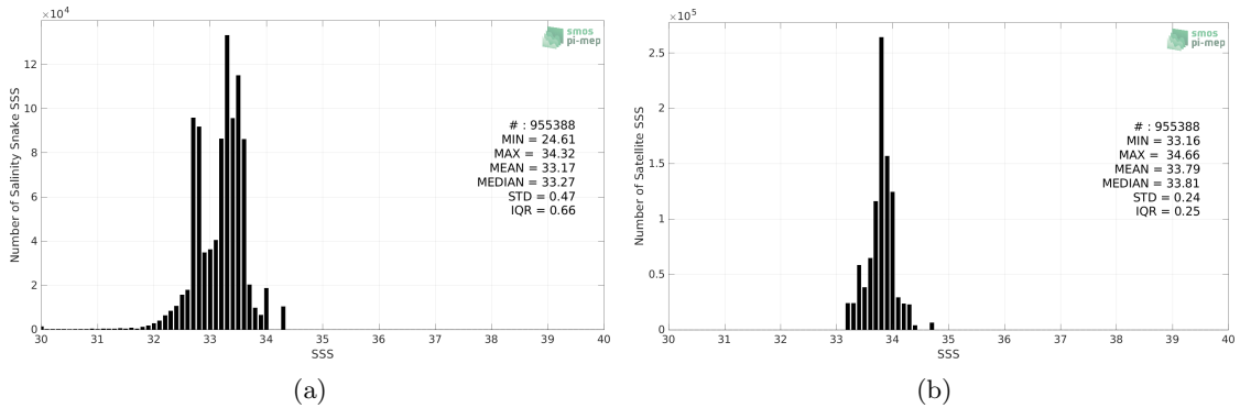
Figure 2: Histograms of SSS from Salinity Snake (a) and SMOS SSS L3 v2 - 9-Days (BEC) (b) considering all match-up pairs per bins of 0.1 over the SPURS 2 Pi-MEP region and for the full satellite product period.
