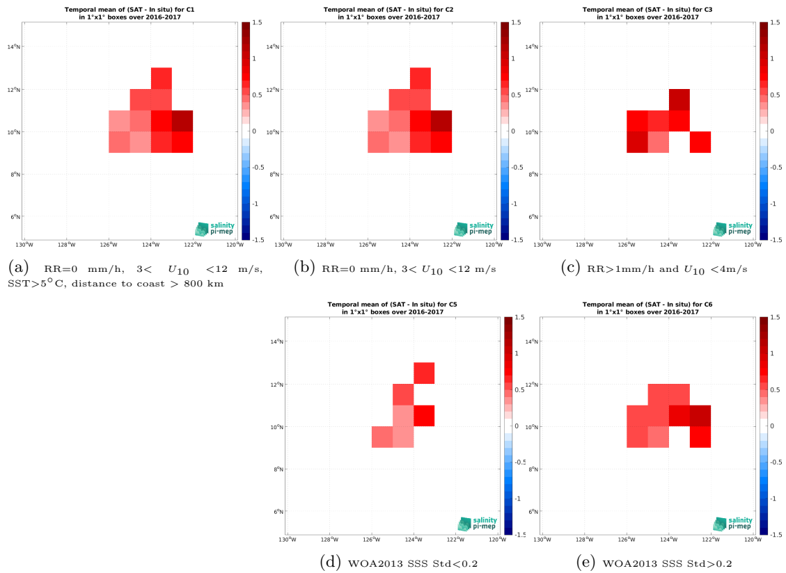
Figure 14: Temporal mean gridded over spatial boxes of size 1^\circ \times 1^\circ of \Delta SSS (SMOS SSS L3 v2 - 9-Days (BEC) - Seaglider (SPURS 2)) for 5 different subdatasets corresponding to:RR=0 mm/h, 3 < U_{10} < 12 m/s, SST > 5°C, distance to coast > 800 km (a), RR=0 mm/h, 3 < U_{10} < 12 m/s (b), RR > 1mm/h and U_{10} < 4 m/s (c), WOA2013 SSS Std < 0.2 (d), WOA2013 SSS Std > 0.2 (e).
