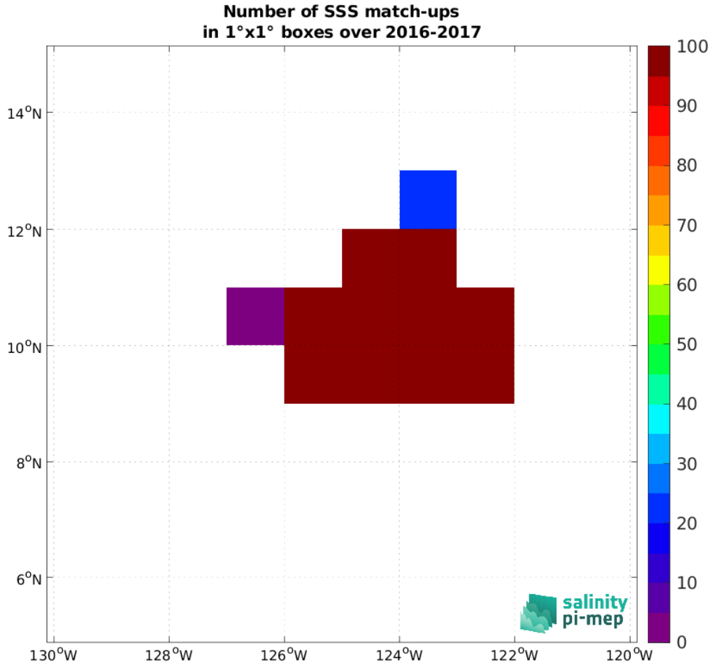
Figure 5: Number of SSS match-ups between Seaglider (SPURS 2) SSS and the SMOS SSS L3 v2 - 9-Days (BEC) SSS product for the SPURS 2 Pi-MEP region over 1^\circ \times 1^\circ boxes and for the full satellite product period.
