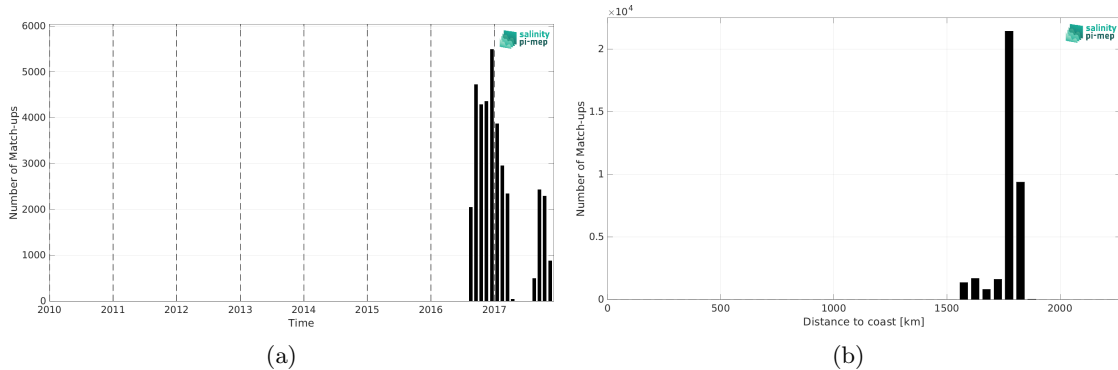
Figure 2: Number of match-ups between Seaglider (SPURS 2) and SMOS SSS L3 v2 - 9-Days (BEC) SSS as a function of time (a) and as function of the distance to coast (b) over the SPURS 2 Pi-MEP region and for the full satellite product period.
