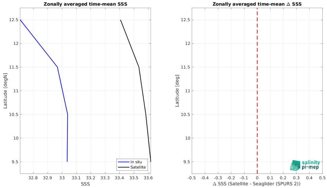
Figure 9: Left panel: Zonal mean SSS from SMOS SSS L3 v2 - 9-Days (BEC) satellite product (black) and from Seaglider (SPURS 2) (blue). Right panel: Zonal mean of \Delta SSS (Satellite - Seaglider (SPURS 2)) for all the collected Pi-MEP match-up pairs estimated over the full satellite product period.
