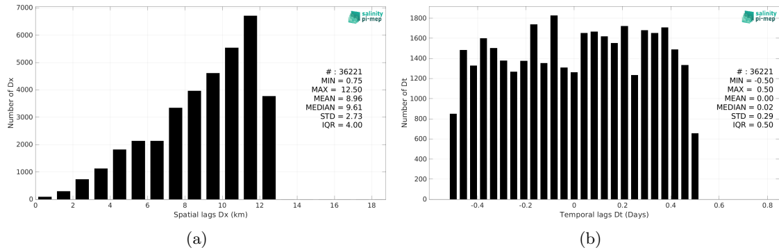
Figure 6: Histograms of the spatial (a) and temporal (b) lags between the location/time of the Seaglider (SPURS 2) measurement and the date of the corresponding SMOS SSS L3 v2 - 9-Days (BEC) SSS pixel.
