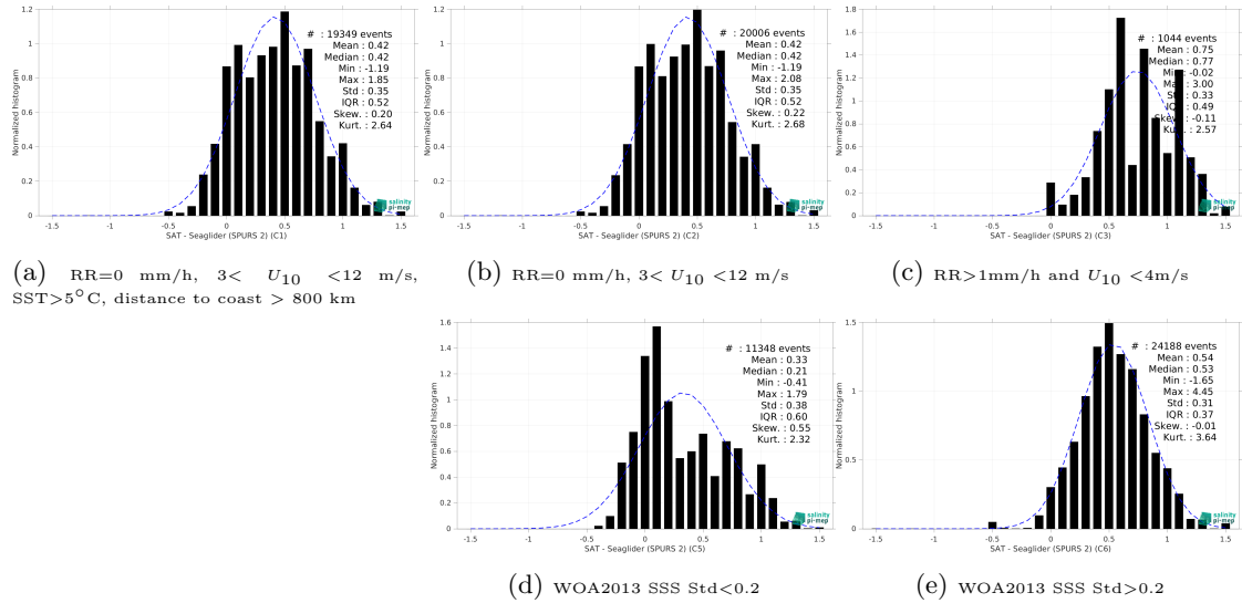
Figure 15: Normalized histogram of \Delta SSS (SMOS SSS L3 v2 - 9-Days (BEC) - Seaglider (SPURS 2)) for 5 different subdatasets corresponding to: RR=0 mm/h, 3 < U_{10} < 12 m/s, SST > 5°C, distance to coast > 800 km (a), RR=0 mm/h, 3 < U_{10} < 12 m/s (b), RR > 1mm/h and U_{10} < 4 m/s (c), WOA2013 SSS Std < 0.2 (d), WOA2013 SSS Std > 0.2 (e).
