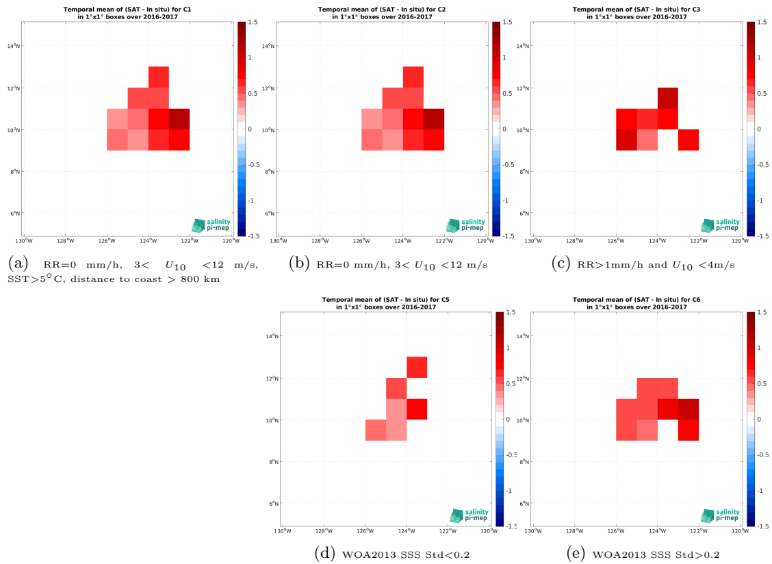
Figure 14: Temporal mean gridded over spatial boxes of size 1^\circ \times 1^\circ of \Delta\text{SSS} (SMOS SSS L3 v2 - 9-Days (BEC) - Seaglider (SPURS 2)) for 5 different subdatasets corresponding to:RR=0 mm/h, 3 < U_{10} < 12 m/s, SST>5°C, distance to coast > 800 km (a), RR=0 mm/h, 3 < U_{10} < 12 m/s (b), RR>1mm/h and U_{10} < 4 m/s (c), WOA2013 SSS Std<0.2 (d), WOA2013 SSS Std>0.2 (e).
