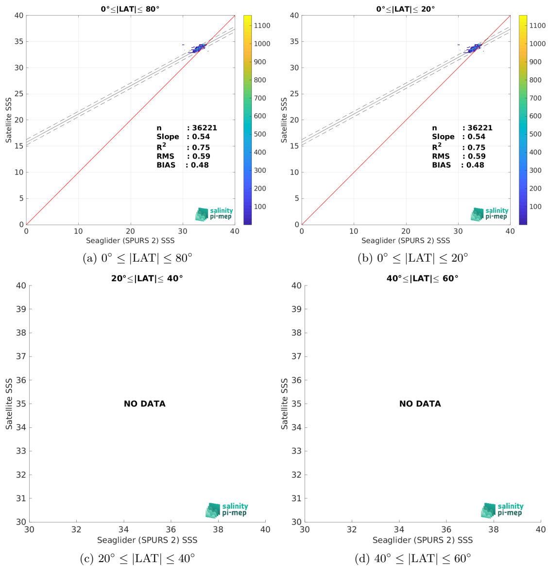
Figure 10: Contour maps of the concentration of SMOS SSS L3 v2 - 9-Days (BEC) SSS (y-axis) versus Seaglider (SPURS 2) SSS (x-axis) at match-up pairs for different latitude bands. For each plot, the red line shows x=y . The black thin and dashed lines indicate a linear fit through the data cloud and the \pm 95\% confidence levels, respectively. The number match-up pairs n , the slope and R^2 coefficient of the linear fit, the root mean square (RMS) and the mean bias between satellite and in situ data are indicated for each latitude band in each plots.
