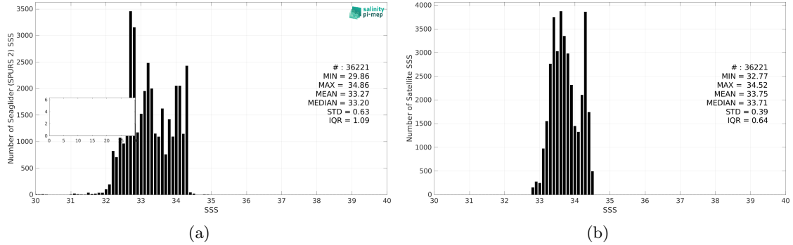
Figure 3: Histograms of SSS from Seaglider (SPURS 2) (a) and SMOS SSS L3 v2 - 9-Days (BEC) (b) considering all match-up pairs per bins of 0.1 over the SPURS 2 Pi-MEP region and for the full satellite product period.
