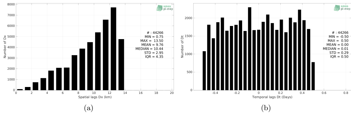
Figure 5: Histograms of the spatial (a) and temporal (b) lags between the location/time of the Seaglider measurement and the date of the corresponding SMOS SSS L3 v2 - 9-Days (BEC) SSS pixel.
