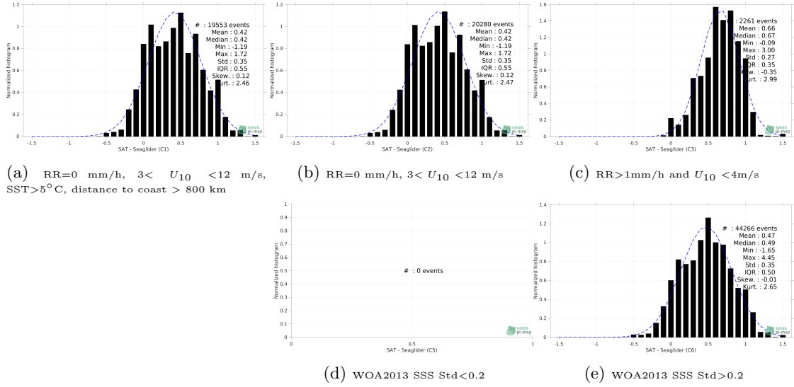
Figure 13: Normalized histogram of \Delta SSS (SMOS SSS L3 v2 - 9-Days (BEC) - Seaglider) for 5 different subdatasets corresponding to: RR=0 mm/h, 3 < U_{10} < 12 m/s, SST>5°C, distance to coast > 800 km (a), RR=0 mm/h, 3 < U_{10} < 12 m/s (b), RR>1mm/h and U_{10} < 4 m/s (c), WOA2013 SSS Std<0.2 (d), WOA2013 SSS Std>0.2 (e).
