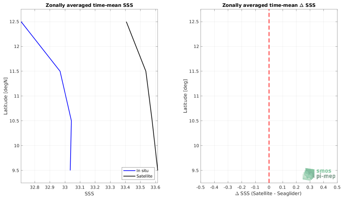
Figure 8: Left panel: Zonal mean SSS from SMOS SSS L3 v2 - 9-Days (BEC) satellite product (black) and from Seaglider (blue). Right panel: Zonal mean of \Delta SSS (Satellite - Seaglider) for all the collected Pi-MEP match-up pairs estimated over the full satellite product period.
