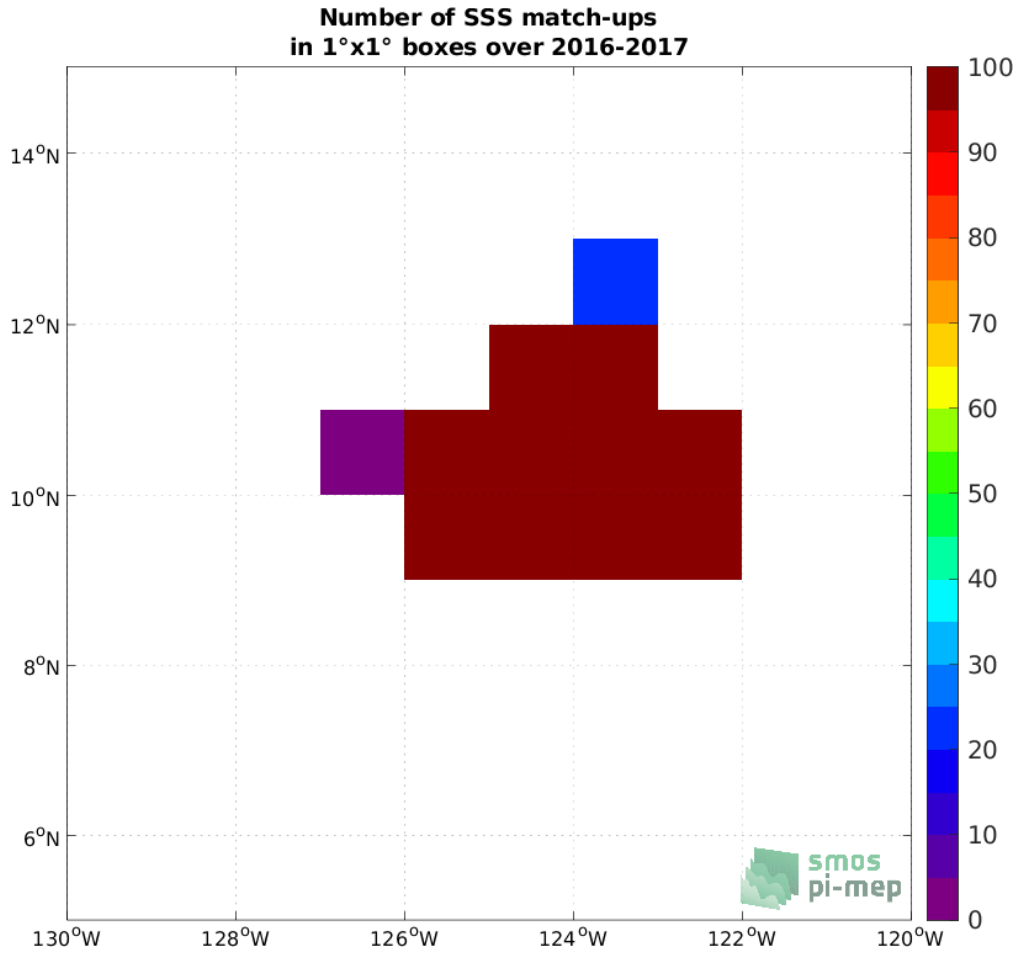
Figure 4: Number of SSS match-ups between Seaglider SSS and the SMOS SSS L3 v2 - 9-Days (BEC) SSS product for the SPURS 2 Pi-MEP region over 1°x1° boxes and for the full satellite product period.
