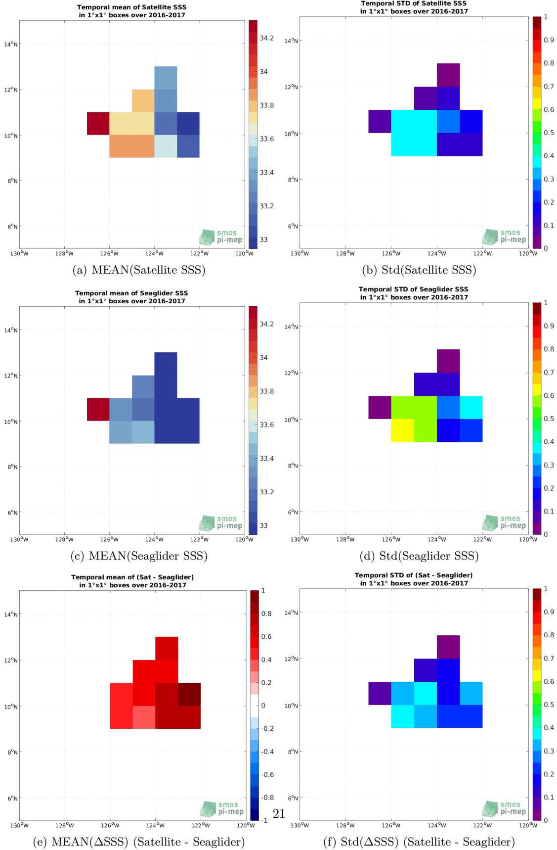
Figure 6: Temporal mean (left) and Std (right) of SSS from SMOS SSS L3 v2 - 9-Days (BEC) (top), Seaglider (middle), and of \Delta SSS (Satellite - Seaglider). Only match-up pairs are used to generate these maps.
