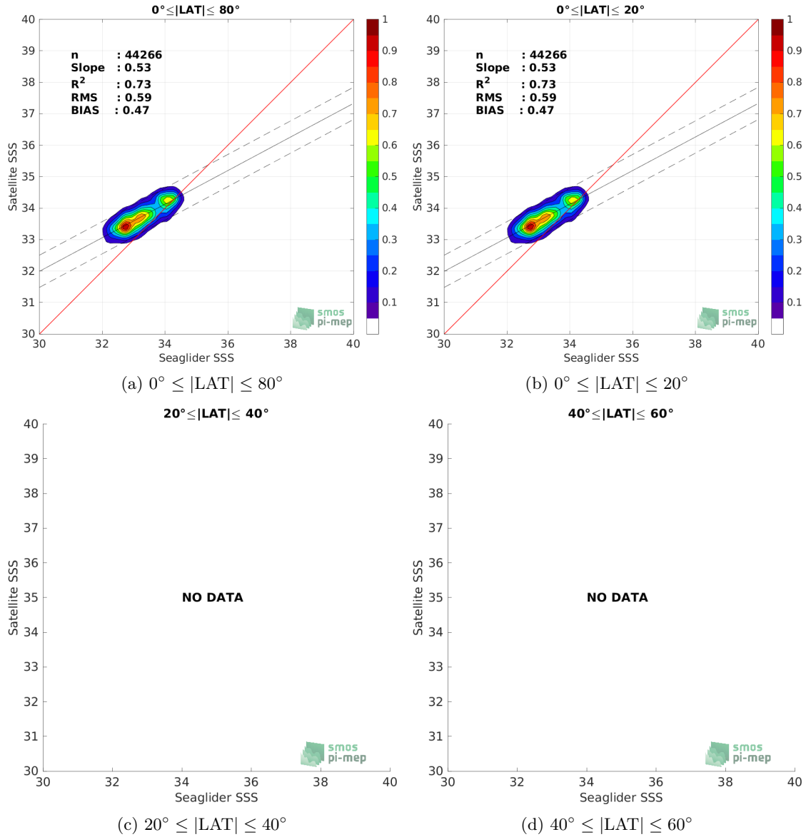
Figure 9: Contour maps of the concentration of SMOS SSS L3 v2 - 9-Days (BEC) SSS (y-axis) versus Seaglider SSS (x-axis) at match-up pairs for different latitude bands. For each plot, the red line shows x=y . The black thin and dashed lines indicate a linear fit through the data cloud and the \pm 95\% confidence levels, respectively. The number match-up pairs n , the slope and R^2 coefficient of the linear fit, the root mean square (RMS) and the mean bias between satellite and in situ data are indicated for each latitude band in each plots.
