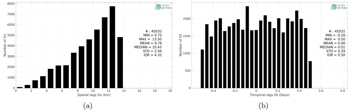
Figure 4: Histograms of the spatial (a) and temporal (b) lags between the location/time of the Seaglider measurement and the date of the corresponding SMOS SSS L3 v2 - 9-Days (BEC) SSS pixel.
