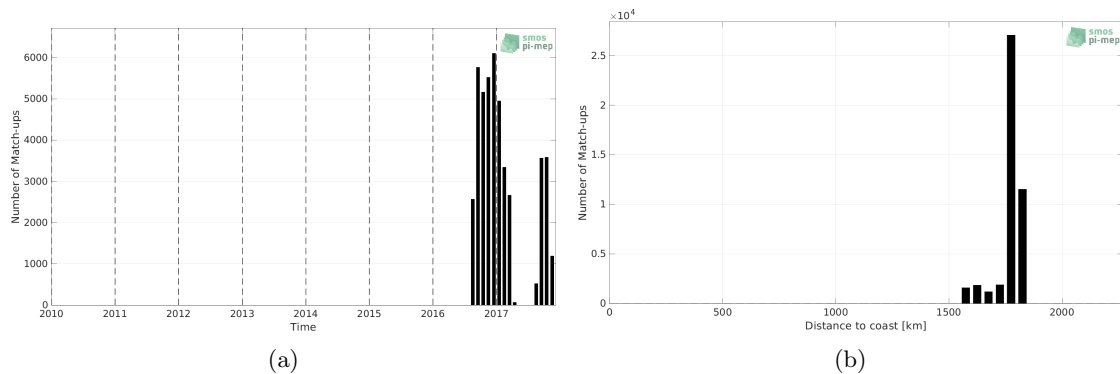
Figure 1: Number of match-ups between Seaglider and SMOS SSS L3 v2 - 9-Days (BEC) SSS as a function of time (a) and as function of the distance to coast (b) over the SPURS 2 Pi-MEP region and for the full satellite product period.
