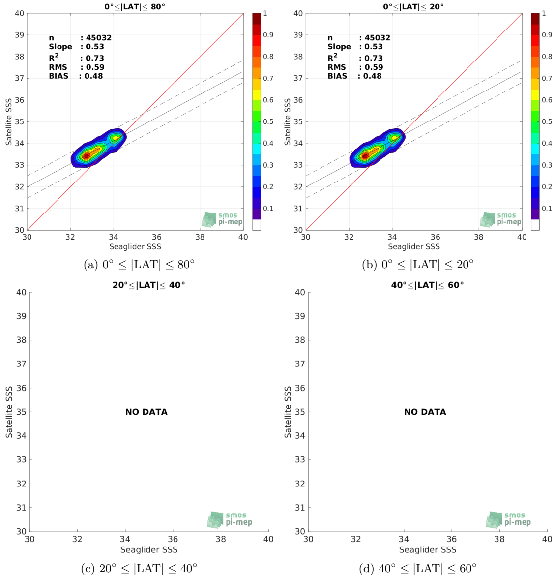
Figure 8: Contour maps of the concentration of SMOS SSS L3 v2 - 9-Days (BEC) SSS (y-axis) versus Seaglider SSS (x-axis) at match-up pairs for different latitude bands. For each plot, the red line shows x=y . The black thin and dashed lines indicate a linear fit through the data cloud and the \pm 95\% confidence levels, respectively. The number match-up pairs n , the slope and R^2 coefficient of the linear fit, the root mean square (RMS) and the mean bias between satellite and in situ data are indicated for each latitude band in each plots.
