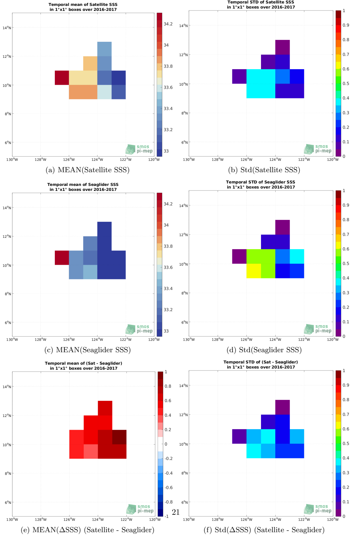
Figure 5: Temporal mean (left) and Std (right) of SSS from SMOS SSS L3 v2 - 9-Days (BEC) (top), Seaglider (middle), and of \Delta SSS (Satellite - Seaglider). Only match-up pairs are used to generate these maps.
