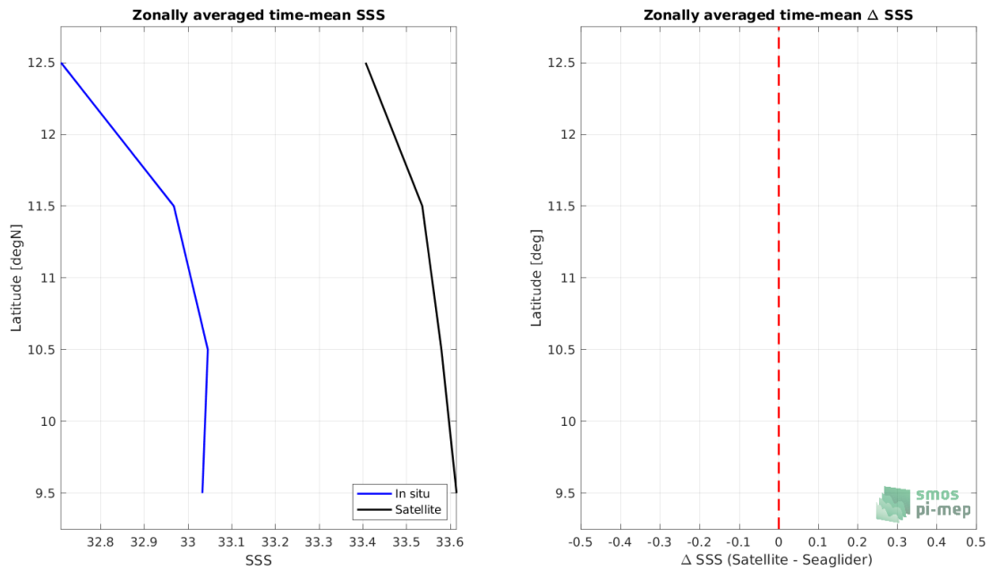
Figure 7: Left panel: Zonal mean SSS from SMOS SSS L3 v2 - 9-Days (BEC) satellite product (black) and from Seaglider (blue). Right panel: Zonal mean of \Delta SSS (Satellite - Seaglider) for all the collected Pi-MEP match-up pairs estimated over the full satellite product period.
