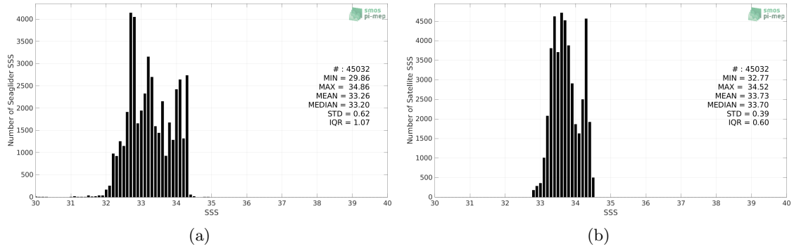
Figure 2: Histograms of SSS from Seaglader (a) and SMOS SSS L3 v2 - 9-Days (BEC) (b) considering all match-up pairs per bins of 0.1 over the SPURS 2 Pi-MEP region and for the full satellite product period.
