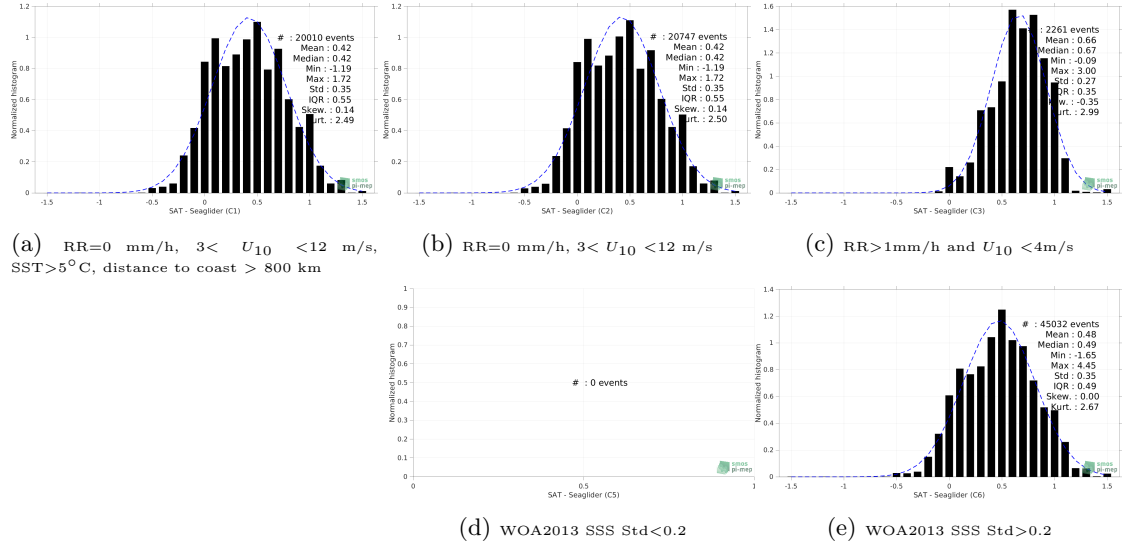
Figure 12: Normalized histogram of \Delta SSS (SMOS SSS L3 v2 - 9-Days (BEC) - Seaglider) for 5 different subdatasets corresponding to: RR=0 mm/h, 3 < U_{10} < 12 m/s, SST>5°C, distance to coast > 800 km (a), RR=0 mm/h, 3 < U_{10} < 12 m/s (b), RR>1mm/h and U_{10} < 4 m/s (c), WOA2013 SSS Std<0.2 (d), WOA2013 SSS Std>0.2 (e).
