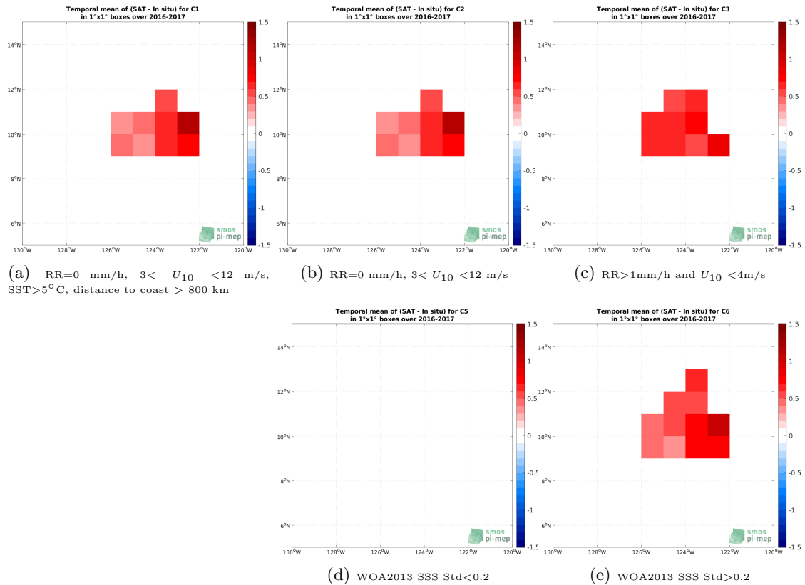
Figure 11: Temporal mean gridded over spatial boxes of size 1^\circ \times 1^\circ of \Delta SSS (SMOS SSS L3 v2 - 9-Days (BEC) - Seaglider) for 5 different subdatasets corresponding to:RR=0 mm/h, 3 < U_{10} < 12 m/s, SST >5^\circ C, distance to coast > 800 km (a), RR=0 mm/h, 3 < U_{10} < 12 m/s (b), RR >1 mm/h and U_{10} < 4 m/s (c), WOA2013 SSS Std <0.2 (d), WOA2013 SSS Std >0.2 (e).
