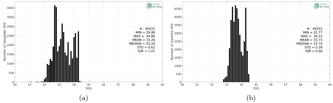
Figure 2: Histograms of SSS from Seaglider (a) and SMOS SSS L3 v2 - 9-Days (BEC) (b) considering all match-up pairs per bins of 0.1 over the SPURS 2 Pi-MEP region and for the full satellite product period.
