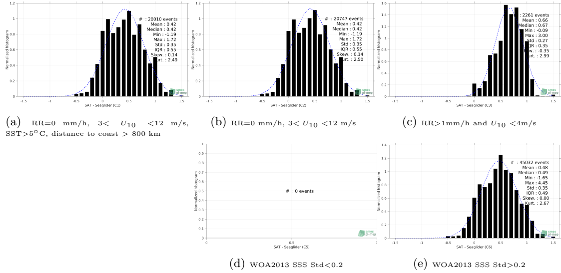
Figure 12: Normalized histogram of \Delta SSS (SMOS SSS L3 v2 - 9-Days (BEC) - Seaglider) for 5 different subdatasets corresponding to: RR=0 mm/h, 3 < U_{10} < 12 m/s, SST > 5°C, distance to coast > 800 km (a), RR=0 mm/h, 3 < U_{10} < 12 m/s (b), RR > 1mm/h and U_{10} < 4 m/s (c), WOA2013 SSS Std < 0.2 (d), WOA2013 SSS Std > 0.2 (e).
