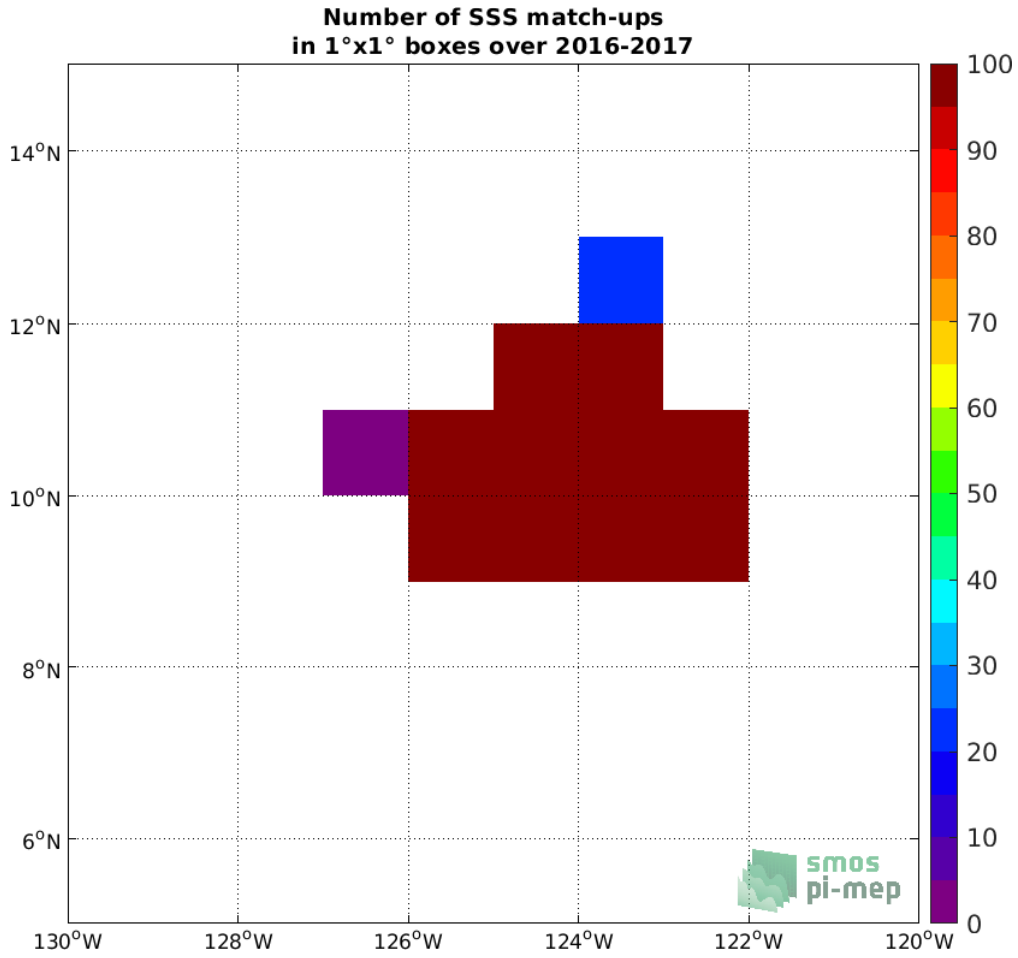
Figure 3: Number of SSS match-ups between Seagliders SSS and the SMOS SSS L3 v2 - 9-Days (BEC) SSS product for the SPURS 2 Pi-MEP region over 1^\circ \times 1^\circ boxes and for the full satellite product period.
