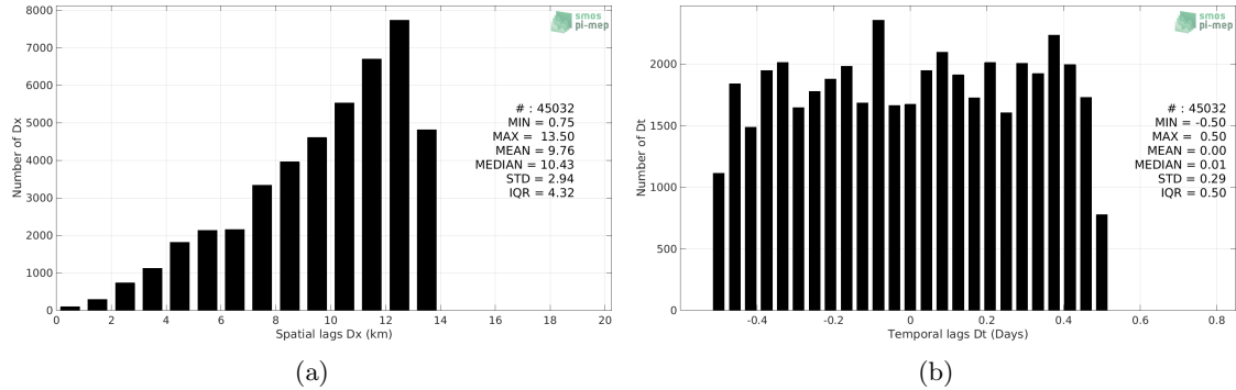
Figure 5: Histograms of the spatial (a) and temporal (b) lags between the time of the Seaglider measurements and the date of the corresponding SMOS SSS L3 v2 - 9-Days (BEC) SSS product.
