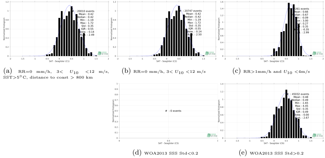
Figure 13: Normalized histogram of \Delta SSS (SMOS SSS L3 v2 - 9-Days (BEC) - Seaglider) for 5 different subdatasets corresponding to: RR=0 mm/h, 3 < U_{10} < 12 m/s, SST > 5°C, distance to coast > 800 km (a), RR=0 mm/h, 3 < U_{10} < 12 m/s (b), RR > 1mm/h and U_{10} < 4 m/s (c), WOA2013 SSS Std < 0.2 (d), WOA2013 SSS Std > 0.2 (e).
