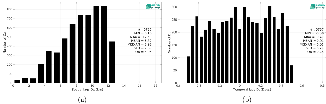
Figure 6: Histograms of the spatial (a) and temporal (b) lags between the location/time of the Saildrone (SPURS 2) measurement and the date of the corresponding SMOS SSS L3 v2 - 9-Days (BEC) SSS pixel.
