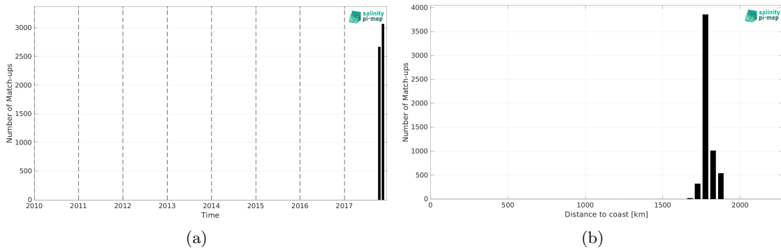
Figure 2: Number of match-ups between Saildrone (SPURS 2) and SMOS SSS L3 v2 - 9-Days (BEC) SSS as a function of time (a) and as function of the distance to coast (b) over the SPURS 2 Pi-MEP region and for the full satellite product period.
