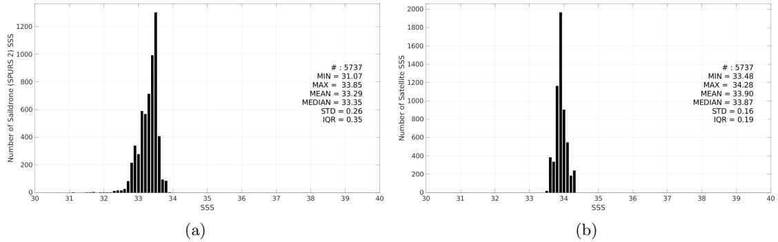
Figure 3: Histograms of SSS from Saildrone (SPURS 2) (a) and SMOS SSS L3 v2 - 9-Days (BEC) (b) considering all match-up pairs per bins of 0.1 over the SPURS 2 Pi-MEP region and for the full satellite product period.
