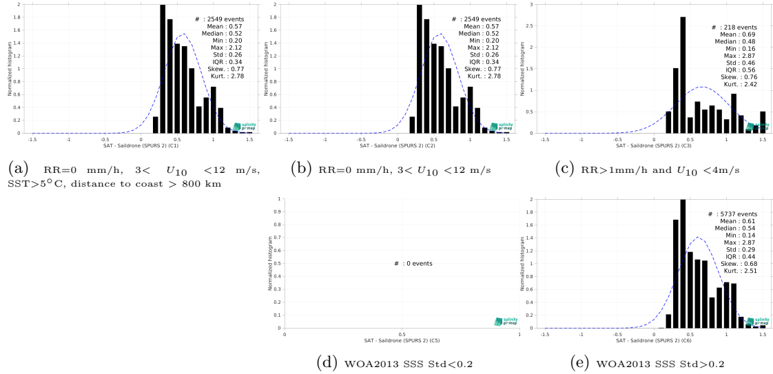
Figure 15: Normalized histogram of \Delta\text{SSS} (SMOS SSS L3 v2 - 9-Days (BEC) - Saildrone (SPURS 2)) for 5 different subdatasets corresponding to: RR=0 mm/h, 3 < U_{10} < 12 m/s, SST > 5^\circ\text{C} , distance to coast > 800 km (a), RR=0 mm/h, 3 < U_{10} < 12 m/s (b), RR > 1\text{mm/h} and U_{10} < 4\text{m/s} (c), WOA2013 SSS \text{Std} < 0.2 (d), WOA2013 SSS \text{Std} > 0.2 (e).
