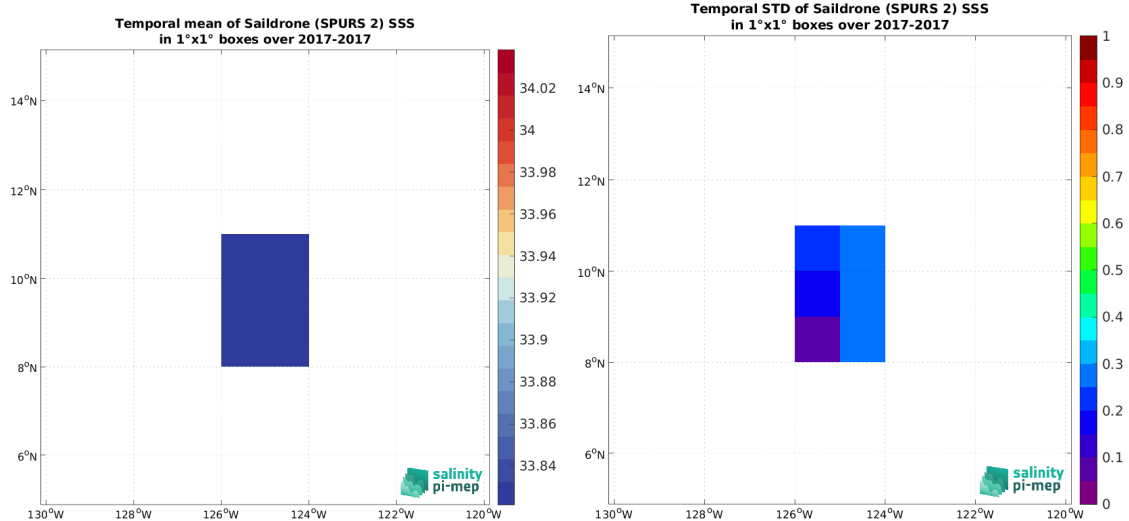
(c) MEAN(Saildrone (SPURS 2) SSS)
