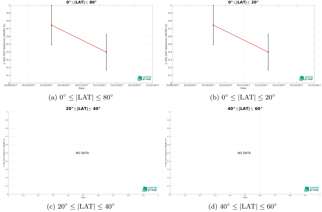
Figure 11: Monthly median (red curves) of \Delta\text{SSS} (Satellite - Saildrone (SPURS 2)) and \pm 1 Std (black vertical thick bars) as function of time for all the collected Pi-MEP match-up pairs estimated over the SPURS 2 Pi-MEP region and for the full satellite product period are shown for different latitude bands: (a) 80^{\circ}\text{S}-80^{\circ}\text{N} , (b) 20^{\circ}\text{S}-20^{\circ}\text{N} , (c) 40^{\circ}\text{S}-20^{\circ}\text{S} and 20^{\circ}\text{N}-40^{\circ}\text{N} and (d) 60^{\circ}\text{S}-40^{\circ}\text{S} and 40^{\circ}\text{N}-60^{\circ}\text{N} .
