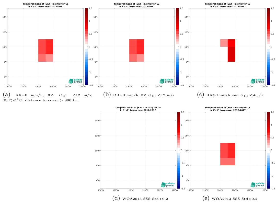
Figure 14: Temporal mean gridded over spatial boxes of size 1^\circ \times 1^\circ of \Delta SSS (SMOS SSS L3 v2 - 9-Days (BEC) - Saildrone (SPURS 2)) for 5 different subdatasets corresponding to:RR=0 mm/h, 3 < U_{10} < 12 m/s, SST > 5^\circ\text{C} , distance to coast > 800 km (a), RR=0 mm/h, 3 < U_{10} < 12 m/s (b), RR > 1 mm/h and U_{10} < 4 m/s (c), WOA2013 SSS Std < 0.2 (d), WOA2013 SSS Std > 0.2 (e).
