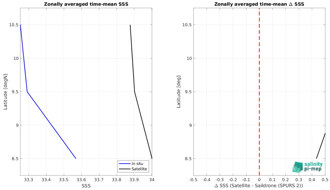
Figure 9: Left panel: Zonal mean SSS from SMOS SSS L3 v2 - 9-Days (BEC) satellite product (black) and from Sairdrone (SPURS 2) (blue). Right panel: Zonal mean of \Delta SSS (Satellite - Sairdrone (SPURS 2)) for all the collected Pi-MEP match-up pairs estimated over the full satellite product period.
