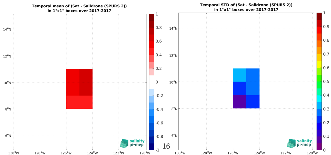
(e) MEAN( \Delta SSS) (Satellite - Saildrone (SPURS 2))
