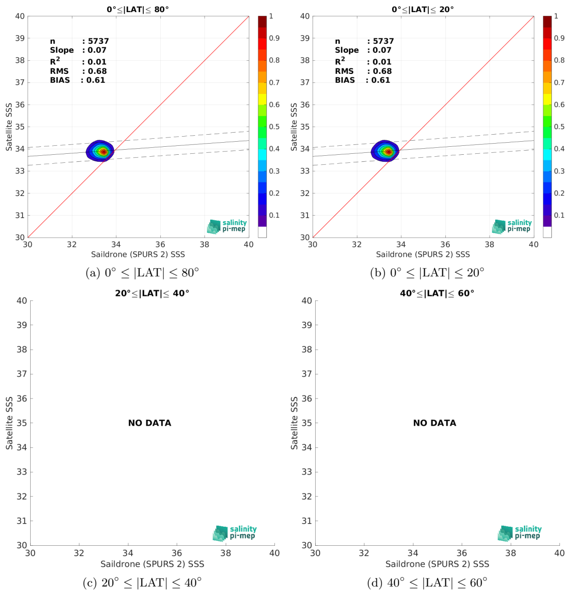
Figure 10: Contour maps of the concentration of SMOS SSS L3 v2 - 9-Days (BEC) SSS (y-axis) versus Saildrone (SPURS 2) SSS (x-axis) at match-up pairs for different latitude bands. For each plot, the red line shows x=y . The black thin and dashed lines indicate a linear fit through the data cloud and the \pm 95\% confidence levels, respectively. The number match-up pairs n , the slope and R^2 coefficient of the linear fit, the root mean square (RMS) and the mean bias between satellite and in situ data are indicated for each latitude band in each plots.
