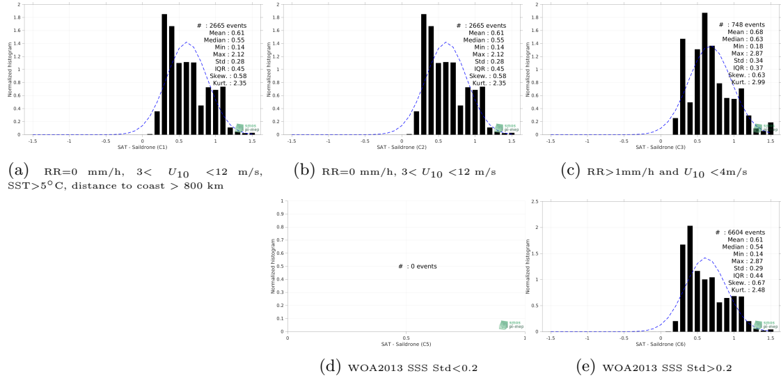
Figure 13: Normalized histogram of \Delta SSS (SMOS SSS L3 v2 - 9-Days (BEC) - Saildrone) for 5 different subdatasets corresponding to: RR=0 mm/h, 3 < U_{10} < 12 m/s, SST>5°C, distance to coast > 800 km (a), RR=0 mm/h, 3 < U_{10} < 12 m/s (b), RR>1mm/h and U_{10} < 4 m/s (c), WOA2013 SSS Std<0.2 (d), WOA2013 SSS Std>0.2 (e).
