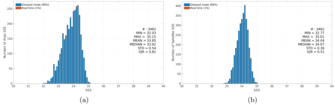
Figure 3: Histograms of SSS from Argo (a) and SMOS SSS L3 v2 - 9-Days (BEC) (b) considering all match-up pairs per bins of 0.1 over the SPURS 2 Pi-MEP region and for the full satellite product period.
