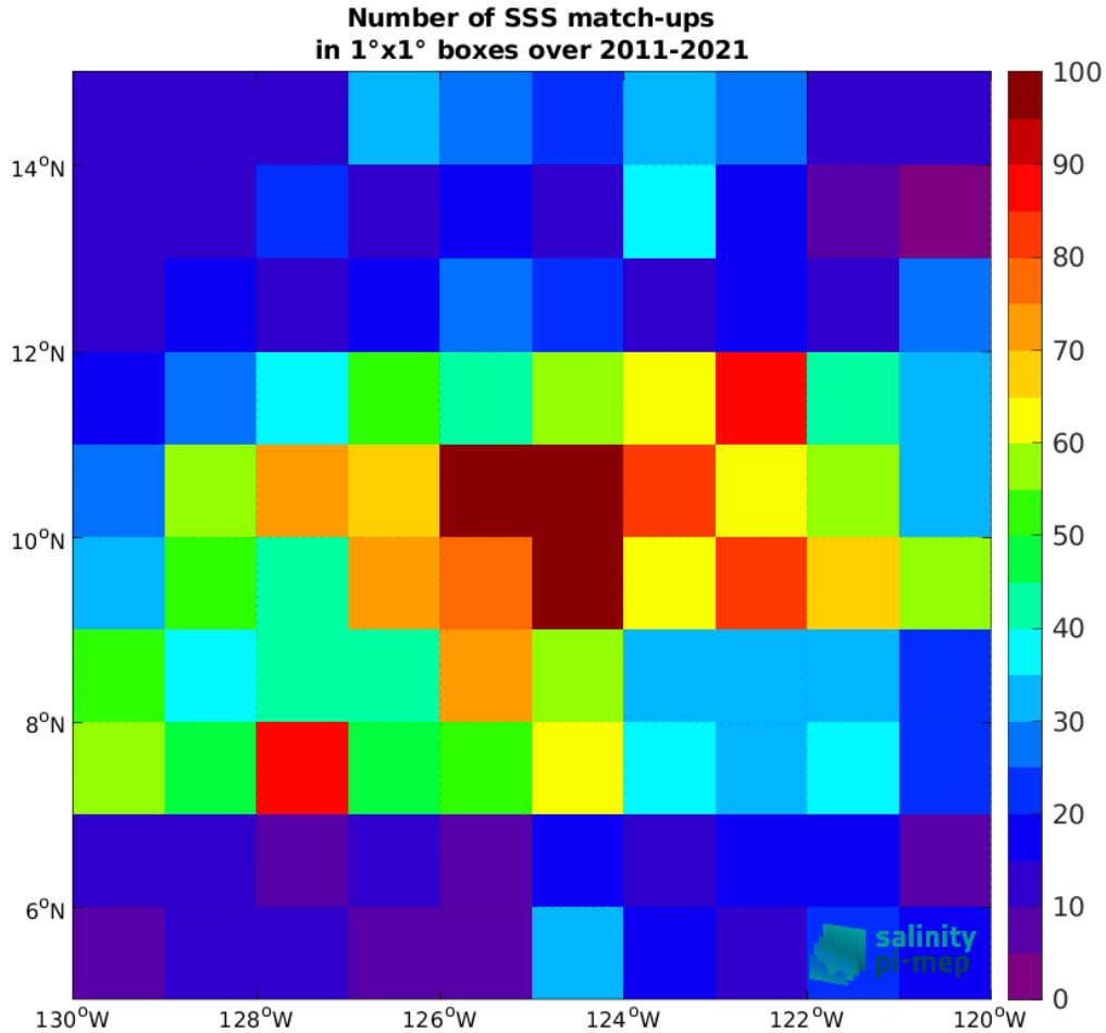
Figure 5: Number of SSS match-ups between Argo SSS and the SMOS SSS L3 v2 - 9-Days (BEC) SSS product for the SPURS 2 Pi-MEP region over 1^\circ \times 1^\circ boxes and for the full satellite product period.
