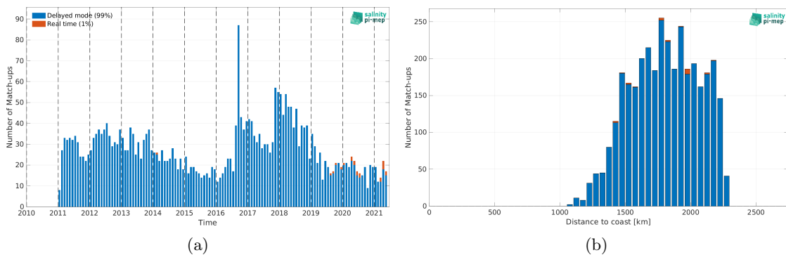
Figure 2: Number of match-ups between Argo and SMOS SSS L3 v2 - 9-Days (BEC) SSS as a function of time (a) and as function of the distance to coast (b) over the SPURS 2 Pi-MEP region and for the full satellite product period.
