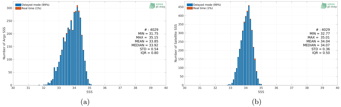
Figure 2: Histograms of SSS from Argo (a) and SMOS SSS L3 v2 - 9-Days (BEC) (b) considering all match-up pairs per bins of 0.1 over the SPURS 2 Pi-MEP region and for the full satellite product period.
