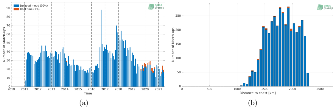
Figure 1: Number of match-ups between Argo and SMOS SSS L3 v2 - 9-Days (BEC) SSS as a function of time (a) and as function of the distance to coast (b) over the SPURS 2 Pi-MEP region and for the full satellite product period.
