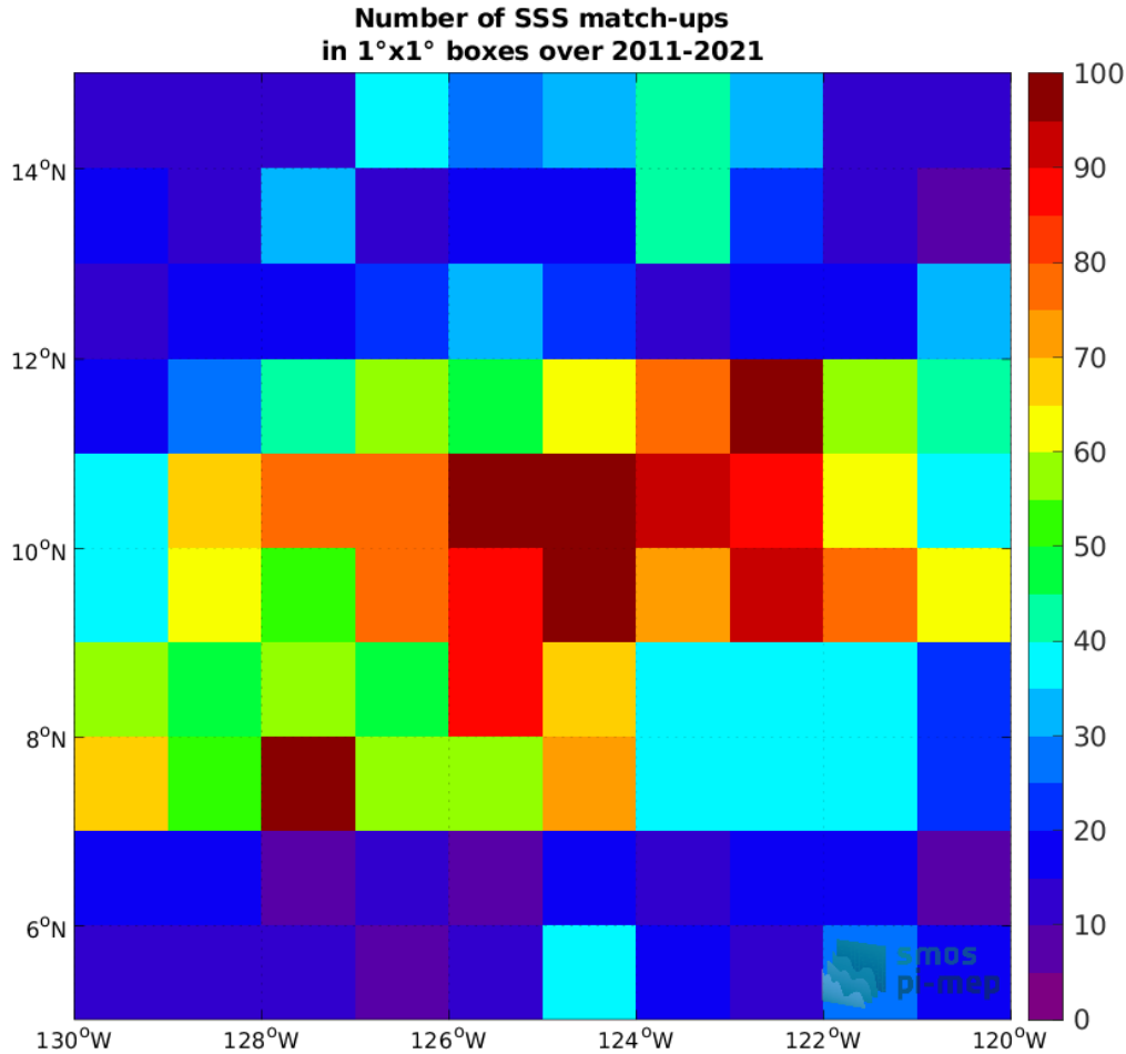
Figure 4: Number of SSS match-ups between Argo SSS and the SMOS SSS L3 v2 - 9-Days (BEC) SSS product for the SPURS 2 Pi-MEP region over 1^\circ \times 1^\circ boxes and for the full satellite product period.
