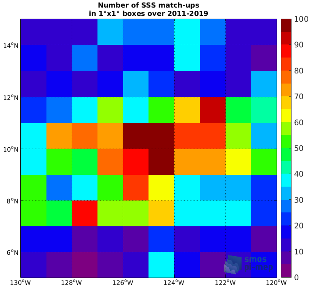
Figure 4: Number of SSS match-ups between Argo SSS and the SMOS SSS L3 v2 - 9-Days (BEC) SSS product for the SPURS 2 Pi-MEP region over 1°x1° boxes and for the full satellite product period.
