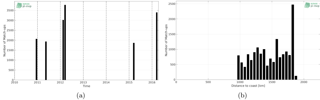
Figure 1: Number of match-ups between TSG-SAMOS and SMOS-L3-BEC-OA-V1-9DAYS-0.25DEG SSS as a function of time (a) and as function of the distance to coast (b) over the SPURS 2 Pi-MEP region and for the full satellite product period.
