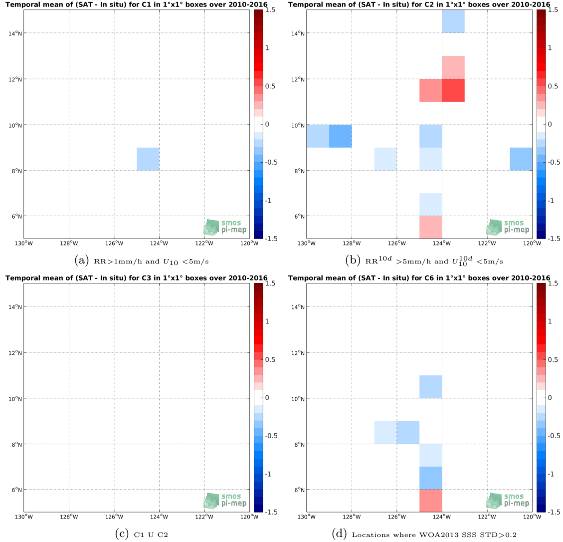
Figure 12: Temporal mean gridded over spatial boxes of size 1^\circ \times 1^\circ of \Delta SSS (SMOS-L3-BEC-OA-V1-9DAYS-0.25DEG - TSG-SAMOS) for 4 different subdatasets corresponding to: RR > 1\text{mm/h} and U_{10} < 5\text{m/s} (a), RR^{10d} > 5\text{mm/h} and U_{10}^{10d} < 5\text{m/s} (b), C1 U C2 (c), Locations where WOA2013 SSS STD > 0.2 (d).
