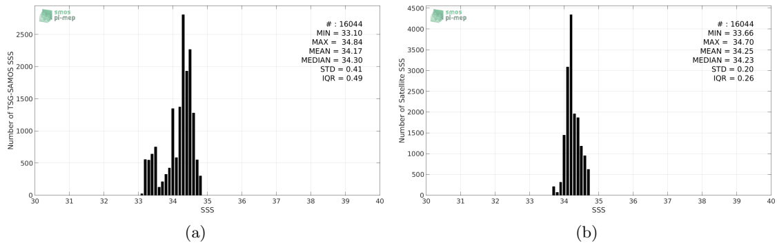
Figure 2: Histograms of SSS from TSG-SAMOS (a) and SMOS-L3-BEC-OA-V1-9DAYS-0.25DEG (b) considering all match-up pairs per bins of 0.1 over the SPURS 2 Pi-MEP region and for the full satellite product period.
