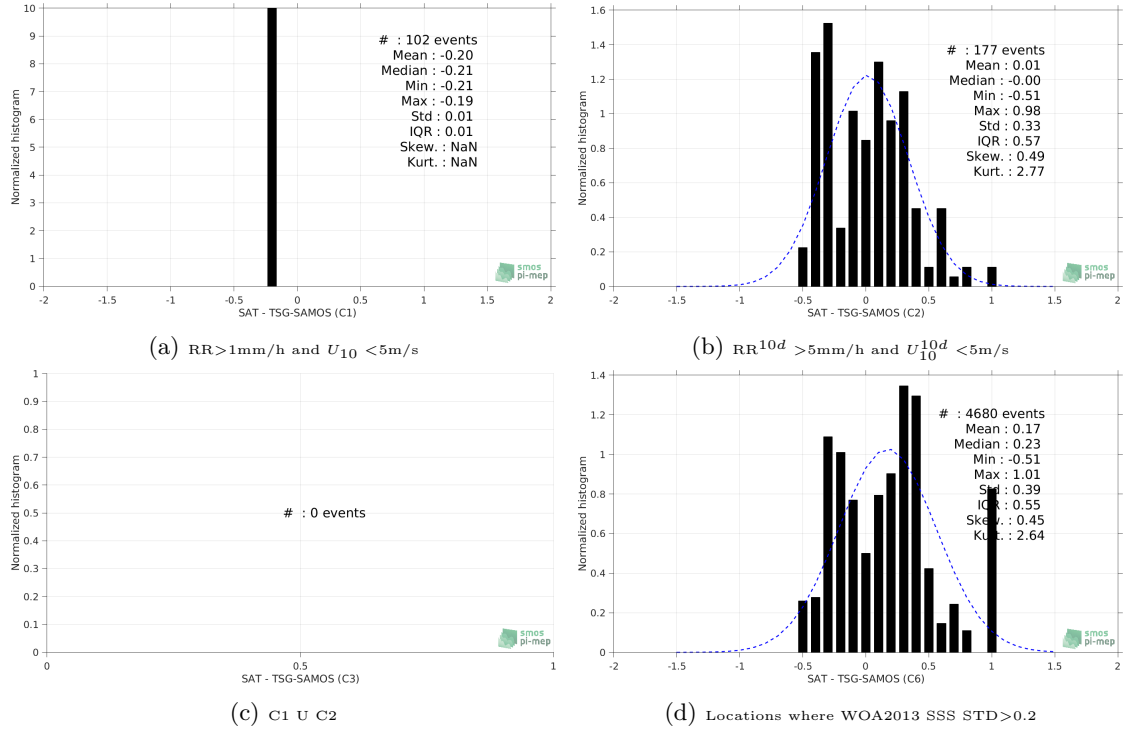
Figure 13: Normalized histogram of \Delta SSS (SMOS-L3-BEC-OA-V1-9DAYS-0.25DEG - TSG-SAMOS) for 6 different subdatasets corresponding to: RR > 1mm/h and U_{10} < 5 m/s (a), RR^{10d} > 5 mm/h and U_{10}^{10d} < 5 m/s (b), C1 U C2 (c), Locations where WOA2013 SSS STD > 0.2 (d).
