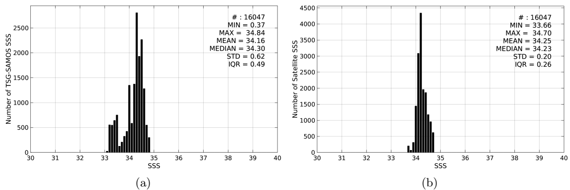
Figure 2: Histograms of SSS from TSG-SAMOS (a) and SMOS-L3-BEC-OA-V1-9DAYS-0.25DEG (b) considering all match-up pairs per bins of 0.1 over the SPURS 2 Pi-MEP region and for the full satellite product period.
