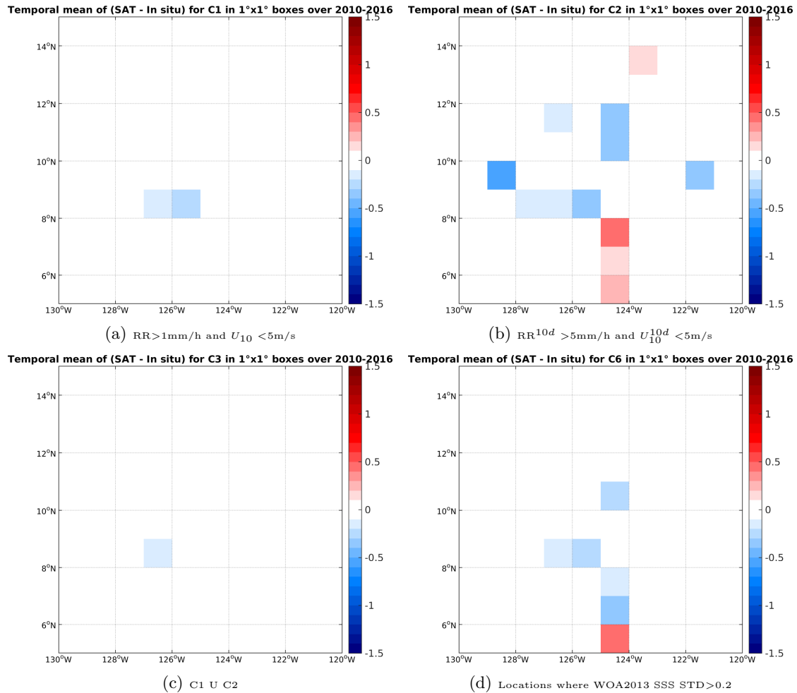
Figure 12: Temporal mean gridded over spatial boxes of size 1^\circ \times 1^\circ of \Delta SSS (SMOS-L3-BEC-OA-V1-9DAYS-0.25DEG - TSG-SAMOS) for 4 different subdatasets corresponding to: RR > 1mm/h and U_{10} < 5 m/s (a), RR^{10d} > 5 mm/h and U_{10}^{10d} < 5 m/s (b), C1 U C2 (c), Locations where WOA2013 SSS STD > 0.2 (d).
