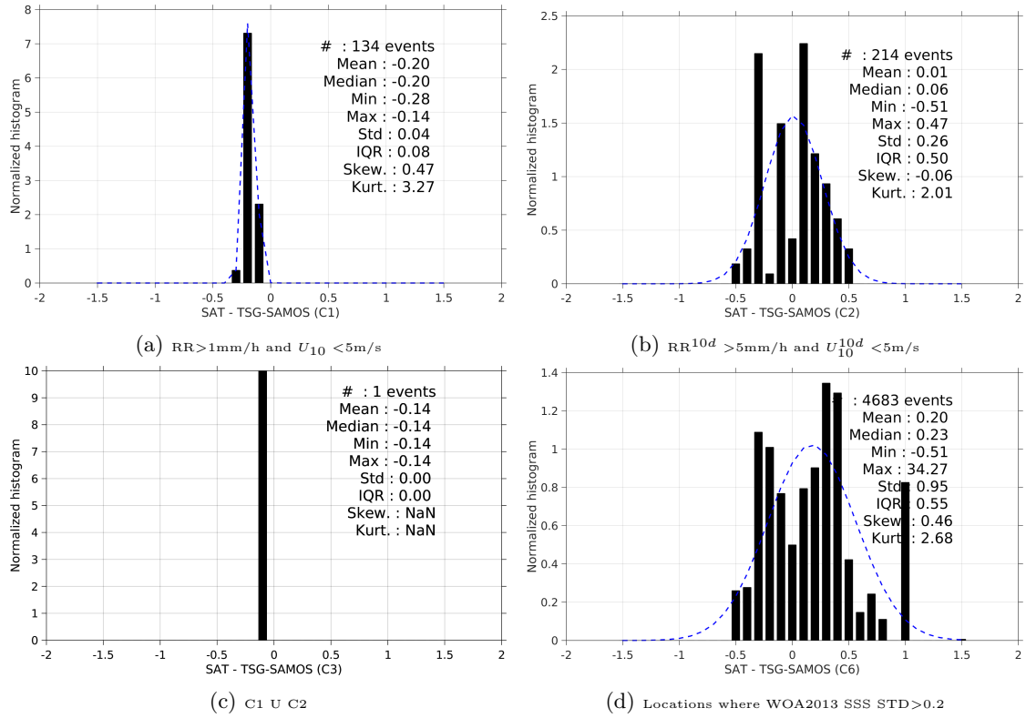
Figure 13: Normalized histogram of \Delta\text{SSS} (SMOS-L3-BEC-OA-V1-9DAYS-0.25DEG - TSG-SAMOS) for 6 different subdatasets corresponding to: RR > 1mm/h and U_{10} < 5\text{m/s} (a), RR^{10d} > 5\text{mm/h} and U_{10}^{10d} < 5\text{m/s} (b), C1 U C2 (c), Locations where WOA2013 SSS STD > 0.2 (d).
