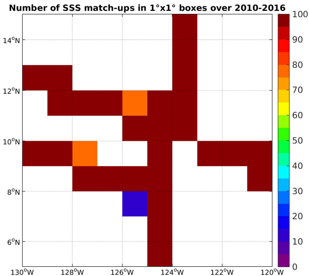
Figure 4: Number of SSS match-ups between TSG-SAMOS SSS and the SMOS-L3-BEC-OA-V1-9DAYS-0.25DEG SSS product for the SPURS 2 Pi-MEP region over 1°x1° boxes and for the full satellite product period.
