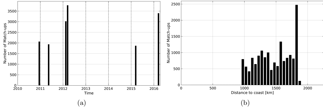
Figure 1: Number of match-ups between TSG-SAMOS and SMOS-L3-BEC-OA-V1-9DAYS-0.25DEG SSS as a function of time (a) and as function of the distance to coast (b) over the SPURS 2 Pi-MEP region and for the full satellite product period.
