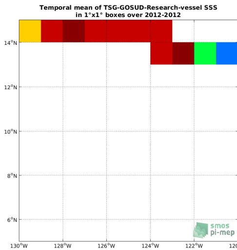
(c) MEAN(TSG-GOSUD-Research-vessel SSS)
