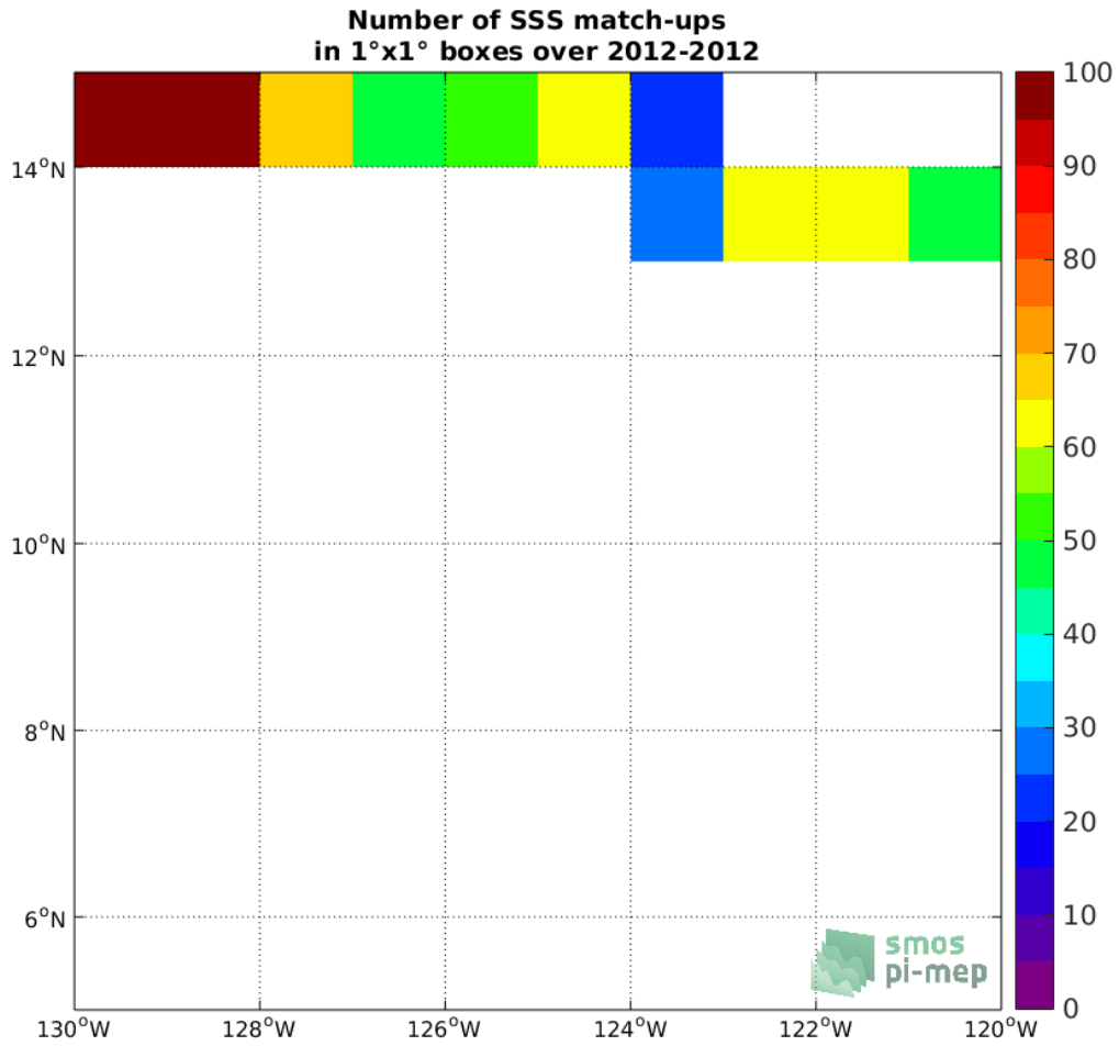
Figure 4: Number of SSS match-ups between TSG-GOSUD-Research-vessel SSS and the SMOS-L3-BEC-OA-V1-9DAYS-0.25DEG SSS product for the SPURS 2 Pi-MEP region over 1°x1° boxes and for the full satellite product period.
