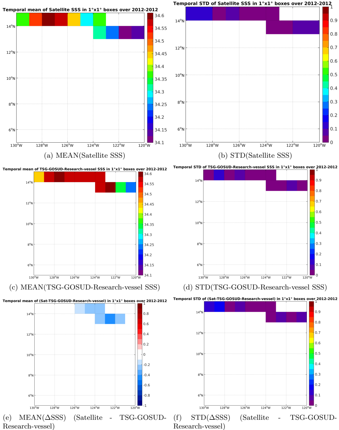
Figure 6: Temporal mean (left) and STD (right) of SSS from SMOS-L3-BEC-OA-V1-9DAYS-0.25DEG (top), TSG-GOSUD-Research-vessel (middle), and of \Delta SSS (Satellite - TSG-GOSUD-Research-vessel). Only match-up pairs are used to generate these maps.
