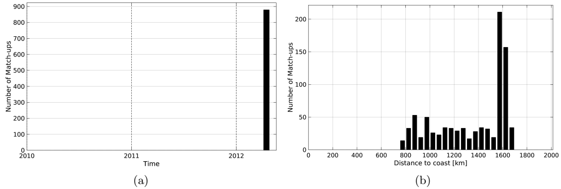
Figure 1: Number of match-ups between TSG-GOSUD-Research-vessel and SMOS-L3-BEC-OA-V1-9DAYS-0.25DEG SSS as a function of time (a) and as function of the distance to coast (b) over the SPURS 2 Pi-MEP region and for the full satellite product period.
