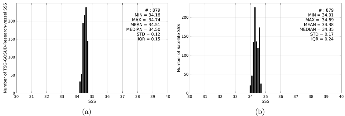
Figure 2: Histograms of SSS from TSG-GOSUD-Research-vessel (a) and SMOS-L3-BEC-OA-V1-9DAYS-0.25DEG (b) considering all match-up pairs per bins of 0.1 over the SPURS 2 Pi-MEP region and for the full satellite product period.
