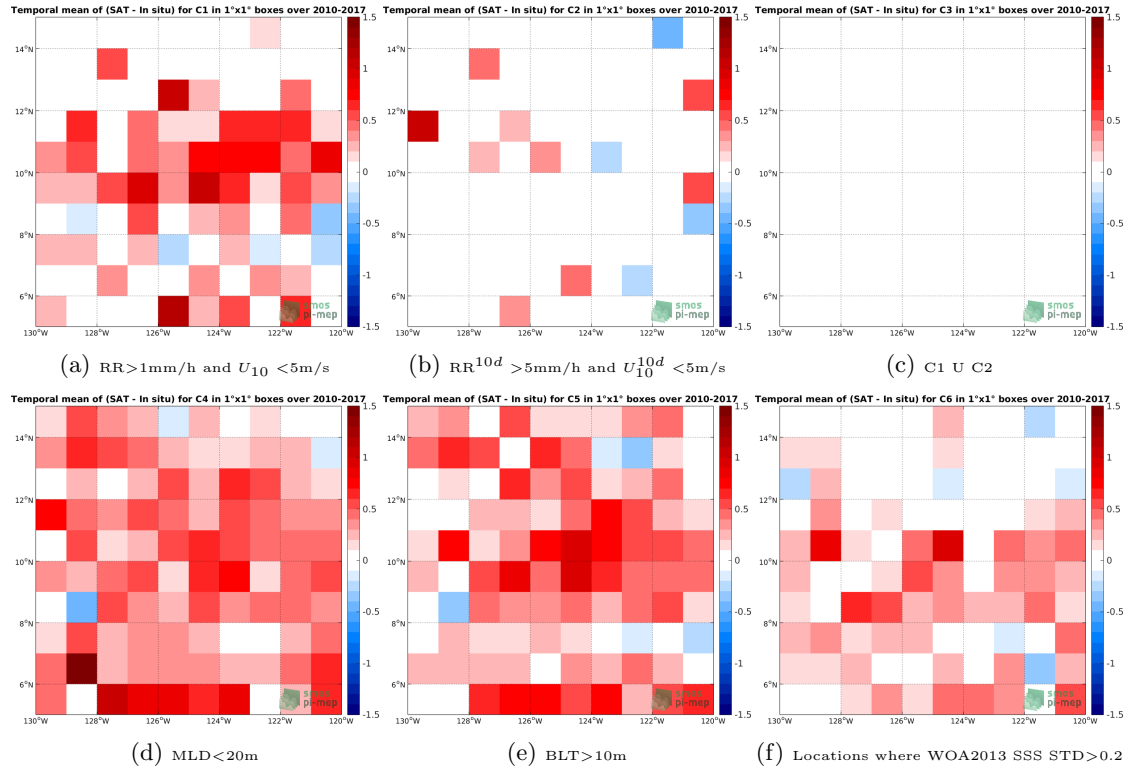
Figure 12: Temporal mean gridded over spatial boxes of size 1^\circ \times 1^\circ of \Delta\text{SSS} (SMOS-L3-BEC-OA-V1-9DAYS-0.25DEG - Argo) for 6 different subdatasets corresponding to:RR >1\text{mm/h} and U_{10} < 5\text{m/s} (a), RR^{10d} > 5\text{mm/h} and U_{10}^{10d} < 5\text{m/s} (b), C1 U C2 (c),MLD <20\text{m} (d),BLT >10\text{m} (e),Locations where WOA2013 SSS STD >0.2 (f).
