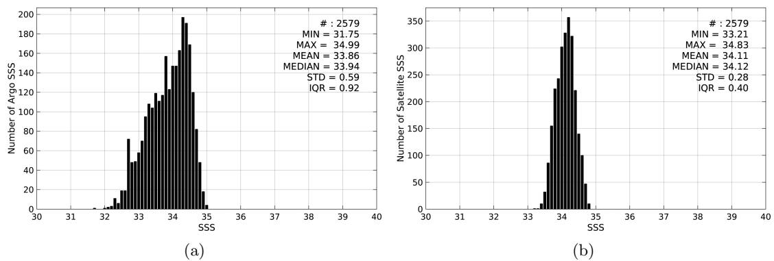
Figure 2: Histograms of SSS from Argo (a) and SMOS-L3-BEC-OA-V1-9DAYS-0.25DEG (b) considering all match-up pairs per bins of 0.1 over the SPURS 2 Pi-MEP region and for the full satellite product period.
