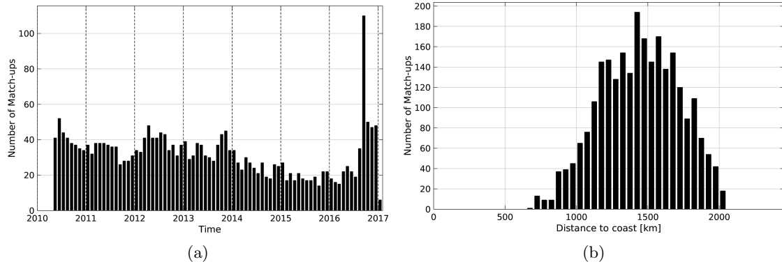
Figure 1: Number of match-ups between Argo and SMOS-L3-BEC-OA-V1-9DAYS-0.25DEG SSS as a function of time (a) and as function of the distance to coast (b) over the SPURS 2 Pi-MEP region and for the full satellite product period.
