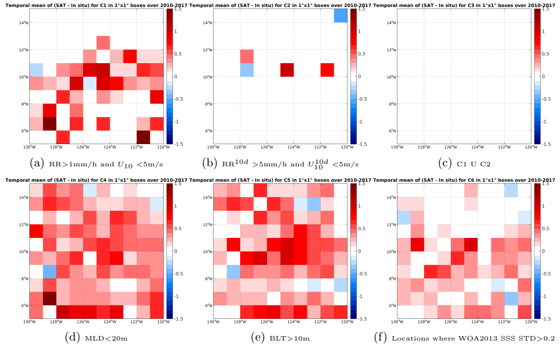
Figure 12: Temporal mean gridded over spatial boxes of size 1^\circ \times 1^\circ of \Delta SSS (SMOS-L3-BEC-OA-V1-9DAYS-0.25DEG - Argo) for 6 different subdatasets corresponding to: RR > 1mm/h and U_{10} < 5\text{m/s} (a), RR^{10d} > 5\text{mm/h} and U_{10^d} < 5\text{m/s} (b), C1 U C2 (c), MLD < 20m (d), BLT > 10m (e), Locations where WOA2013 SSS STD > 0.2 (f).
