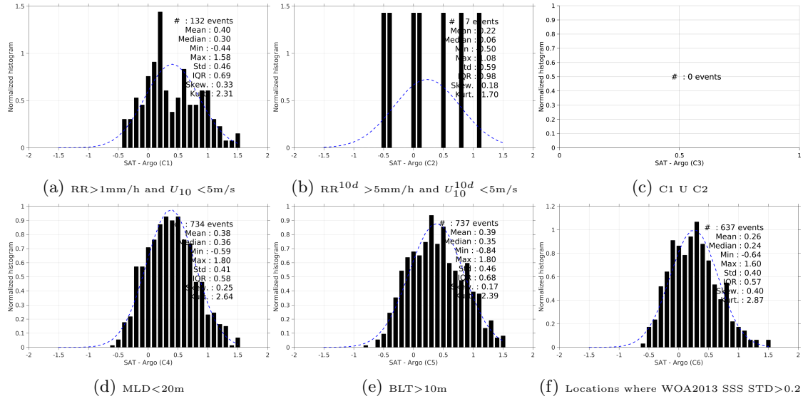
Figure 13: Normalized histogram of \Delta SSS (SMOS-L3-BEC-OA-V1-9DAYS-0.25DEG - Argo) for 6 different subdatasets corresponding to: RR>1mm/h and U_{10} < 5 m/s (a), RR 10d >5mm/h and U_{10}^{10d} < 5 m/s (b), C1 U C2 (c),MLD<20m (d),BLT>10m (e),Locations where WOA2013 SSS STD>0.2 (f).
