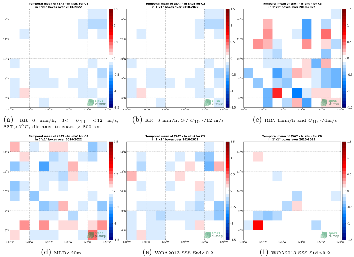
Figure 12: Temporal mean gridded over spatial boxes of size 1^\circ \times 1^\circ of \Delta SSS (SMOS SSS L2-AVERAGED v700 (ESA) - Argo) for 6 different subdatasets corresponding to:RR=0 mm/h, 3 < U_{10} < 12 m/s, SST >5^\circ C, distance to coast > 800 km (a), RR=0 mm/h, 3 < U_{10} < 12 m/s (b), RR >1 mm/h and U_{10} < 4 m/s (c),MLD <20 m (d),WOA2013 SSS Std <0.2 (e),WOA2013 SSS Std >0.2 (f).
