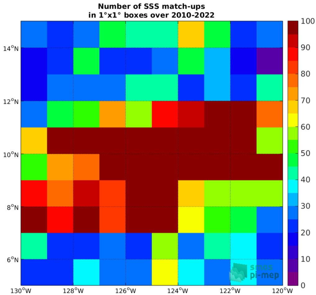
Figure 4: Number of SSS match-ups between Argo SSS and the SMOS SSS L2-AVERAGED v700 (ESA) SSS product for the SPURS 2 Pi-MEP region over 1°x1° boxes and for the full satellite product period.
