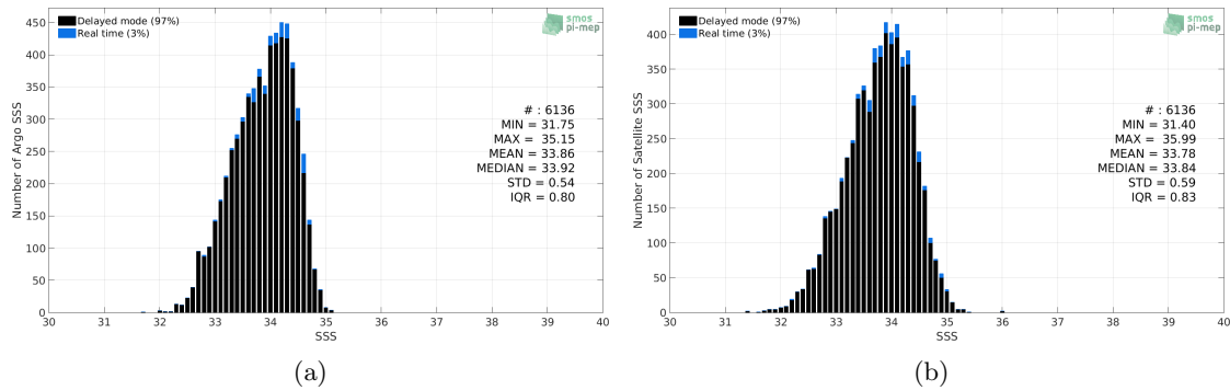
Figure 2: Histograms of SSS from Argo (a) and SMOS SSS L2-AVERAGED v700 (ESA) (b) considering all match-up pairs per bins of 0.1 over the SPURS 2 Pi-MEP region and for the full satellite product period.
