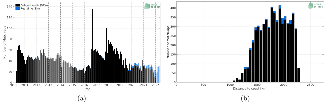
Figure 1: Number of match-ups between Argo and SMOS SSS L2-AVERAGED v700 (ESA) SSS as a function of time (a) and as function of the distance to coast (b) over the SPURS 2 Pi-MEP region and for the full satellite product period.
