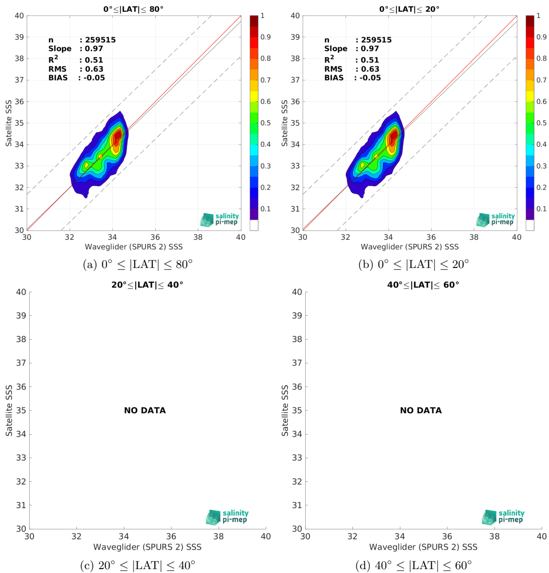
Figure 9: Contour maps of the concentration of SMOS SSS L2 v700 (ESA) SSS (y-axis) versus Waveglider (SPURS 2) SSS (x-axis) at match-up pairs for different latitude bands. For each plot, the red line shows x=y . The black thin and dashed lines indicate a linear fit through the data cloud and the \pm 95\% confidence levels, respectively. The number match-up pairs n , the slope and R^2 coefficient of the linear fit, the root mean square (RMS) and the mean bias between satellite and in situ data are indicated for each latitude band in each plots.
