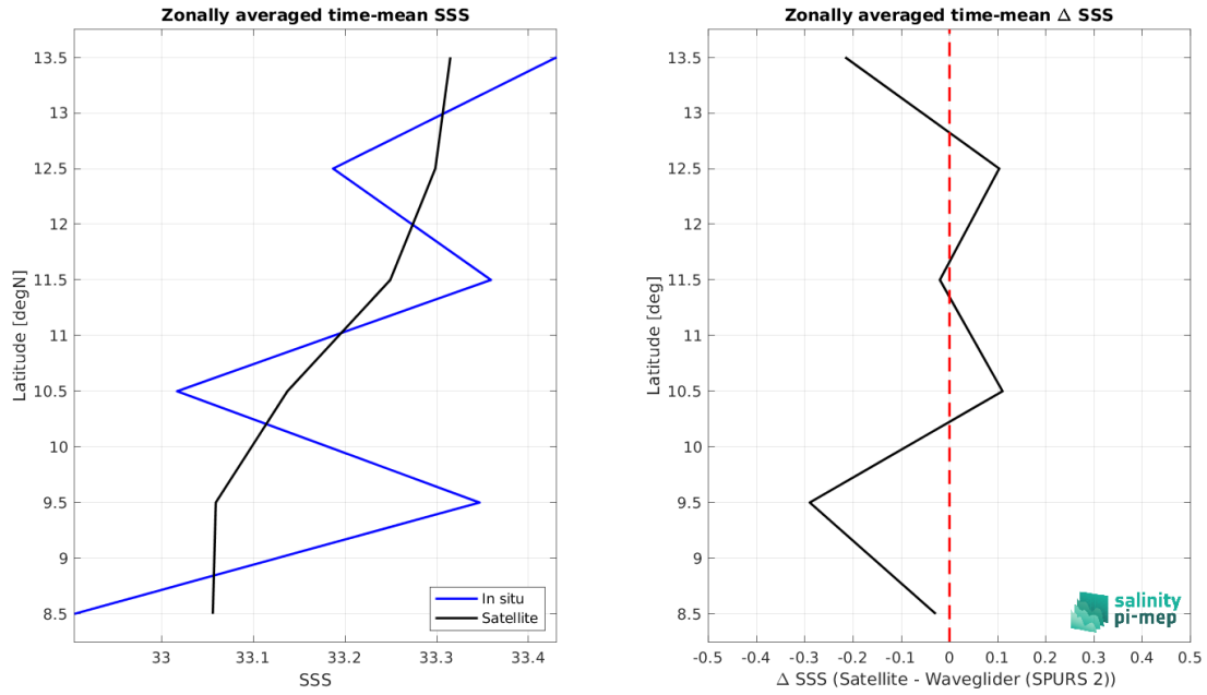
Figure 8: Left panel: Zonal mean SSS from SMOS SSS L2 v700 (ESA) satellite product (black) and from Waveglider (SPURS 2) (blue). Right panel: Zonal mean of \Delta SSS (Satellite - Waveglider (SPURS 2)) for all the collected Pi-MEP match-up pairs estimated over the full satellite product period.
