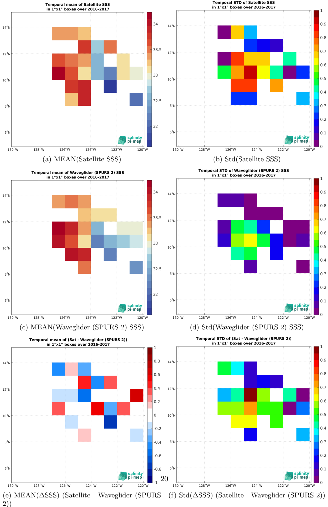
Figure 6: Temporal mean (left) and Std (right) of SSS from SMOS SSS L2 v700 (ESA) (top), Waveglider (SPURS 2) (middle), and of \Delta SSS (Satellite - Waveglider (SPURS 2)). Only match-up pairs are used to generate these maps.
