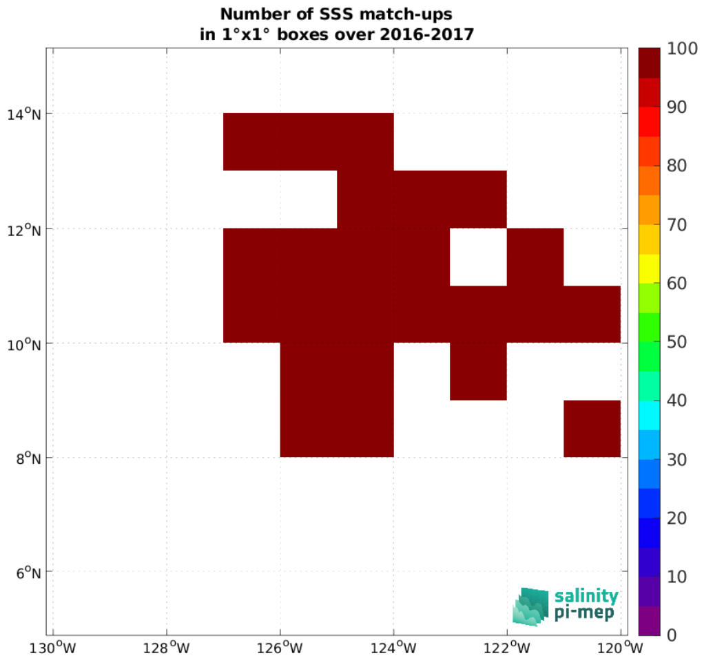
Figure 4: Number of SSS match-ups between Waveglider (SPURS 2) SSS and the SMOS SSS L2 v700 (ESA) SSS product for the SPURS 2 Pi-MEP region over 1^\circ \times 1^\circ boxes and for the full satellite product period.
