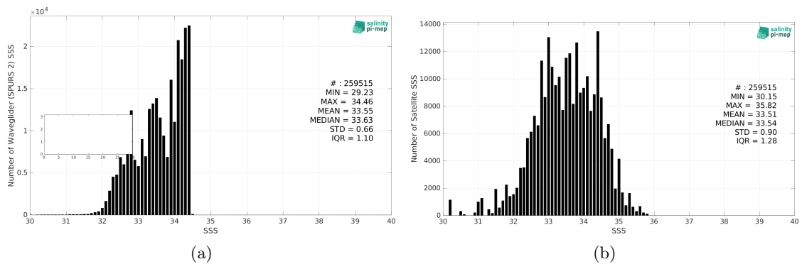
Figure 2: Histograms of SSS from Waveglider (SPURS 2) (a) and SMOS SSS L2 v700 (ESA) (b) considering all match-up pairs per bins of 0.1 over the SPURS 2 Pi-MEP region and for the full satellite product period.
