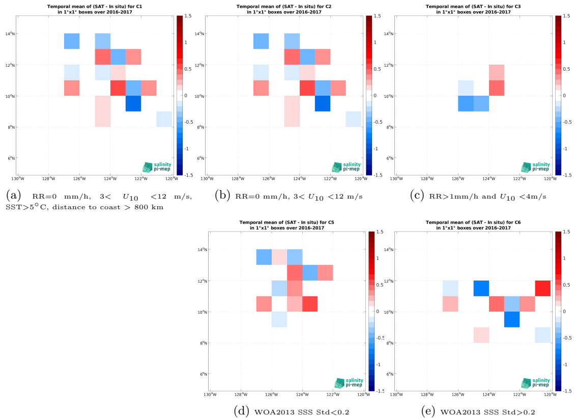
Figure 12: Temporal mean gridded over spatial boxes of size 1^\circ \times 1^\circ of \Delta SSS (SMOS SSS L2 v700 (ESA) - Waveglider (SPURS 2)) for 5 different subdatasets corresponding to:RR=0 mm/h, 3 < U_{10} < 12 m/s, SST >5^\circ\text{C} , distance to coast > 800 km (a), RR=0 mm/h, 3 < U_{10} < 12 m/s (b), RR >1 mm/h and U_{10} < 4 m/s (c), WOA2013 SSS Std <0.2 (d), WOA2013 SSS Std >0.2 (e).
