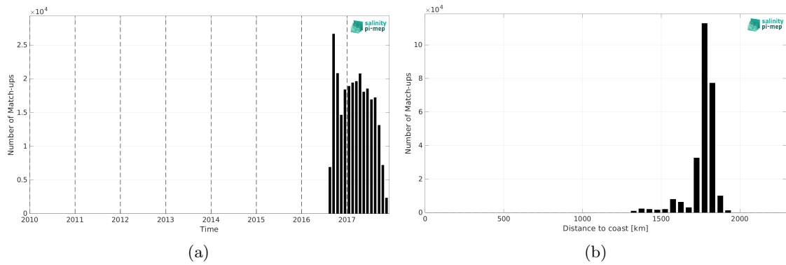
Figure 1: Number of match-ups between Waveglider (SPURS 2) and SMOS SSS L2 v700 (ESA) SSS as a function of time (a) and as function of the distance to coast (b) over the SPURS 2 Pi-MEP region and for the full satellite product period.
