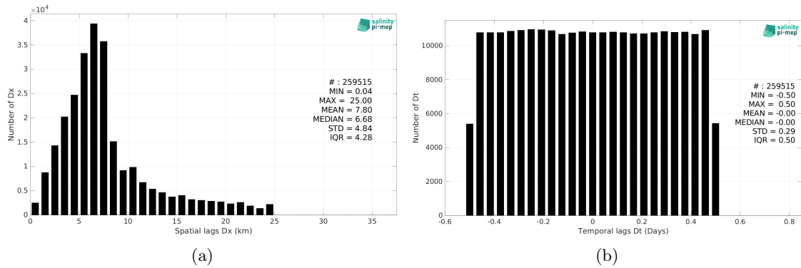
Figure 5: Histograms of the spatial (a) and temporal (b) lags between the location/time of the Waveglider (SPURS 2) measurement and the date of the corresponding SMOS SSS L2 v700 (ESA) SSS pixel.
