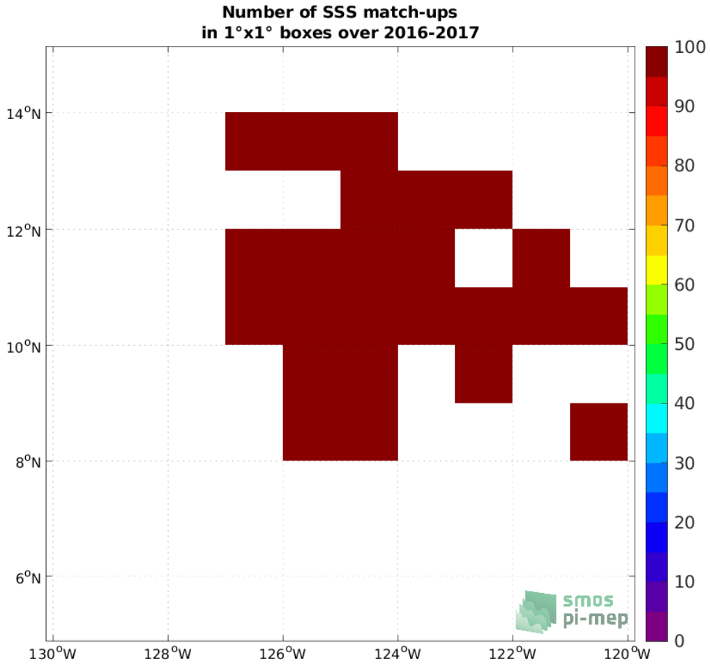
Figure 4: Number of SSS match-ups between Waveglider (SPURS 2) SSS and the SMOS SSS L2 v700 (ESA) SSS product for the SPURS 2 Pi-MEP region over 1°x1° boxes and for the full satellite product period.
