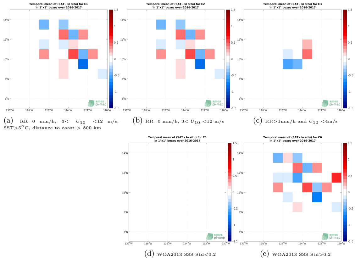
Figure 12: Temporal mean gridded over spatial boxes of size 1^\circ \times 1^\circ of \Delta SSS (SMOS SSS L2 v700 (ESA) - Waveglider) for 5 different subdatasets corresponding to:RR=0 mm/h, 3 < U_{10} < 12 m/s, SST>5°C, distance to coast > 800 km (a), RR=0 mm/h, 3 < U_{10} < 12 m/s (b), RR>1mm/h and U_{10} < 4 m/s (c), WOA2013 SSS Std<0.2 (d), WOA2013 SSS Std>0.2 (e).
