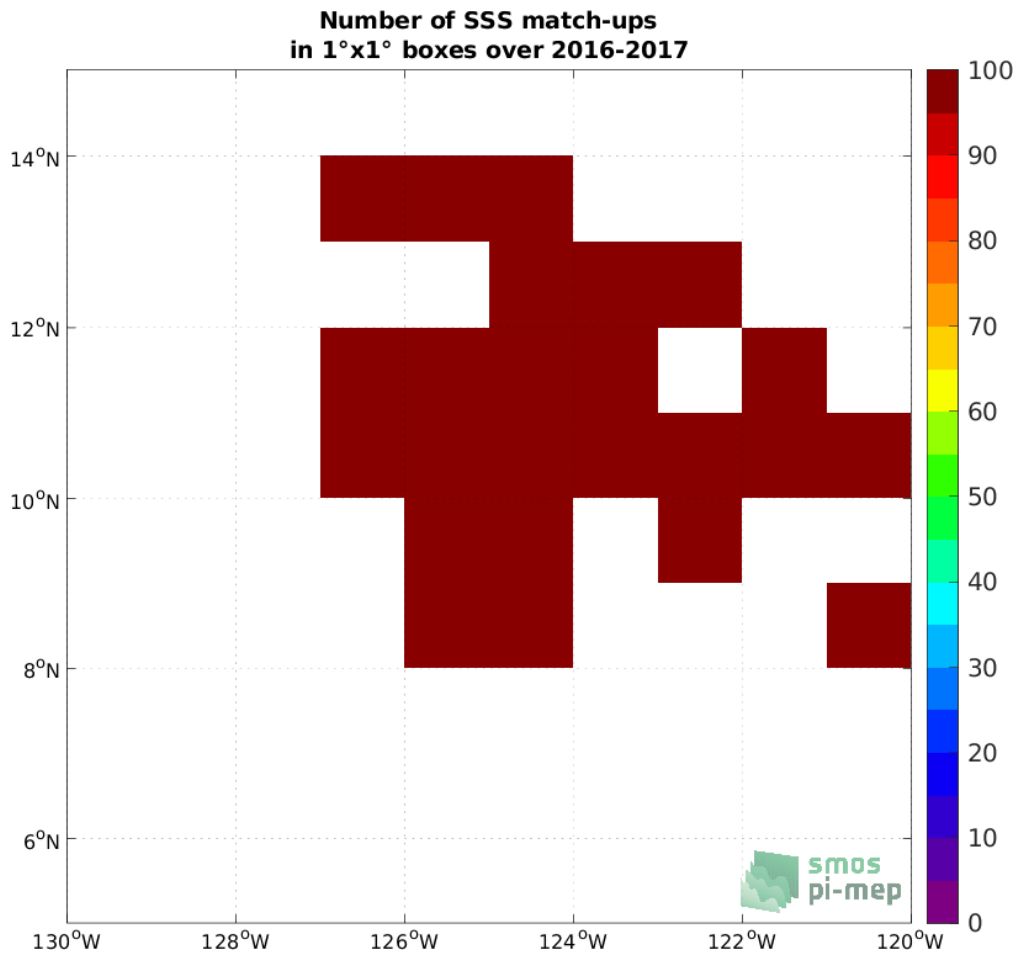
Figure 4: Number of SSS match-ups between Waveglider SSS and the SMOS SSS L2 v700 (ESA) SSS product for the SPURS 2 Pi-MEP region over 1°x1° boxes and for the full satellite product period.
