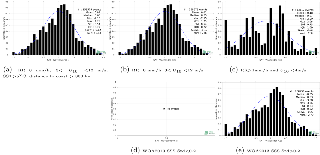
Figure 13: Normalized histogram of \Delta\text{SSS} (SMOS SSS L2 v700 (ESA) - Waveglider) for 5 different subdatasets corresponding to: RR=0 mm/h, 3 < U_{10} < 12 m/s, SST >5^{\circ}\text{C} , distance to coast > 800 km (a), RR=0 mm/h, 3 < U_{10} < 12 m/s (b), RR >1 mm/h and U_{10} < 4 m/s (c), WOA2013 SSS Std <0.2 (d), WOA2013 SSS Std >0.2 (e).
