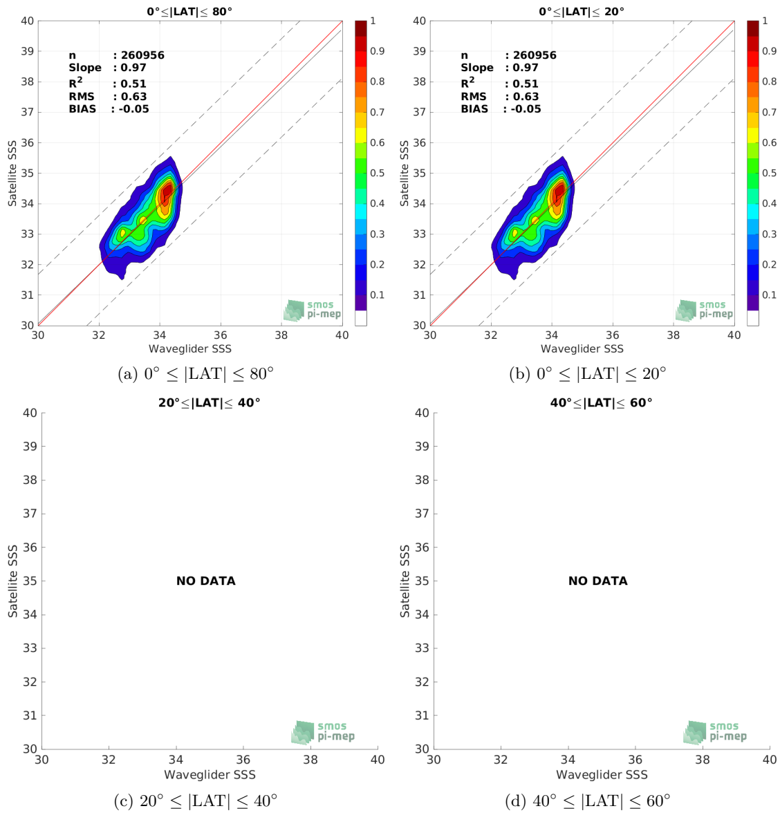
Figure 9: Contour maps of the concentration of SMOS SSS L2 v700 (ESA) SSS (y-axis) versus Waveglider SSS (x-axis) at match-up pairs for different latitude bands. For each plot, the red line shows x=y . The black thin and dashed lines indicate a linear fit through the data cloud and the \pm 95\% confidence levels, respectively. The number match-up pairs n , the slope and R^2 coefficient of the linear fit, the root mean square (RMS) and the mean bias between satellite and in situ data are indicated for each latitude band in each plots.
