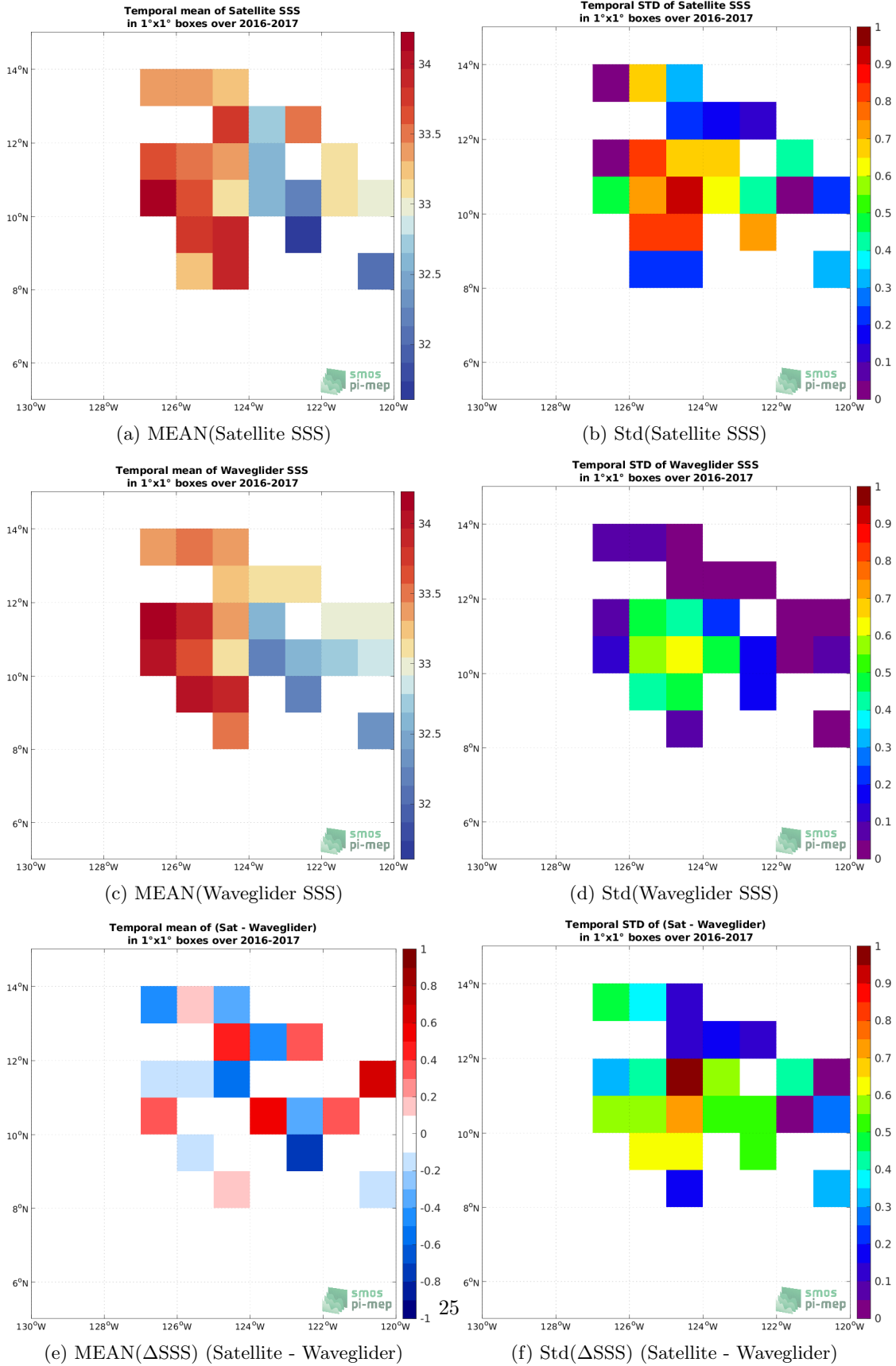
Figure 6: Temporal mean (left) and Std (right) of SSS from SMOS SSS L2 v700 (ESA) (top), Waveglider (middle), and of \Delta SSS (Satellite - Waveglider). Only match-up pairs are used to generate these maps.
