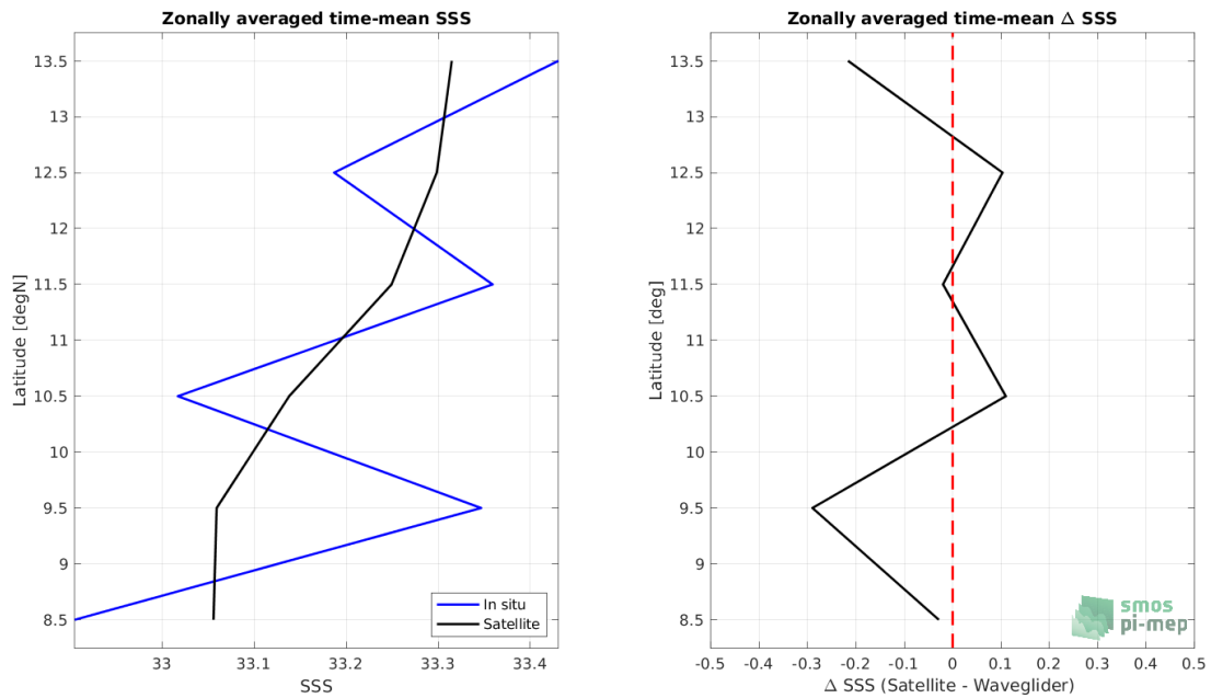
Figure 8: Left panel: Zonal mean SSS from SMOS SSS L2 v700 (ESA) satellite product (black) and from Waveglider (blue). Right panel: Zonal mean of \Delta SSS (Satellite - Waveglider) for all the collected Pi-MEP match-up pairs estimated over the full satellite product period.
