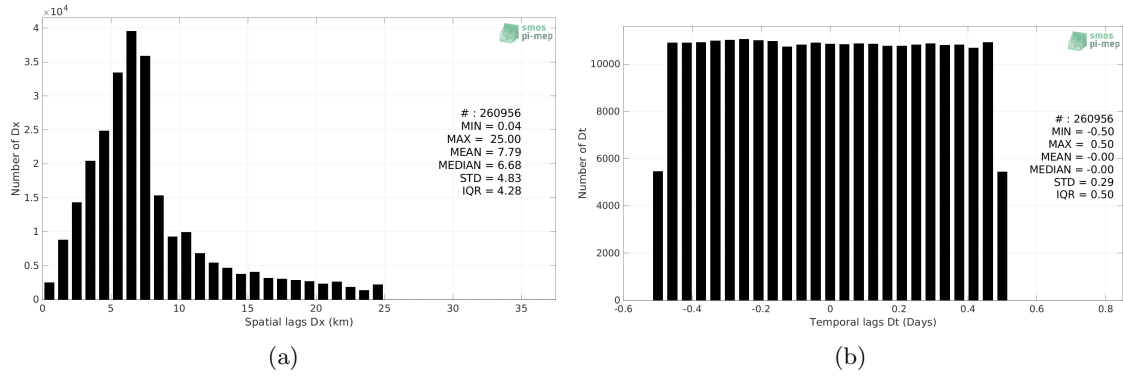
Figure 5: Histograms of the spatial (a) and temporal (b) lags between the location/time of the Waveglider measurement and the date of the corresponding SMOS SSS L2 v700 (ESA) SSS pixel.
