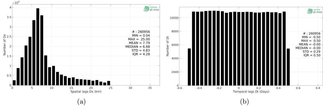
Figure 4: Histograms of the spatial (a) and temporal (b) lags between the location/time of the Waveglider measurement and the date of the corresponding SMOS SSS L2 v700 (ESA) SSS pixel.
