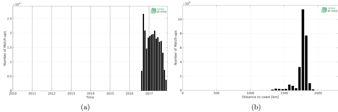
Figure 1: Number of match-ups between Waveglider and SMOS SSS L2 v700 (ESA) SSS as a function of time (a) and as function of the distance to coast (b) over the SPURS 2 Pi-MEP region and for the full satellite product period.
