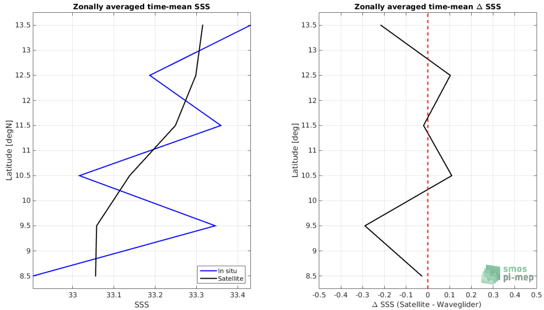
Figure 7: Left panel: Zonal mean SSS from SMOS SSS L2 v700 (ESA) satellite product (black) and from Waveglider (blue). Right panel: Zonal mean of \Delta SSS (Satellite - Waveglider) for all the collected Pi-MEP match-up pairs estimated over the full satellite product period.
