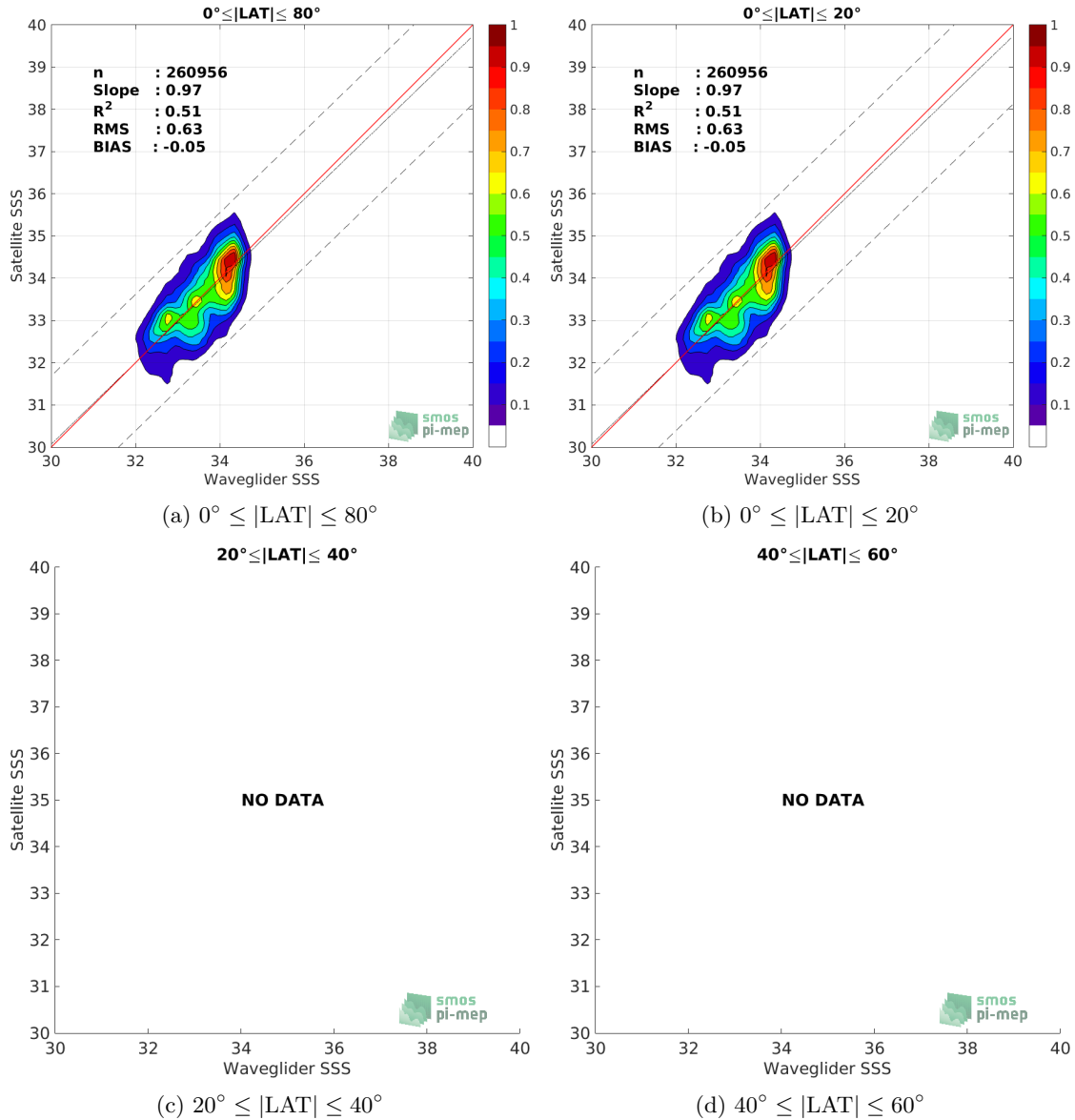
Figure 8: Contour maps of the concentration of SMOS SSS L2 v700 (ESA) SSS (y-axis) versus Waveglider SSS (x-axis) at match-up pairs for different latitude bands. For each plot, the red line shows x=y . The black thin and dashed lines indicate a linear fit through the data cloud and the \pm 95\% confidence levels, respectively. The number match-up pairs n , the slope and R^2 coefficient of the linear fit, the root mean square (RMS) and the mean bias between satellite and in situ data are indicated for each latitude band in each plots.
