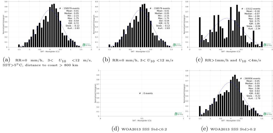
Figure 12: Normalized histogram of \Delta SSS (SMOS SSS L2 v700 (ESA) - Waveglider) for 5 different subdatasets corresponding to: RR=0 mm/h, 3 < U_{10} < 12 m/s, SST > 5°C, distance to coast > 800 km (a), RR=0 mm/h, 3 < U_{10} < 12 m/s (b), RR > 1mm/h and U_{10} < 4 m/s (c), WOA2013 SSS Std < 0.2 (d), WOA2013 SSS Std > 0.2 (e).
