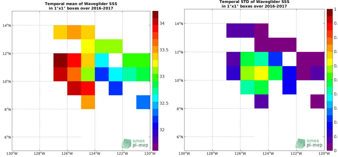
(c) MEAN(Waveglider SSS)
