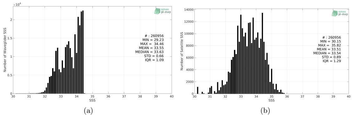
Figure 2: Histograms of SSS from Waveglider (a) and SMOS SSS L2 v700 (ESA) (b) considering all match-up pairs per bins of 0.1 over the SPURS 2 Pi-MEP region and for the full satellite product period.
