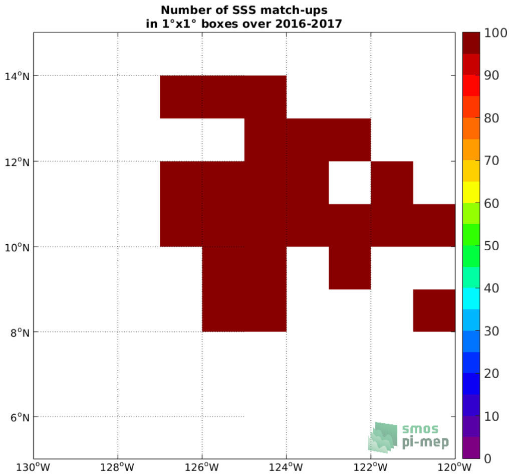
Figure 3: Number of SSS match-ups between Waveglider SSS and the SMOS SSS L2 v700 (ESA) SSS product for the SPURS 2 Pi-MEP region over 1°×1° boxes and for the full satellite product period.
