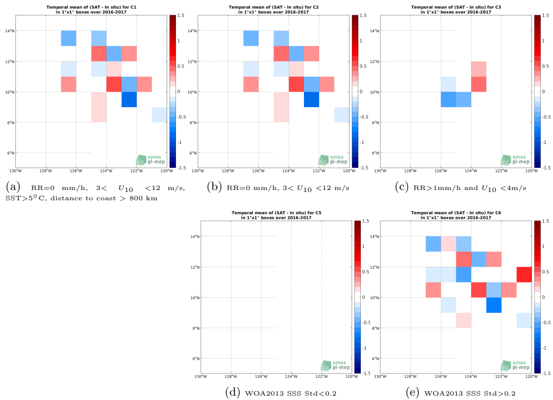
Figure 11: Temporal mean gridded over spatial boxes of size 1^\circ \times 1^\circ of \Delta SSS (SMOS SSS L2 v700 (ESA) - Waveglider) for 5 different subdatasets corresponding to:RR=0 mm/h, 3 < U_{10} < 12 m/s, SST >5^\circ\text{C} , distance to coast > 800 km (a), RR=0 mm/h, 3 < U_{10} < 12 m/s (b), RR >1 mm/h and U_{10} < 4 m/s (c), WOA2013 SSS Std <0.2 (d), WOA2013 SSS Std >0.2 (e).
