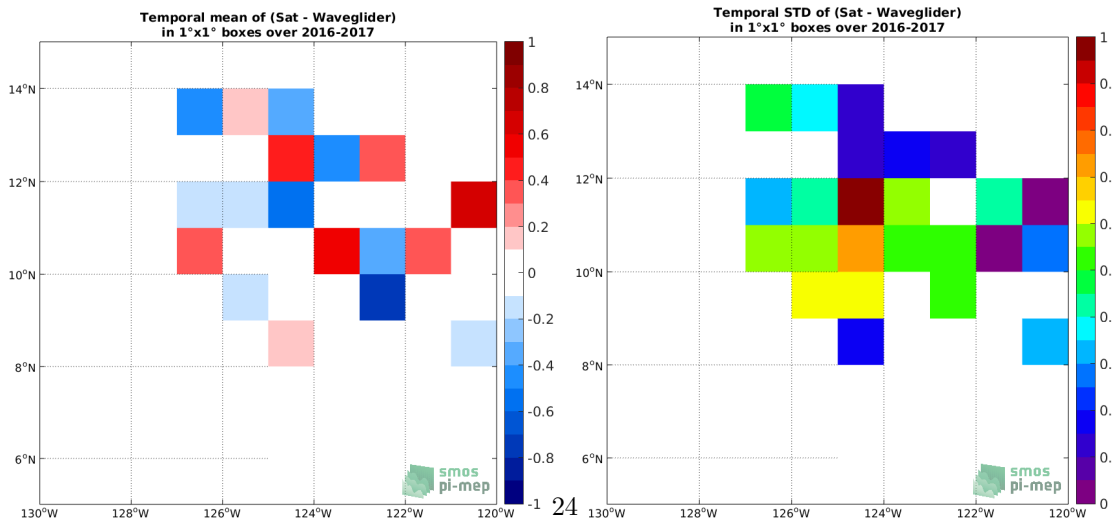
(e) MEAN( \Delta SSS) (Satellite - Waveglider)
