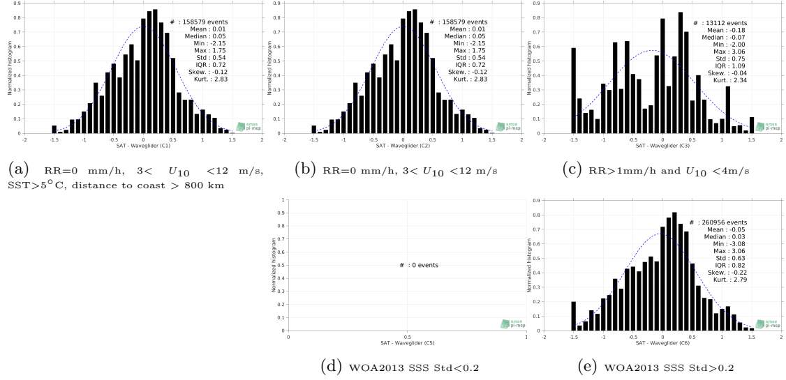
Figure 12: Normalized histogram of \Delta SSS (SMOS SSS L2 v700 (ESA) - Waveglider) for 5 different subdatasets corresponding to: RR=0 mm/h, 3 < U_{10} < 12 m/s, SST > 5°C, distance to coast > 800 km (a), RR=0 mm/h, 3 < U_{10} < 12 m/s (b), RR > 1mm/h and U_{10} < 4 m/s (c), WOA2013 SSS Std < 0.2 (d), WOA2013 SSS Std > 0.2 (e).
