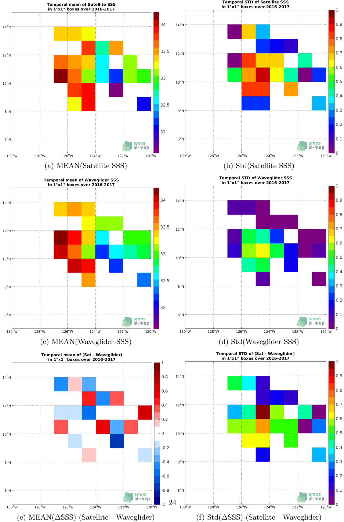
Figure 5: Temporal mean (left) and Std (right) of SSS from SMOS SSS L2 v700 (ESA) (top), Waveglider (middle), and of \Delta SSS (Satellite - Waveglider). Only match-up pairs are used to generate these maps.
