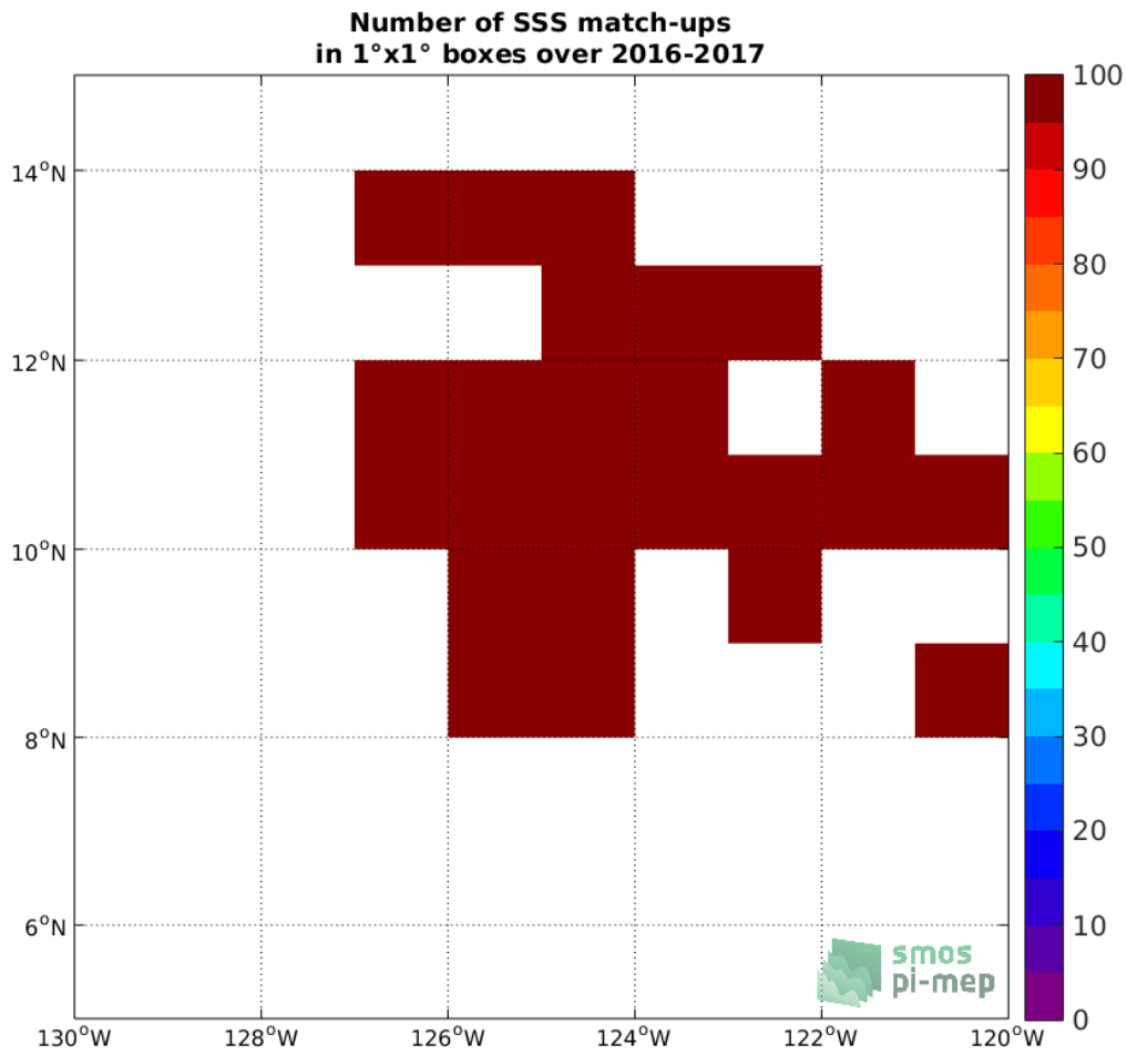
Figure 3: Number of SSS match-ups between Waveglider SSS and the SMOS SSS L2 v700 (ESA) SSS product for the SPURS 2 Pi-MEP region over 1°x1° boxes and for the full satellite product period.
