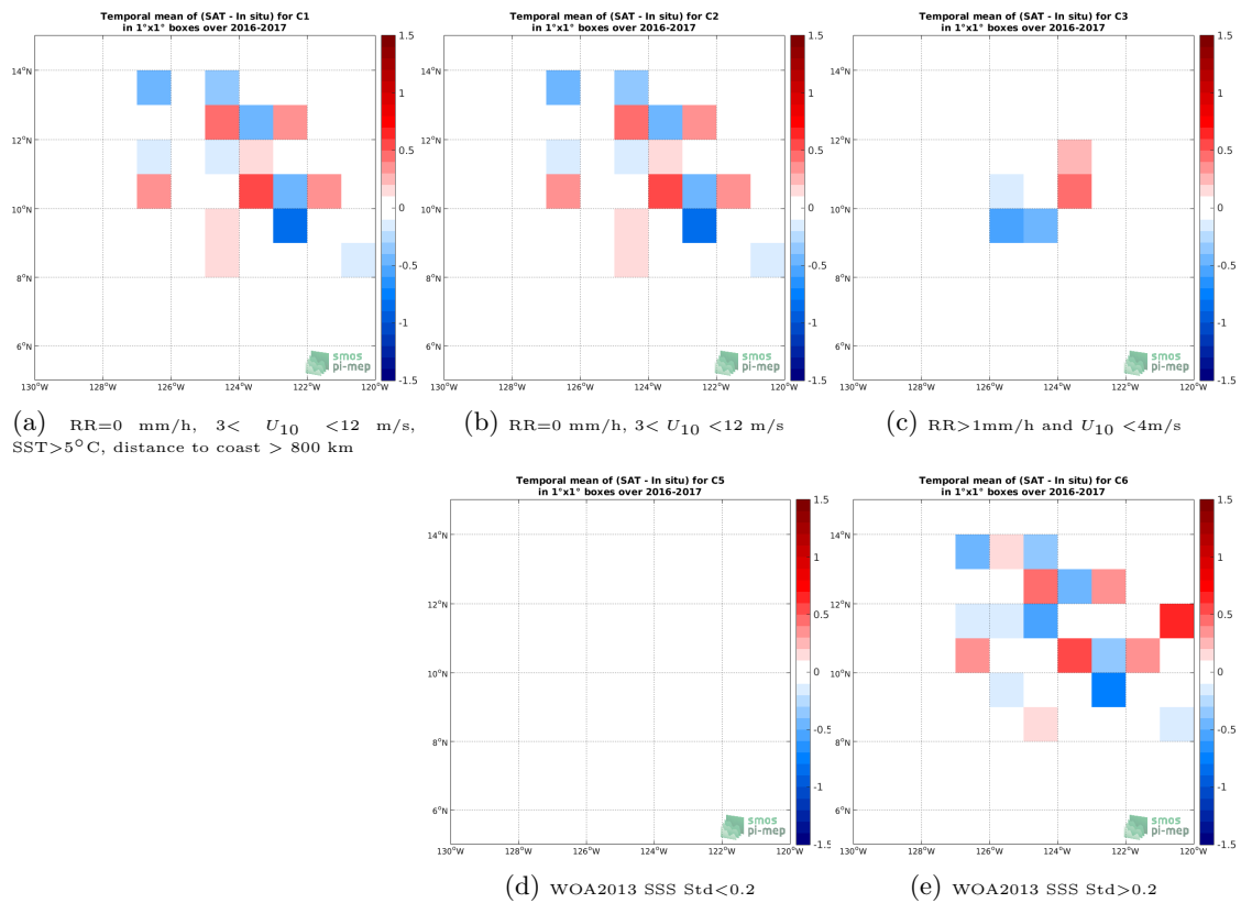
Figure 11: Temporal mean gridded over spatial boxes of size 1^\circ \times 1^\circ of \Delta\text{SSS} (SMOS SSS L2 v700 (ESA) - Waveglider) for 5 different subdatasets corresponding to: RR=0 mm/h, 3 < U_{10} < 12 m/s, SST > 5^\circ\text{C} , distance to coast > 800 km (a), RR=0 mm/h, 3 < U_{10} < 12 m/s (b), RR > 1\text{mm/h} and U_{10} < 4\text{m/s} (c), WOA2013 SSS Std < 0.2 (d), WOA2013 SSS Std > 0.2 (e).
