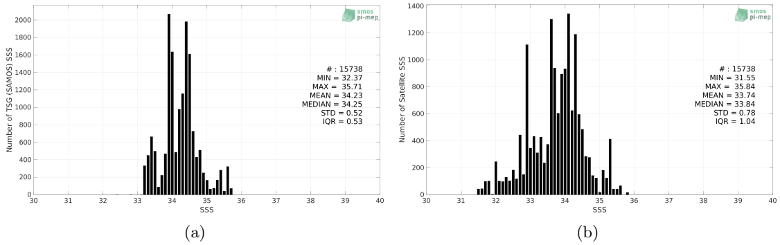
Figure 2: Histograms of SSS from TSG (SAMOS) (a) and SMOS SSS L2 v700 (ESA) (b) considering all match-up pairs per bins of 0.1 over the SPURS 2 Pi-MEP region and for the full satellite product period.
