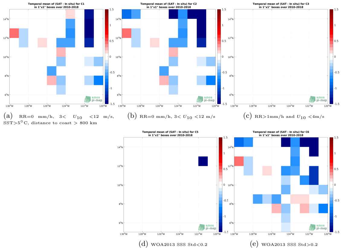
Figure 12: Temporal mean gridded over spatial boxes of size 1^\circ \times 1^\circ of \Delta SSS (SMOS SSS L2 v700 (ESA) - TSG (SAMOS)) for 5 different subdatasets corresponding to:RR=0 mm/h, 3 < U_{10} < 12 m/s, SST >5^\circ C, distance to coast > 800 km (a), RR=0 mm/h, 3 < U_{10} < 12 m/s (b), RR >1 mm/h and U_{10} < 4 m/s (c), WOA2013 SSS Std <0.2 (d), WOA2013 SSS Std >0.2 (e).
