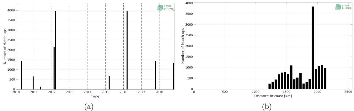
Figure 1: Number of match-ups between TSG (SAMOS) and SMOS SSS L2 v700 (ESA) SSS as a function of time (a) and as function of the distance to coast (b) over the SPURS 2 Pi-MEP region and for the full satellite product period.
