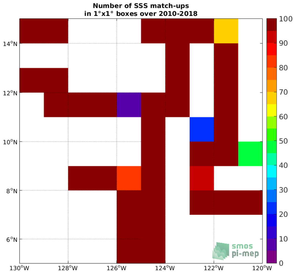
Figure 4: Number of SSS match-ups between TSG (SAMOS) SSS and the SMOS SSS L2 v700 (ESA) SSS product for the SPURS 2 Pi-MEP region over 1°x1° boxes and for the full satellite product period.
