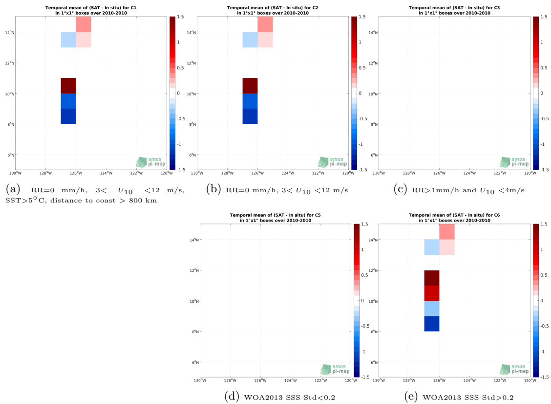
Figure 12: Temporal mean gridded over spatial boxes of size 1^\circ \times 1^\circ of \Delta\text{SSS} (SMOS SSS L2 v700 (ESA) - TSG (GOSUD-Sailing-ship)) for 5 different subdatasets corresponding to:RR=0 mm/h, 3 < U_{10} < 12 m/s, SST>5°C, distance to coast > 800 km (a), RR=0 mm/h, 3 < U_{10} < 12 m/s (b), RR>1mm/h and U_{10} < 4 m/s (c), WOA2013 SSS Std<0.2 (d), WOA2013 SSS Std>0.2 (e).
